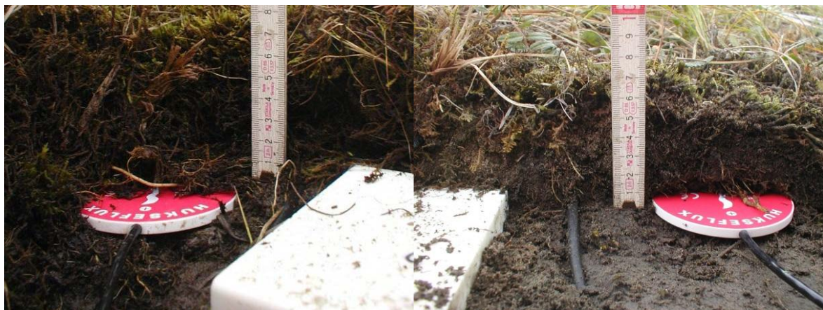
Figure B12. Hukseflux HFP01 ground heat-flux sensors ( left: center, right: rim ), installed on 24 August 2002.
