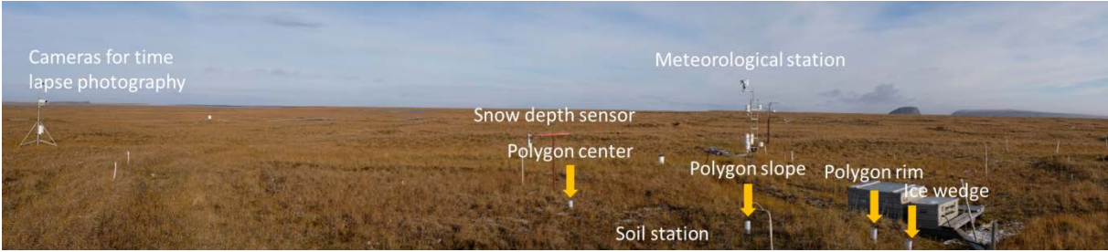
Figure B8. Meteorological station and soil station (consisting of sensors installed along 1D profiles within polygon center, rim, slope, and ice wedge) with cameras for time lapse photography pointing towards both stations for snow and surface observation.
