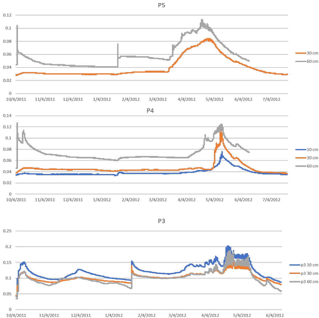
Figure 1. The soil volumetric water content (VWC) data from points 5, 4, and 3, have been graphed here for depths of 10 cm, 30 cm, and 60 cm.
