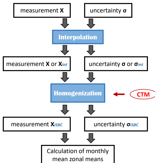
Figure 2. Flow chart describing the different modification and adjustment steps that are applied to the ozone measurements before they are used in the monthly mean zonal mean calculation. Note that 'ISBC' refers to inter-satellite bias correction, which is described in Sect. 3.2.
