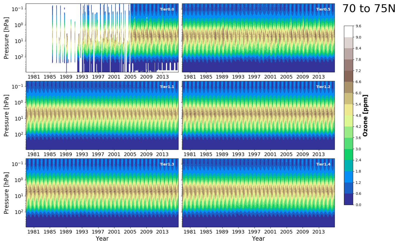
Figure 7. All six Tiers of BSVertOzone for the latitude band 70°N to 75°N (given in ozone mixing ratio on pressure levels).
