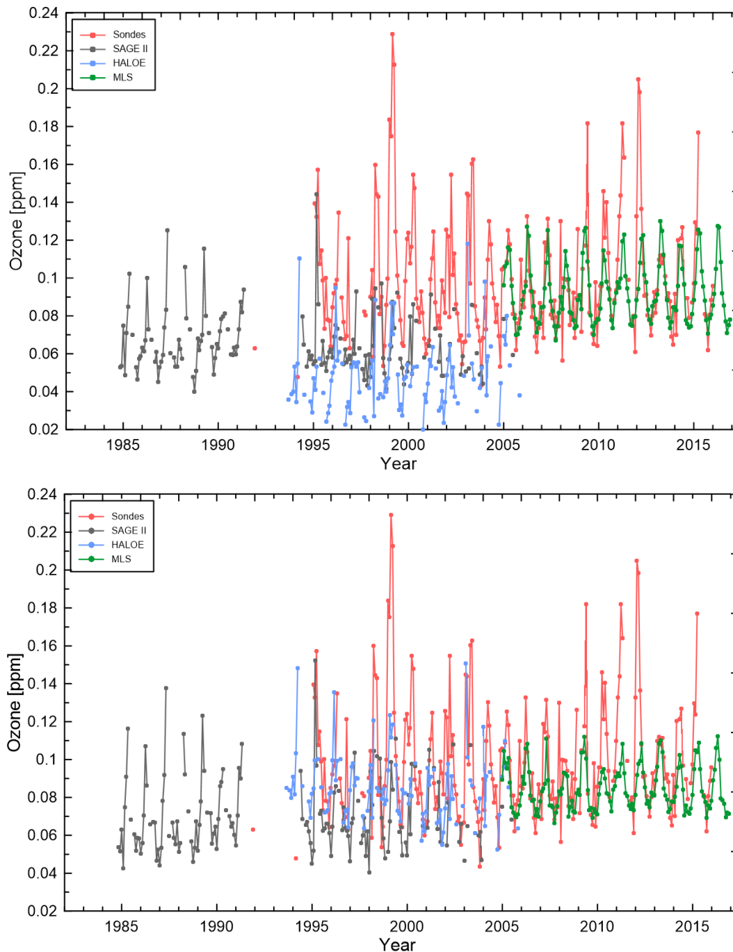
Figure 3. Monthly mean zonal mean ozone mixing ratios from different data sources (color coded as shown in the legends) at 182hPa between 25°N and 30°N. Upper panel: Unadjusted time series and lower panel: adjusted, bias corrected, time series. For more details see text.
