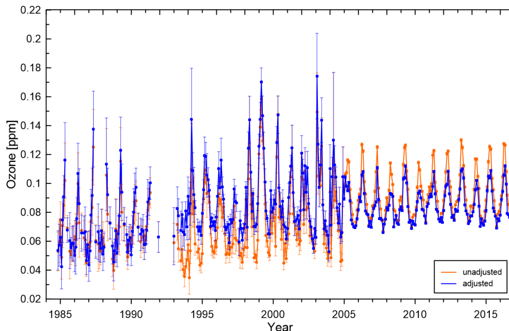
Figure 4. Monthly mean zonal mean ozone mixing ratio at 182hPa between 25°N and 30°N as calculated from all data sources before (orange line) and after (blue line) the homogenization process has been applied to the source data. For more details see text.
