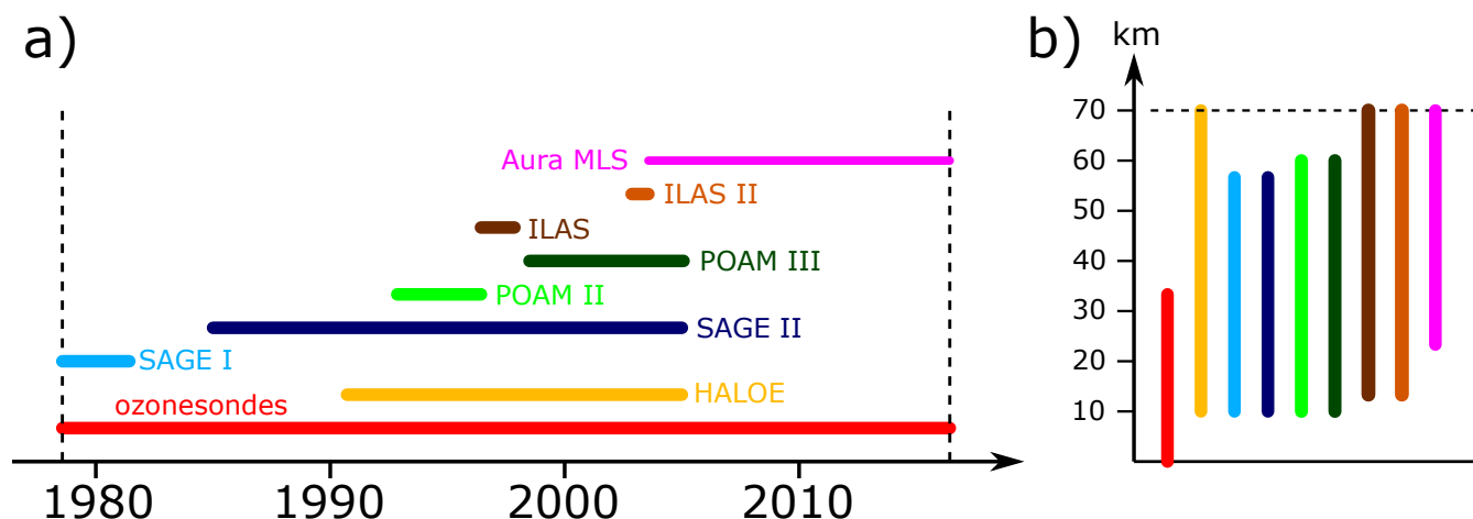
Figure 1. Temporal (a) and vertical coverage (b) of the different ozone data sources used to create the BSVertOzone database. Dashed lines in both parts of the figure denote the BSVertOzone database temporal (1979-2016) and vertical boundaries (0-70km).
