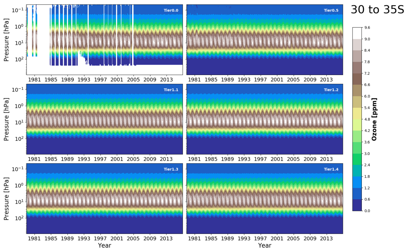
Figure 6. All six Tiers of BSVertOzone for the latitude band 30^{\circ}\text{S} to 35^{\circ}\text{S} (given in ozone mixing ratio on pressure levels).
