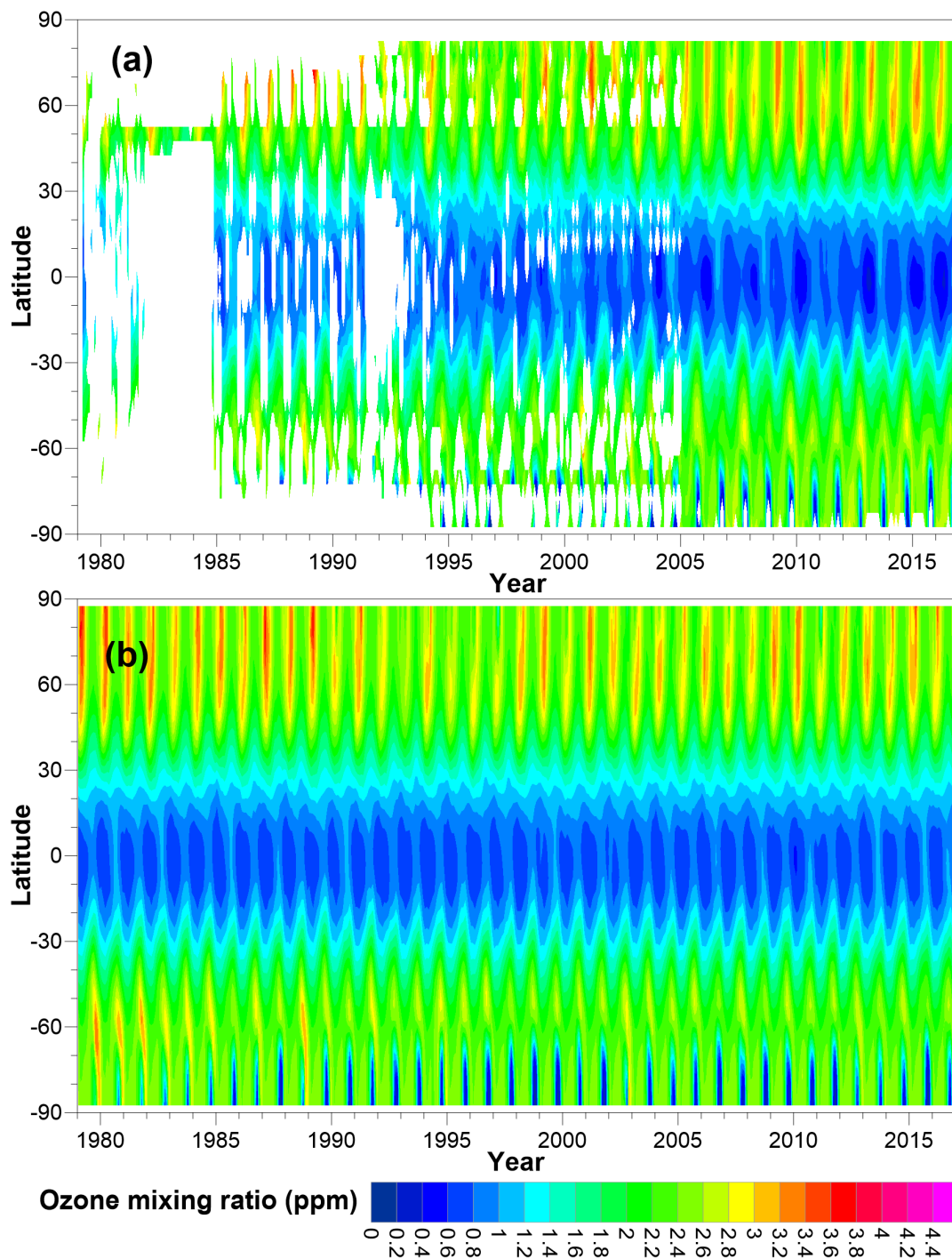
Figure 5. Monthly mean zonal mean ozone mixing ratios at 20hPa for a) unfilled adjusted ozone values from different data sources (Tier 0) and b) pre-filled (Tier 0.5) ozone database. For more details see text.
