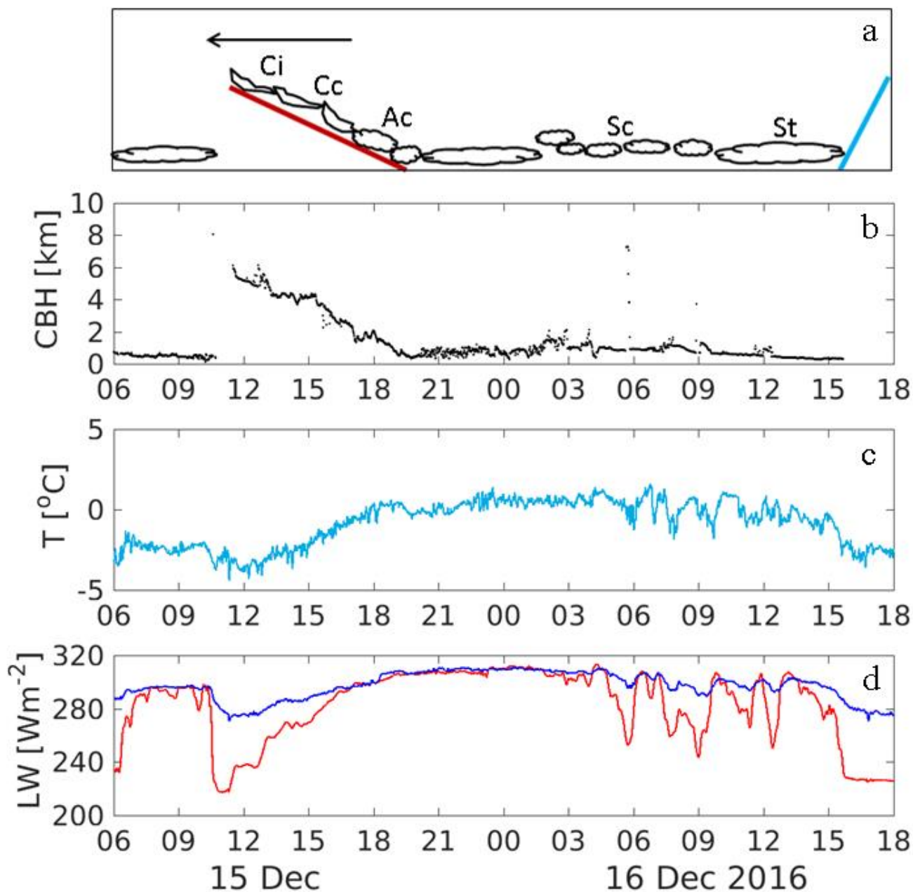
5 Figure 2: A frontal passage on 15 / 16 December 2016 in Ny-Ålesund. a: Schematic diagram of the warm front (red line) and cold front (blue line), their moving direction (black arrow), and associated clouds, respectively. b: Cloud base height (CBH) from ceilometer measurements. c: 2m air temperature from surface meteorological observations. d: Upward and downward longwave radiation (blue and red lines, respectively) from surface radiation measurements.
