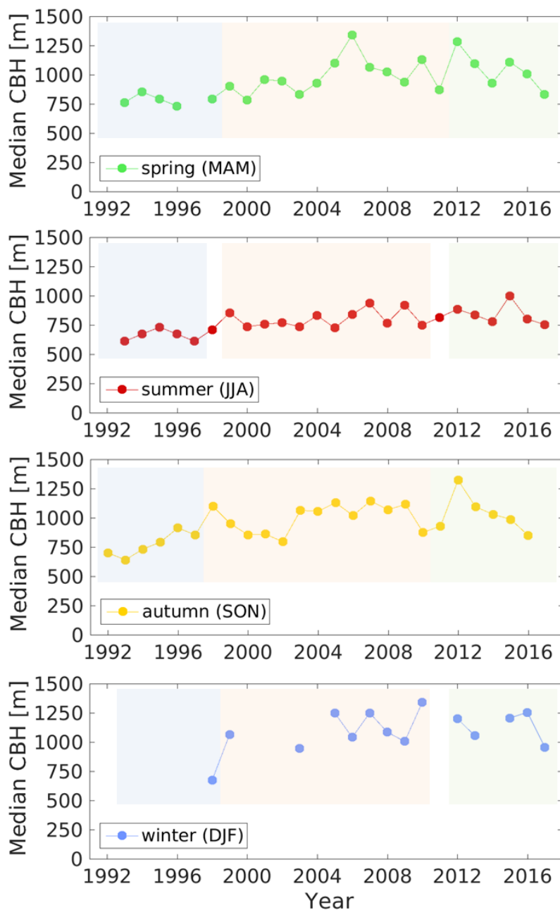
Figure 5: Median cloud base height (CBH) for spring months March-April-May, summer months June-July-August, autumn months September-October-November, and winter months December-January-February, shown from uppermost to lowermost panel, respectively. Only data with >20% available cloud detection data during the season are considered, leading to gaps especially in winter. The background shading indicates the different instrumentation (light blue – LD-WHX, light red – LD-40, light green – CL-51).
