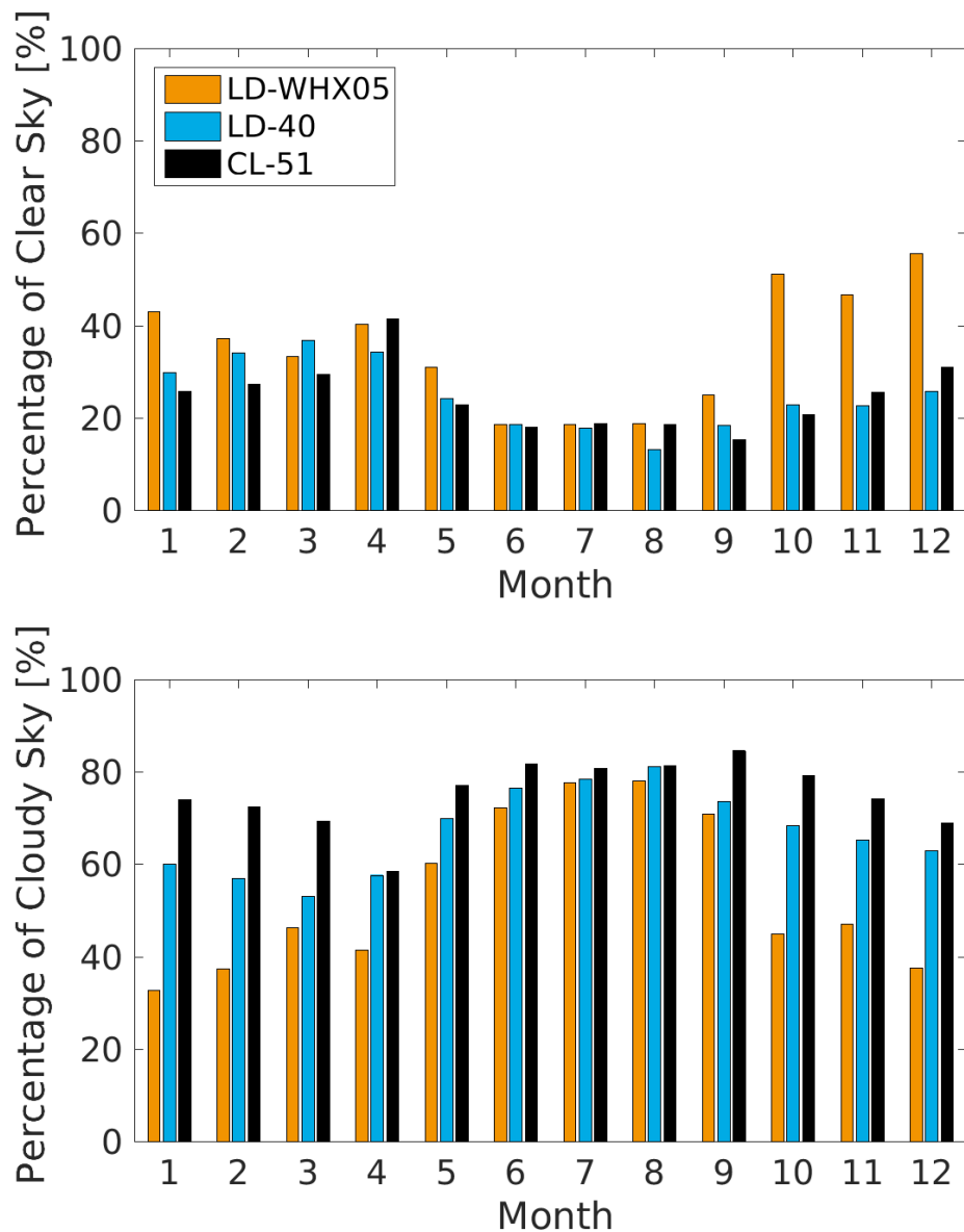
5 Figure 4: Annual cycle of the detected occurrence frequency of clear sky conditions (upper panel) and cloudy conditions (lower panel), given in percent of the total monthly observation times. The average monthly percentage is retrieved from monthly mean values excluding the instrumental overlap months July 1998 and August 2011 as well as months with less than 75% data coverage. The 25-year observation period is presented in the subsets August 1992 to June 1998 (orange), August 1998 to June 2011 (blue), and September 2011 to July 2017 (black) according to the different ceilometer types.
