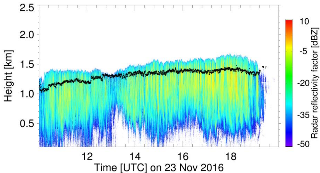
Figure 3: Time-height series of the cloud radar reflectivity factor on 23 Nov 2016 between 10 and 20 UTC at Ny-Ålesund. Black symbols indicate the cloud base height from ceilometer measurements.
