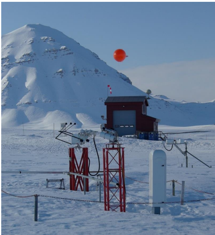
Figure 1: The CL-51 ceilometer located in the vicinity of the radiation measurements of the AWIPEV station at Ny-Ålesund, in April 2013. In the background the balloon facility for radiosonde launches, and a red tethered balloon. (photo: J. Graeser)
