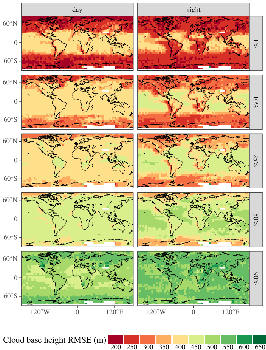
Figure 8. Cloud base uncertainty quantiles. Statistics are calculated within each 5^\circ \times 5^\circ latitude–longitude box. The left (right) column shows statistics of daytime (nighttime) retrievals; daytime and nighttime are defined by the CALIOP VFM product.
