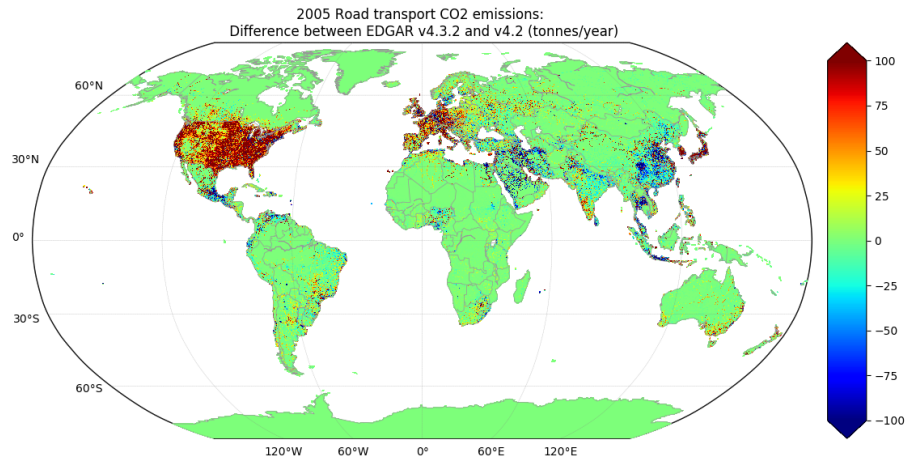
Fig. 2. Difference EDGARv4.3.2 and EDGARv4.2 emissions of CO 2 for road transport (in t/yr per gridcell of 0.1deg)
