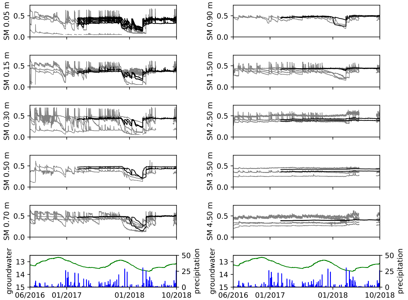
Figure 2. All Level 2 soil moisture (SM) series at depths from 0.05 to 4.50 m in \text{m}^3 \text{m}^{-3} units, groundwater depth below land surface in m, and precipitation ( \text{mm hour}^{-1} ). Soil moisture recorded with SMT100 sensors are in black, soil moisture recorded with TDR sensors are in gray and additionally filtered using a 13 hour moving window.
