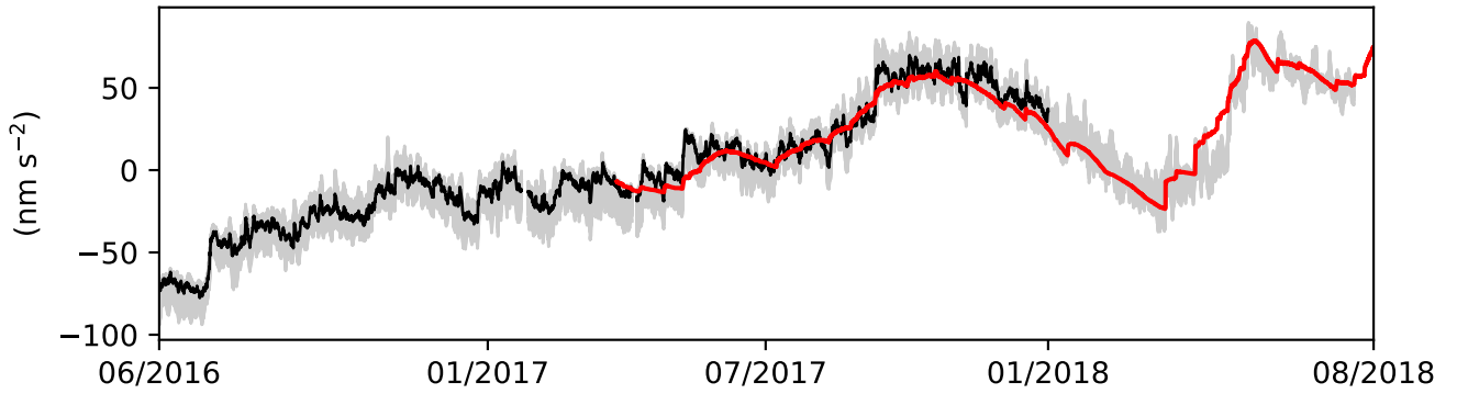
Figure 4. Measured gravity residuals reduced for all available large-scale model combinations (in gray). Model combination Atmacs, ODT, and NOAH025 in black. Red line shows the local gravity model.
