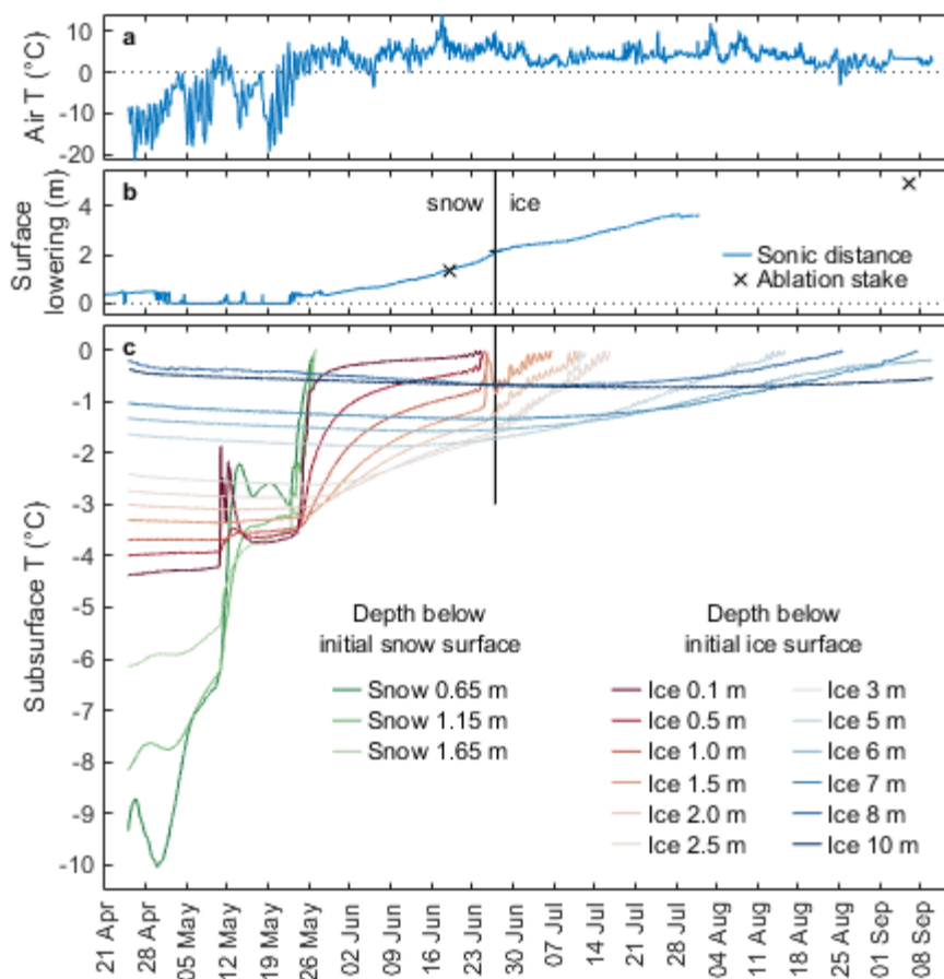
Figure 5. Hourly ice and snow temperature ( T ) measurements from thermistors installed at depth in the snow and ice adjacent to the On-Ice weather station (c). Panel (a) shows air temperature, (b) shows cumulative surface lowering measured by the sonic ranger and ablation stakes. Initial thermistor depths are listed in the legend given in depth below the initial snow surface for the three snow thermistors and depth below the snow-ice surface interface for the 12 ice thermistors. The snow depth at installation on 19 April 2013 was 2.10 m. Note that the instrumentation depth becomes shallower as the glacier surface ablates during the melt season. The onset of large diurnal temperature fluctuations above 0^{\circ}\text{C} indicates that the thermistors have melted out and are affected by solar radiation. After a sensor exceeds 0^{\circ}\text{C} , we do not plot the remaining data.
