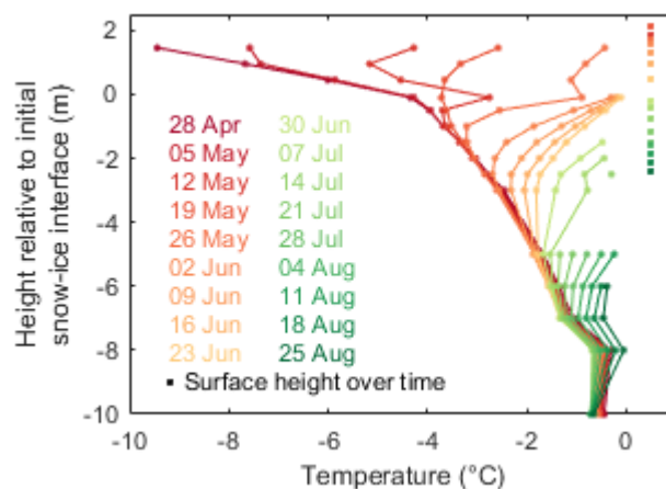
Figure 6. Vertical profiles of temperature in the upper 10 m of the glacier at the On-Ice station in summer of 2013. After a sensor exceeds 0^{\circ}\text{C} , we do not plot the remaining data.
