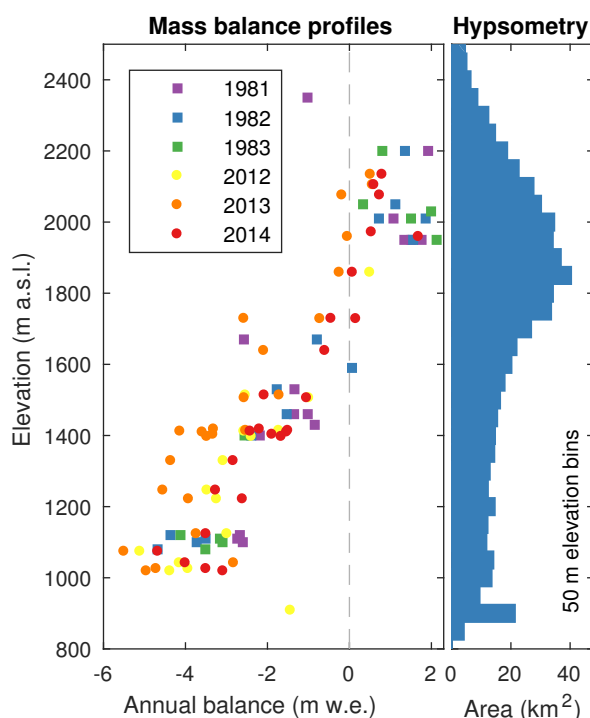
Figure 12. Annual point mass balances on West Fork, Susitna, East Fork, Maclaren, and Eureka Glacier versus elevation. The apparent outlier in 2012 (-1.4 m w.e. at 908 m a.s.l.) was due to debris cover at the site. The hypsometry of all 127 glaciers in the Alaska Range portion of the Susitna basin is also shown in 50 m elevation bands. The hypsometry comes from the Randolph Glacier Inventory (Pfeffer et al., 2014), which used glacier outlines from 2009 and elevation from airborne interferometry ( http://ifsar.gina.alaska.edu ) collected in summer 2010.
