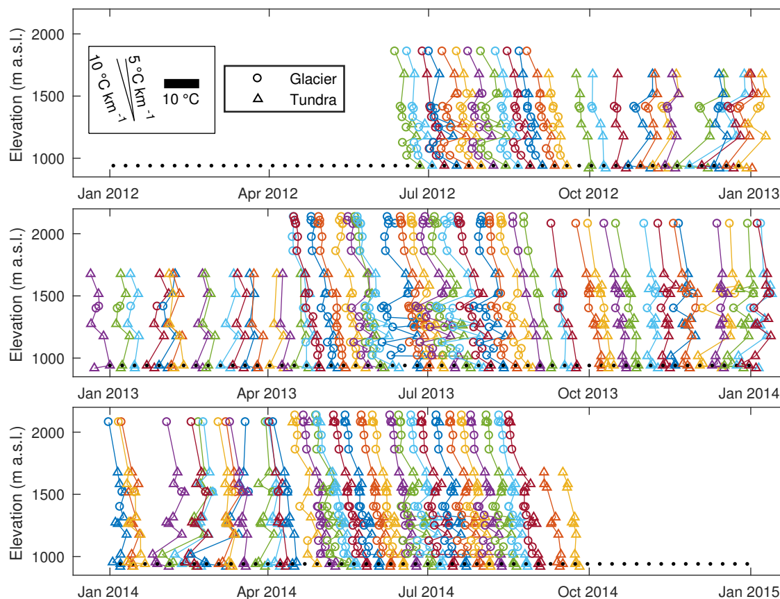
Figure 11. Weekly air temperature profiles show the winter inversions and summer differences between glacier and tundra temperature. Each week's profile is plotted relative to a reference station (Windy Creek Lower, 940 m a.s.l.).
