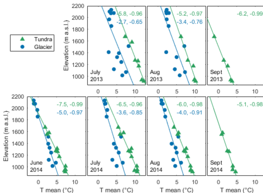
Figure 10. Monthly temperature profiles from simple weather stations on the glaciers and on the tundra. Environmental lapse rates ( ^{\circ}\text{C km}^{-1} ) were calculated by linear regression between monthly average data and station elevations and are reported in the upper right of each subplot, along with the r-value of the fit.
