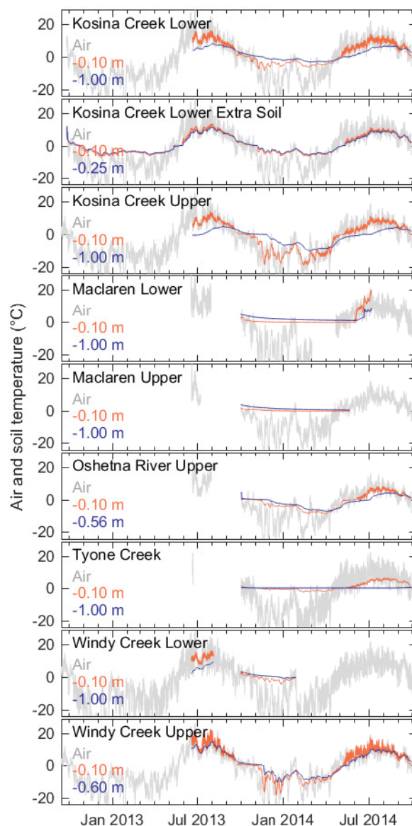
Figure 17. Hourly soil temperatures at depth below the soil surface for all sites with soils data, and air temperatures from each site’s simple AWS. Each panel lists the depth of the soil temperature probes.
