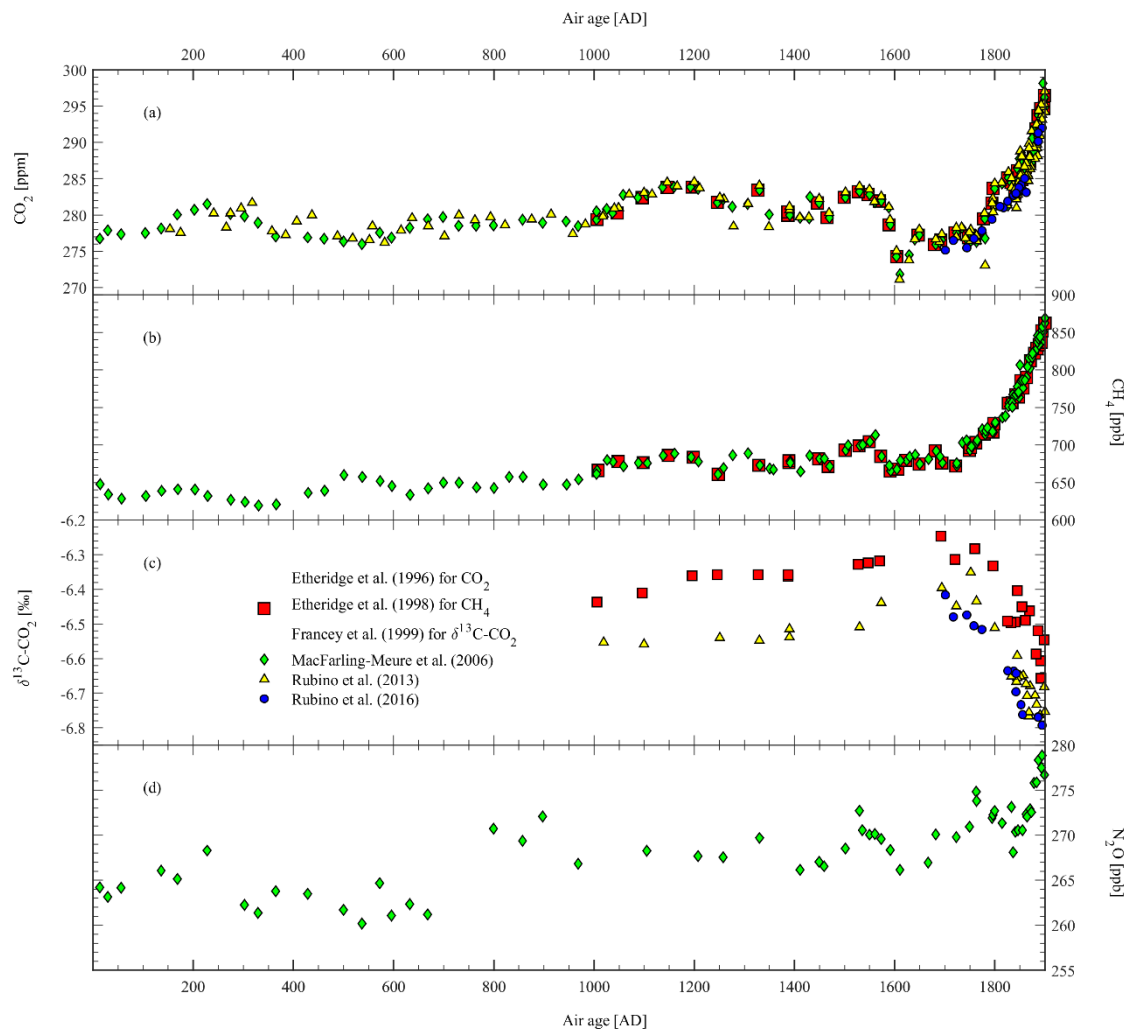
Figure 2: Published Pre-Industrial Period (1-1900 AD) GHG records from Law Dome ice extracted and measured at CSIRO ICELAB-GASLAB.
