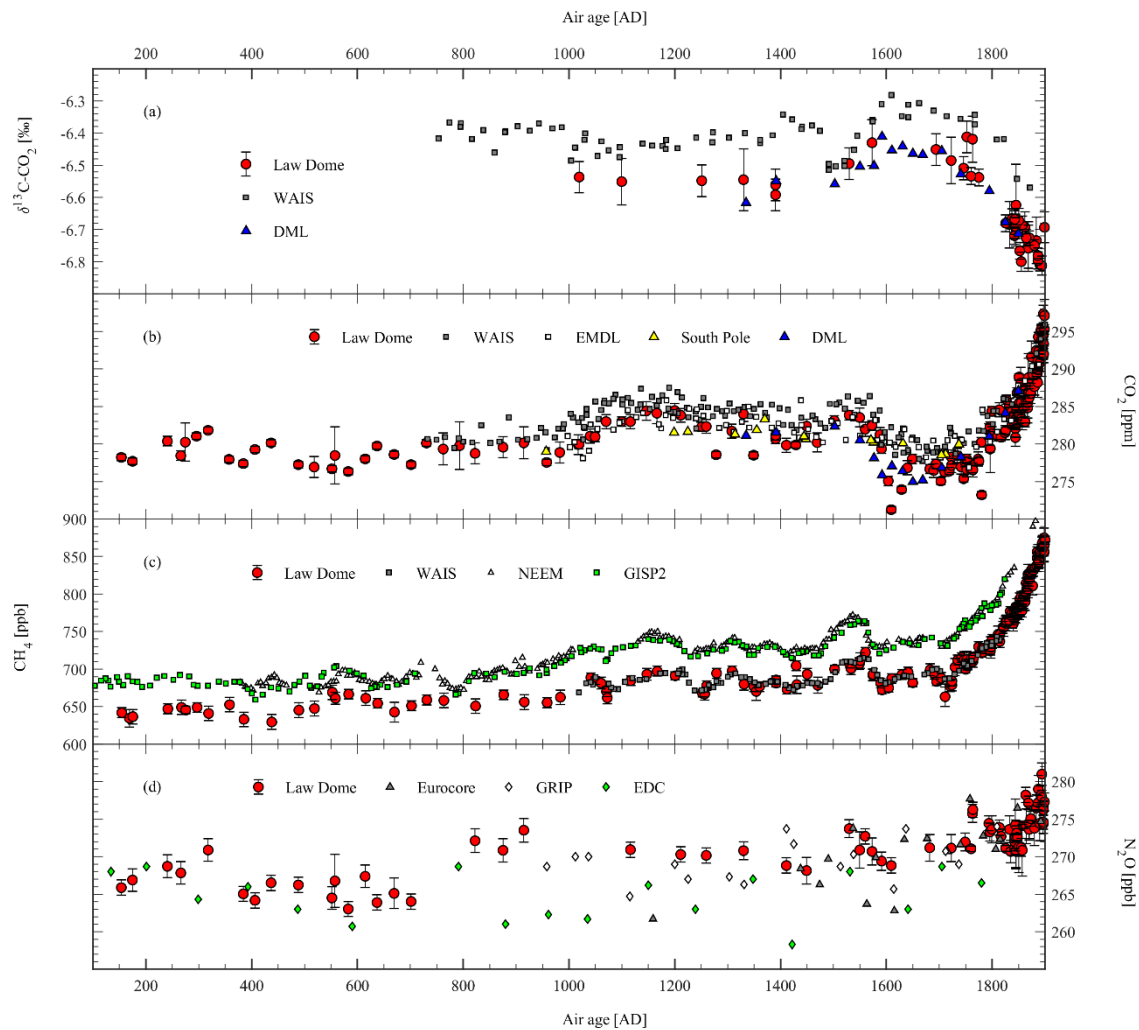
Figure 4: Revised records (100-1900 AD) of (a) \delta^{13}\text{C-CO}_2 ; (b) \text{CO}_2 ; (c) \text{CH}_4 and (d) \text{N}_2\text{O} from Law Dome ice compared to published records from other sites: WAIS- \delta^{13}\text{C-CO}_2 from Bauska et al. (2015), WAIS- \text{CO}_2 from Ahn et al. (2012), DML- \text{CO}_2 and -\delta^{13}\text{C-CO}_2 from Rubino et al. (2016), EDML- and South Pole- \text{CO}_2 from Siegenthaler et al. (2005), WAIS- \text{CH}_4 from Mitchell et al. (2011), NEEM- \text{CH}_4 from Rhodes et al.
