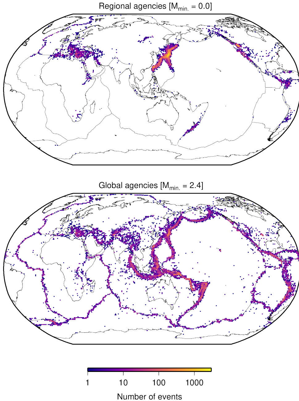
Figure 3. Global maps showing the number of events with at least one source mechanism reported in the ISC Bulletin for the time period from January 1964 to December 2018, in a 1^\circ by 1^\circ grid, for mechanism solutions reported by local and regional agencies (top), and global agencies (bottom, [GCMT, HRVD, IPGP, ISC, MOS, NEIC, NEIS]). Minimum magnitude ( M_{\min.} ) following the scheme described in Di Giacomo and Storchak (2015) is shown on top of each map.
