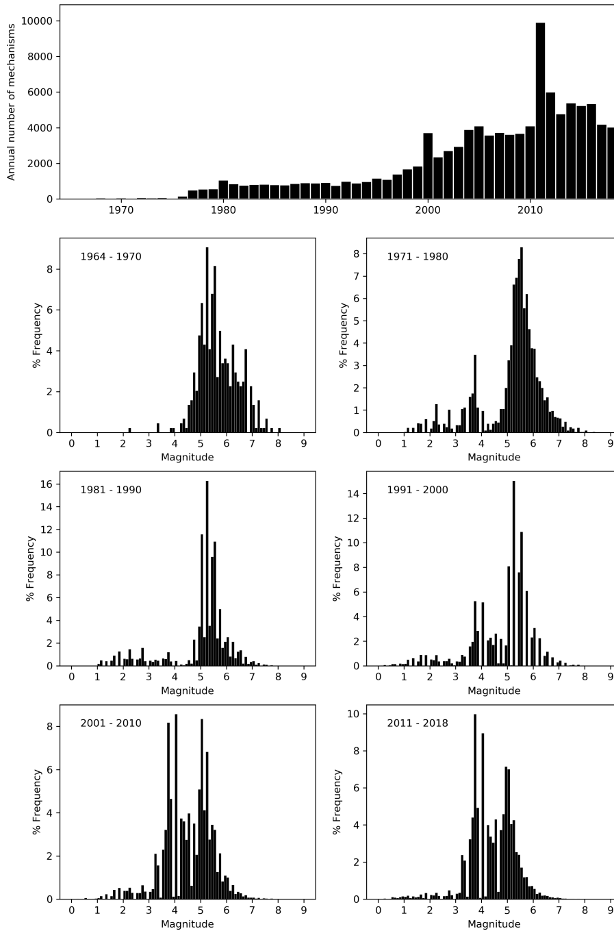
Figure 1. Number of source mechanisms in the ISC Bulletin from January 1964 to December 2018 and normalized frequency - magnitude distributions with respect to different time periods. A magnitude value for each event with an associated source mechanism is selected following the scheme described in Di Giacomo and Storchak (2015). Note the high peak in the top subplot in 2011 which is associated with the 2011 Tohoku earthquake aftershock sequence. A slight dip for year 2018 is only apparent as the data collection is not yet complete.
