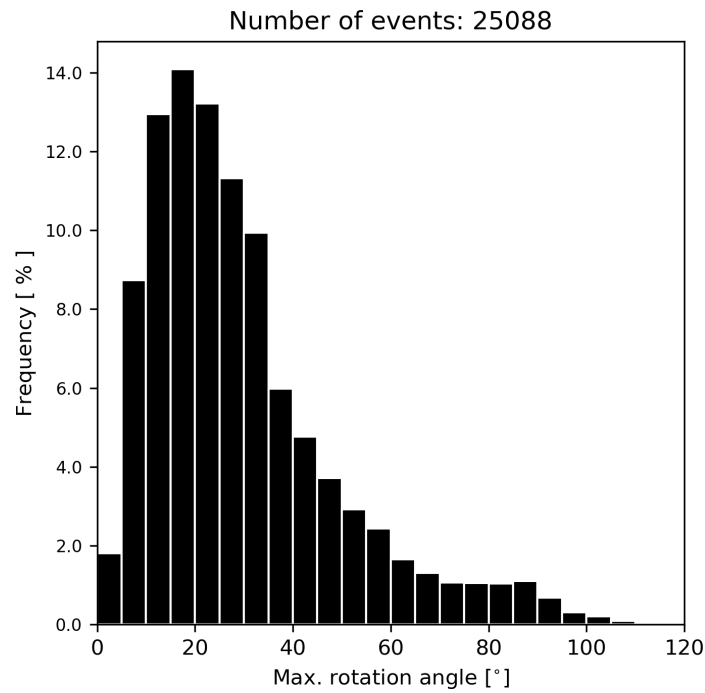
Figure 5. Frequency distribution of available source mechanisms per event in the ISC Bulletin for the time period from January 1964 to December 2018 (top), and intra-event maximum rotation angle frequency distribution for the seismic events having at least two mechanism solutions available (bottom).
