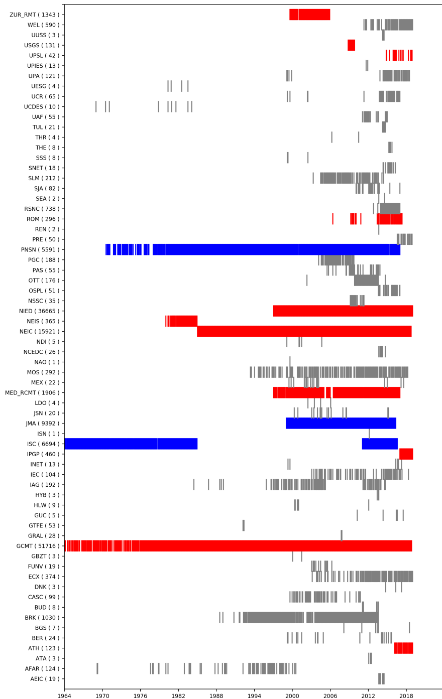
Figure 2. Time distribution of source mechanisms in the ISC Bulletin (January 1964 – December 2018) reported by different agencies. The numbers in brackets next to each agency code shows the total number of reported source mechanism solutions. Red lines indicate waveform inversion techniques, blue lines indicate first motion polarity techniques and grey colour shows cases where there is no information available on the techniques being used or we could not verify them. A detailed list of the reporting agencies is shown in Table 1.
