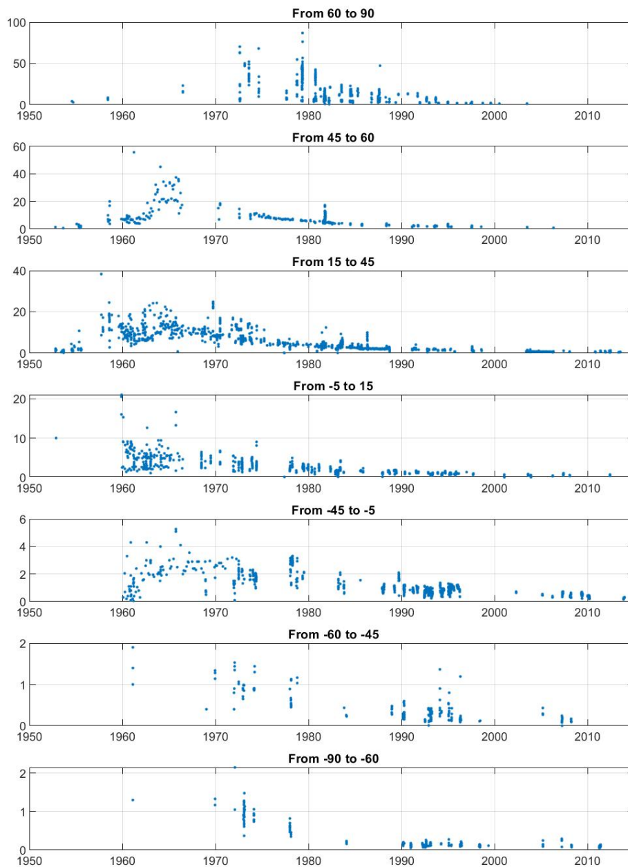
Figure 3: Global ocean surface water (depth < 50 m) tritium concentrations (in TU) for selected latitude bands.
