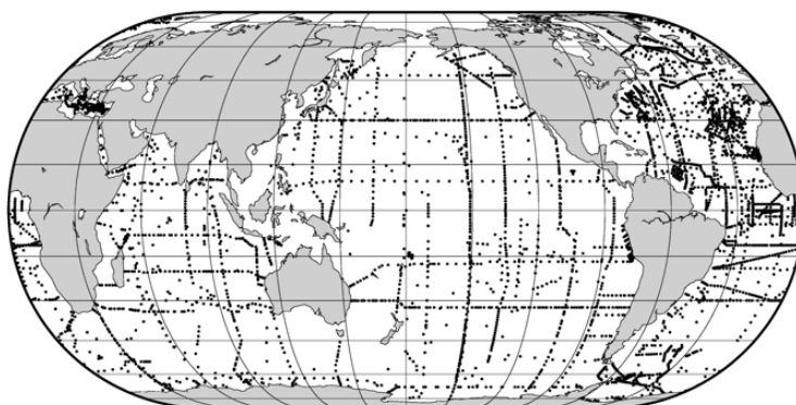
Figure 2: Tritium and helium sample locations
