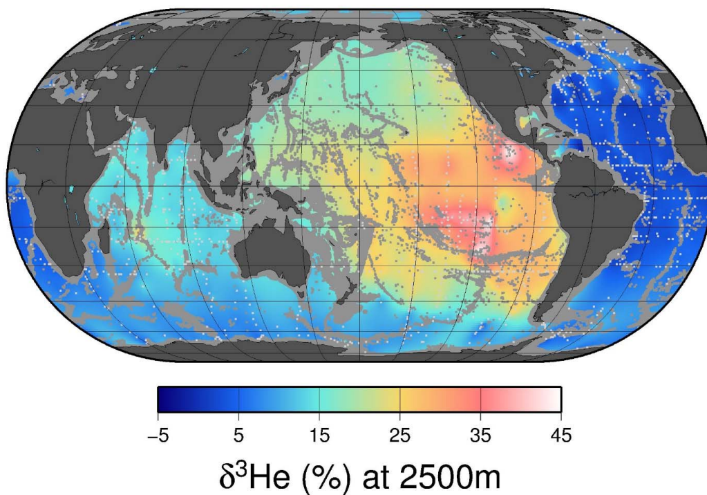
5 Figure 7: A map of \delta^3\text{He} values at approximately 2500 m depth. The values plotted are simply an average of all measurements within a 1^\circ square between 2250 and 2750 dbar. Depths shallower than 2500 m are masked in gray and sampling locations indicated by light gray dots. (Perhaps Reiner or I may do something better here, such as interpolate onto a neutral density surface.)
