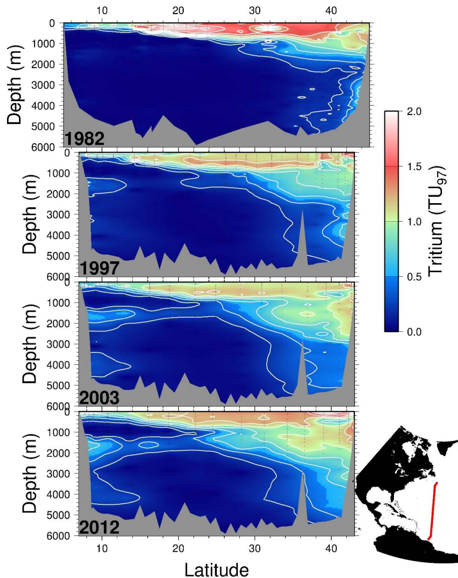
Figure 4: Four meridional tritium sections along roughly 52°W in the North Atlantic taken in 1982, 1997, 2003, and 2012. The tritium concentrations have been decay corrected to a common time (January 1, 1997) for comparison. Contour intervals are 0.2 TU 97 and measurement uncertainties are of order 0.01 TU 97 or better. Due to differences in cruise tracks, the topography for the
