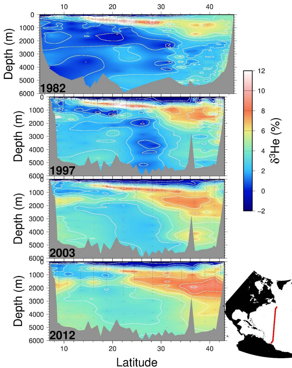
Figure 5: Four meridional \delta^3\text{He} sections along roughly 52^\circ\text{W} in the North Atlantic taken in 1982, 1997, 2003, and 2012. Contour intervals are 1% and measurement uncertainties are 0.15%.
