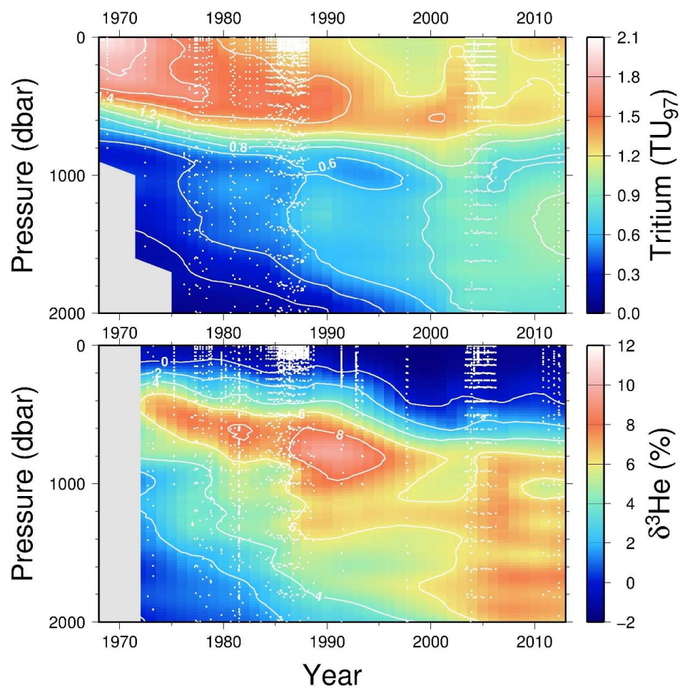
Figure 6: A time series of tritium (upper) and helium isotope measurements in the vicinity of Bermuda (North Atlantic). Tritium values have been decay-corrected to a common time (January 1, 1997). White dots indicate sampling depths and times.
