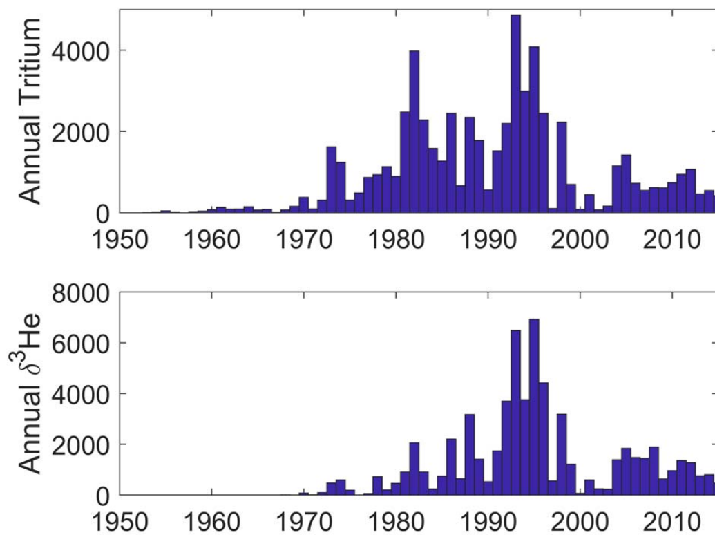
Figure 1: Time distributions of annual tritium (upper panel) and helium (lower panel) measurements.
