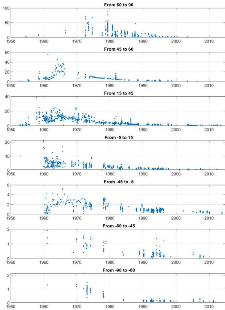
Figure 43: Global ocean surface water (depth < 50 m) tritium concentrations (in TU) for selected latitude bands.
