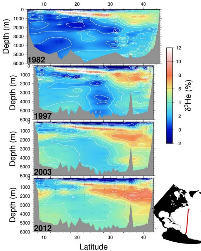
Figure 65: Four meridional \delta^3\text{He} sections along roughly 52°W in the North Atlantic taken in 1982, 1997, 2003, and 2012. Contour intervals are 1% and measurement uncertainties are 0.15%. Due to differences in cruise tracks, the topography for the 1982 occupation differs from the others.
