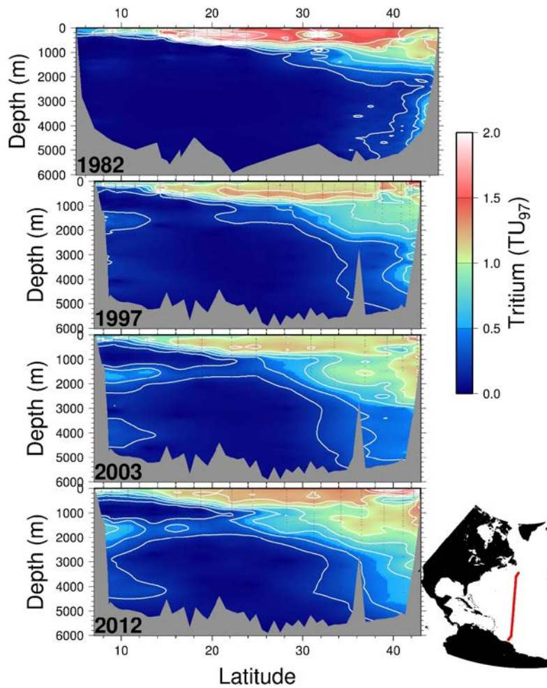
Figure 54: Four meridional tritium sections along roughly 52°W in the North Atlantic taken in 1982, 1997, 2003, and 2012. The tritium concentrations have been decay corrected to a common time (January 1, 1997) for comparison. Contour intervals are 0.2 TU 97 and measurement uncertainties are of order 0.01 TU 97 or better. Due to differences in cruise tracks, the topography for the 1982 occupation differs from the others.
