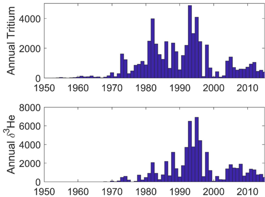
Figure 21: Time distributions of annual tritium (upper panel) and helium (lower panel) measurements.
