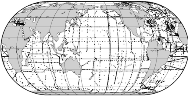
Figure 33: Tritium and helium sample locations
