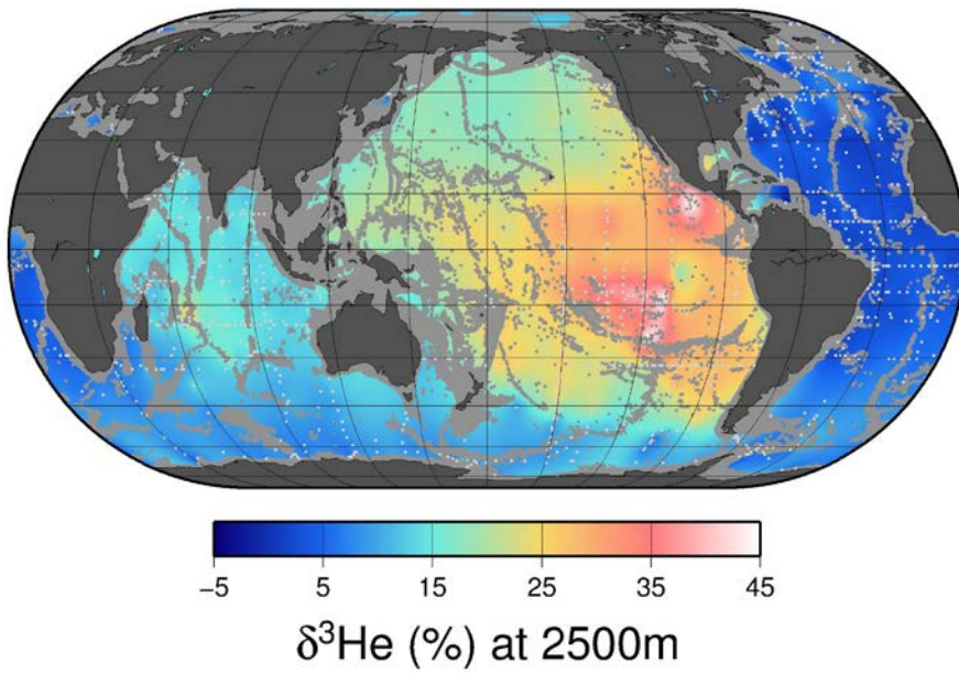
Figure 87: A map of \delta^3\text{He} values at approximately 2500 m depth. The values plotted are simply an average of all measurements within a 1^\circ square between 2250 and 2750 dbar. Depths shallower than 2500 m are masked in gray and sampling locations indicated by light gray dots. (Perhaps Reiner or I may do something better here, such as interpolate onto a neutral density surface.)
