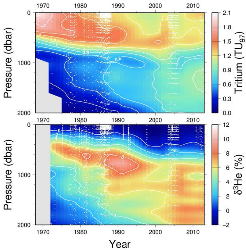
Figure 76: A time series of tritium (upper) and helium isotope measurements in the vicinity of Bermuda (North Atlantic). Tritium values have been decay-corrected to a common time (January 1, 1997). White dots indicate sampling depths and times.
