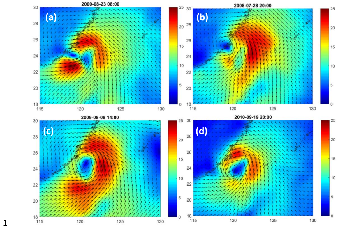
2 Figure 8 Wind patterns at the time close to the start of the SST drop. (a) Typhoon Bilis 3 in 2000. The SST started to decrease on 2000/8/23 at 10:00. The wind pattern was 4 observed on 2000/8/23 at 08:00. (b) Typhoon Fungwong in 2008. The SST started to 5 decrease on 2008/7/28 at 18:00. The wind pattern was observed on 2008/7/28 at 20:00. 6 (c) Typhoon Morakot in 2009. The SST started to decrease on 2009/8/8 at 13:00. The 7 wind pattern was observed on 2009/8/8 at 14:00. (d) Typhoon Fanapi in 2010. The SST 8 started to decrease on 2010/9/19 at 22:00. The wind pattern was observed on 2010/9/19 9 at 20:00
