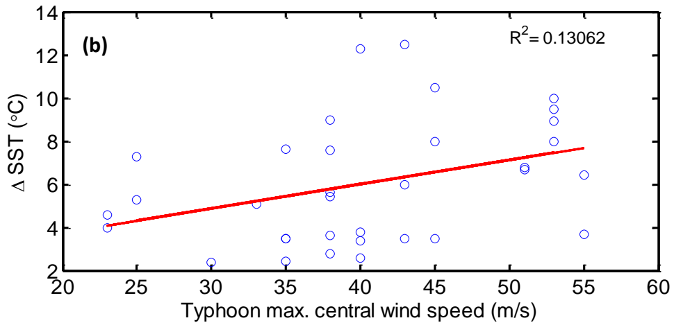
Figure 5 The correlation of \Delta SST with 2 typhoon intensity indicators (a) min. central pressure; (b) max. wind speed
