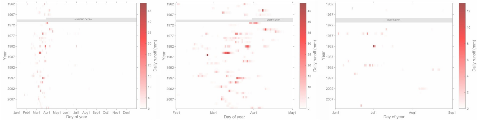
Figure 2. Daily runoff (mm) for the 50-year period (January 1 st 1962 to December 31 st 2011) on Hillslope 2.
