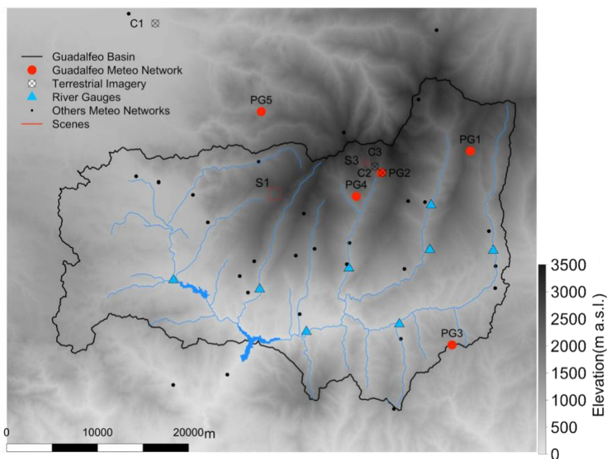
15 Figure 2: The Guadalfeo Network in Sierra Nevada (Spain). PG, weather stations (red circles); C, time-lapse cameras (cross-circles); S, the camera scenes (red rectangles; S2 is a near-field scene and cannot be represented due to its size). Black points identify the location of weather stations belonging to other meteorological networks in the Sierra Nevada area. The limits of the Guadalfeo Experimental Basin (black line), the main river streams (blue line), gauge stations (blue triangles) and reservoirs (blue areas) are included over the elevation map of the area.
