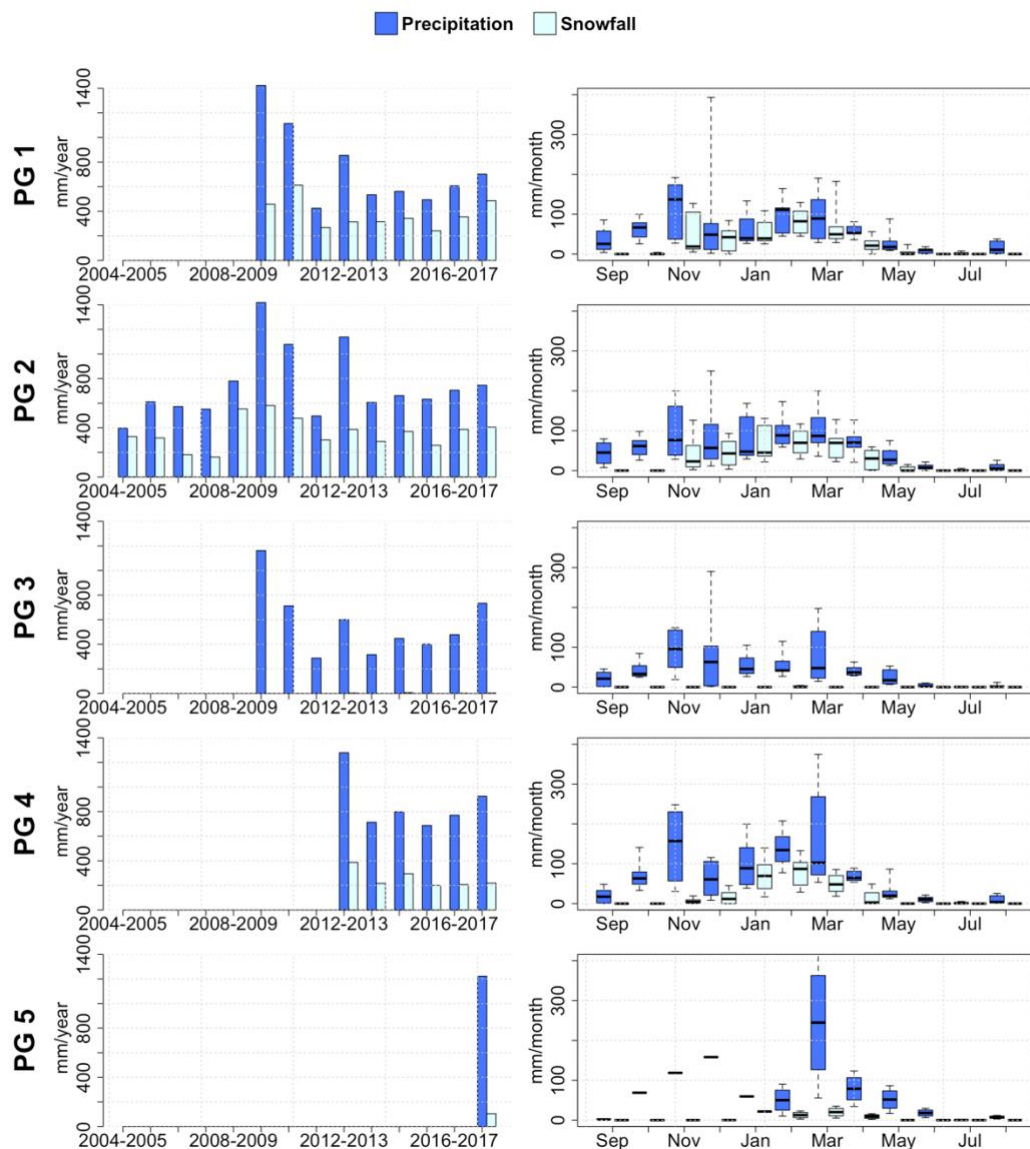
Figure 7: Precipitation and snowfall in the weather stations of the Guadalfeo Network in Sierra Nevada (Spain). Left: Annual precipitation and snowfall at each station during the 2004-2016 period. Right: Mean monthly precipitation and snowfall at each station during the study period; box-plots show the mean values (black line), interval range and the 10 th and 90 th percentiles (whiskers) of each sample (series duration in Figure 3).
