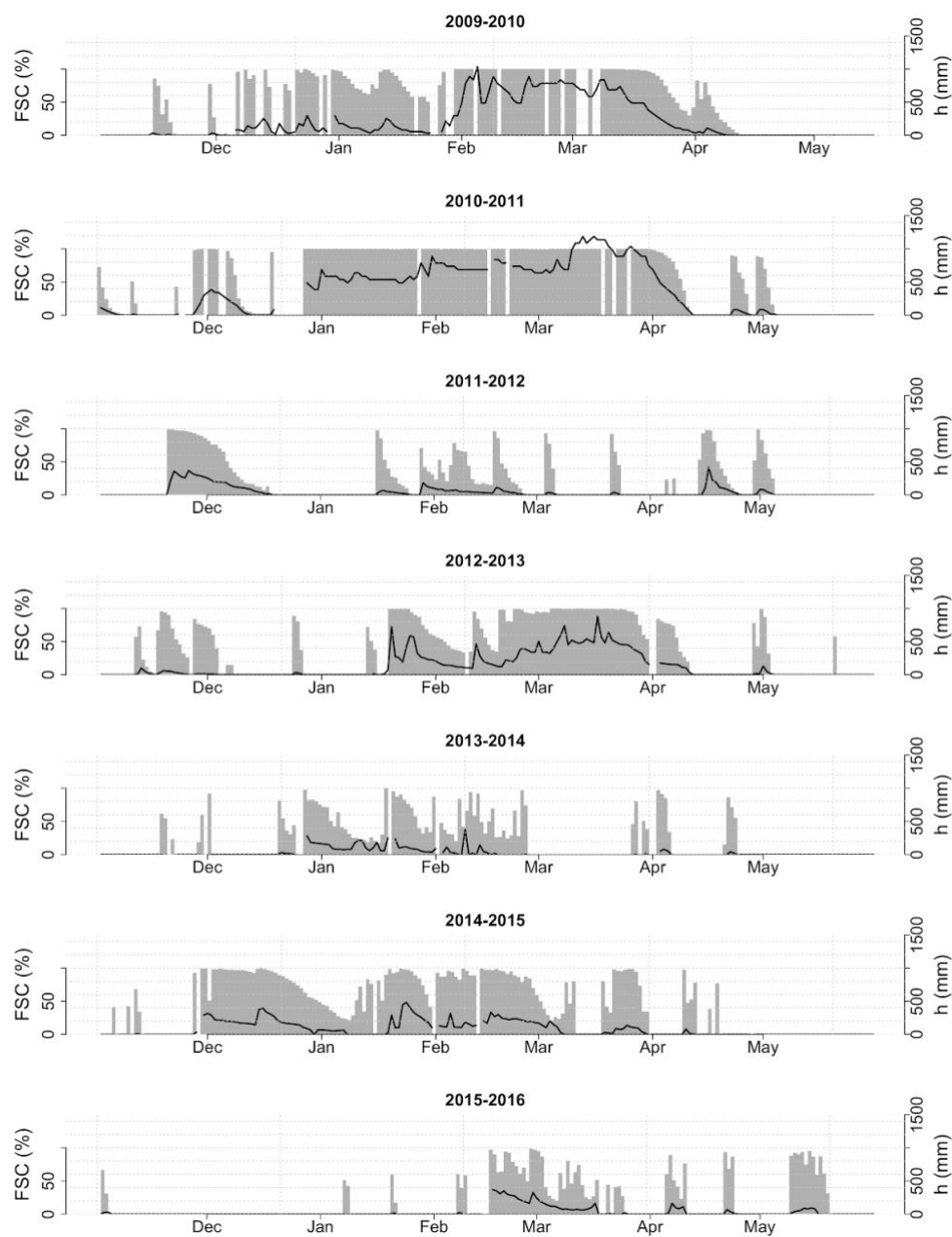
Figure 6: Snow variables retrieved from the images of the time-lapse camera C2 in the Guadafeo Network. Evolution of the observed daily fractional snow cover and snow depth from the 30x30m scene during the snow season (1 Nov-31 May) during each hydrological year of the period 2009-2016.
