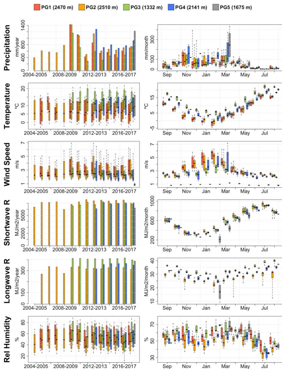
5 Figure 4: Annual and monthly descriptors of the meteorological variables monitored during 2004-2017 by each weather stations in the Guadalfeo Network. Left: annual precipitation, incoming short- and longwave radiation; annual mean daily temperature, wind speed and air relative humidity. Right: mean monthly precipitation, incoming short- and longwave radiation; mean monthly temperature, wind speed and air relative humidity. Box-plots show the median values (black line), the interval range and the 10 th and 90 th percentiles (whiskers) of each sample (series duration in Figure 3).
