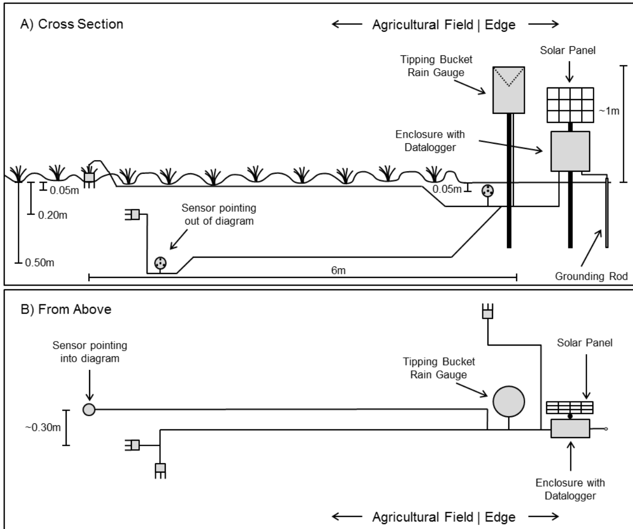
Figure 4. General configuration of 4-probe soil moisture station.
