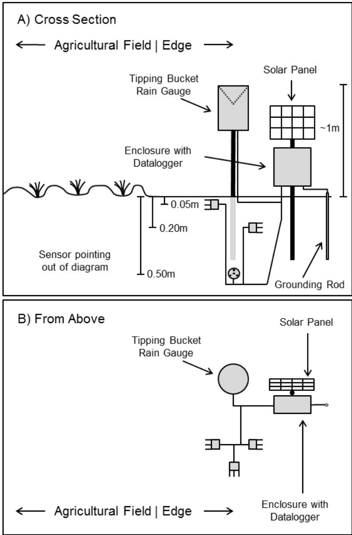
Figure 3. General configuration of 3-probe soil moisture station.
