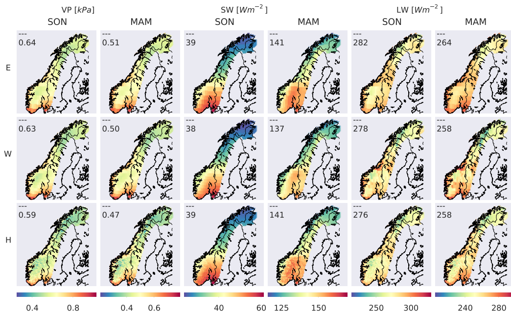
Figure 1. Mean (1982-2000) vapor pressure (VP), incident shortwave (SW \downarrow ) and longwave (LW \downarrow ) radiation estimates in fall (SON) and spring (MAM) of Era-Interim, WFDEI, and HySN. The mean value for the points which are land points for all models are denoted in the upper left corner of each image.
