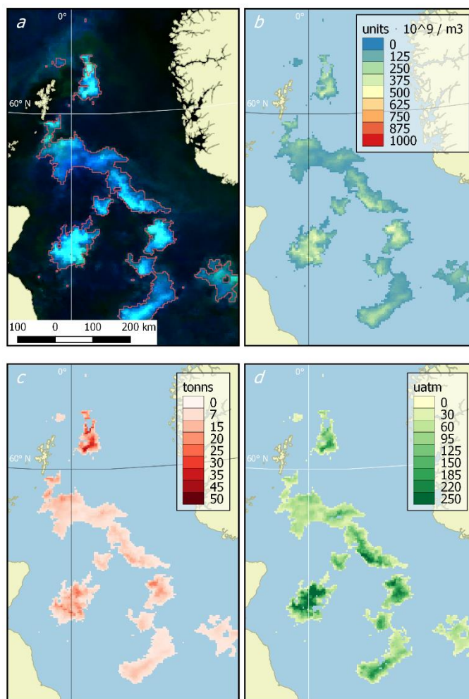
10 Figure 2: Example of dataset products (the North Sea, 2016.06.09). a = source OC CCI RGB imagery with the bloom mask contoured in red, b = coccolith concentration ( 10^9 \cdot \text{m}^{-3} ), c = content of particulate inorganic carbon (tonnes), d = increase in \text{CO}_2 partial pressure in water ( \mu\text{atm} ).
