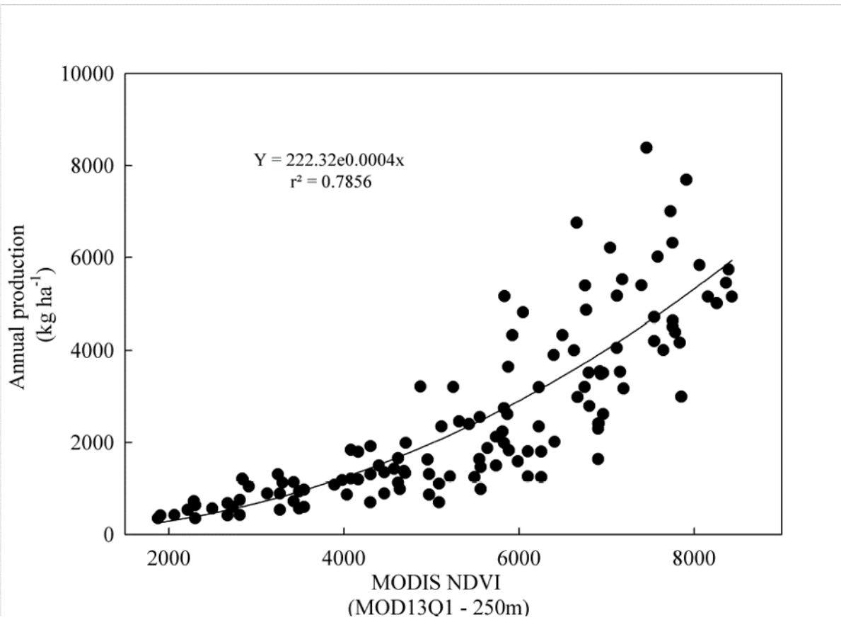
Figure 8. Relationship between annual production and annual maximum NDVI on 51 grassland vegetation types.
