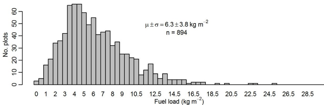
Figure 4. The distribution of surface fuel loading for the FIA plots of three FTG: Loblolly/shortleaf pine (160), Douglas-fir (200), and California mixed conifer (370).
