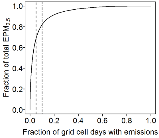
Figure 17. Cumulative distribution of daily PM 2.5 emissions aggregated on a 10 km × 10 km grid. Dashed line and dashed – 5 dotted line mark 5% and 10% of grid cell days with emissions.
