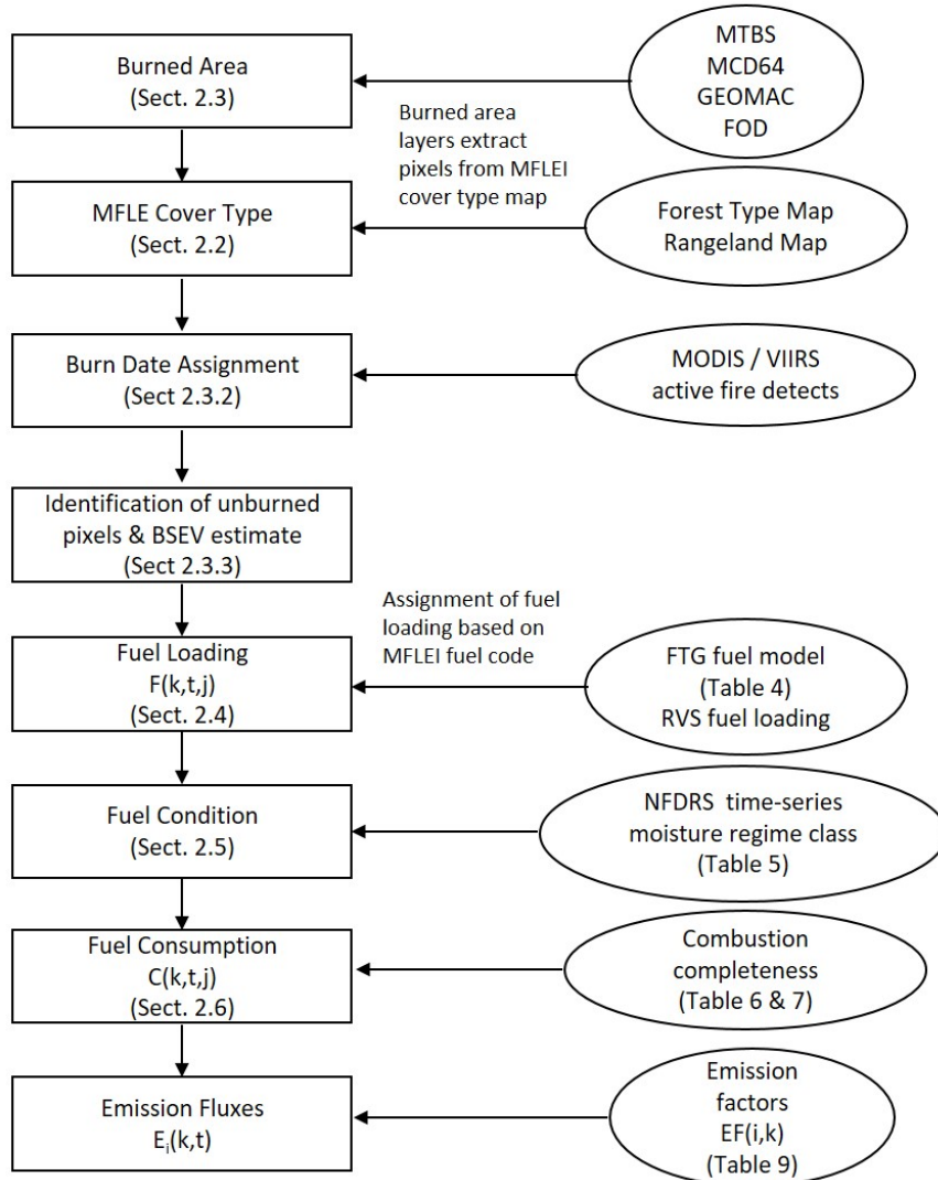
Figure 1. Diagram of MFLEI biomass burning emission model methodology and datasets.
