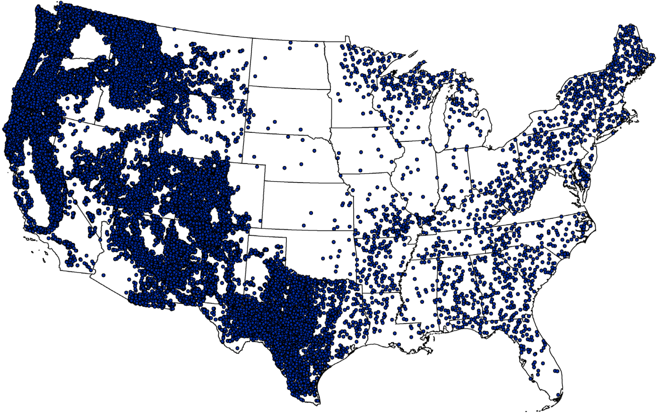
5 Figure 3. Location of FIA plots used to develop surface fuel loading classifications.
