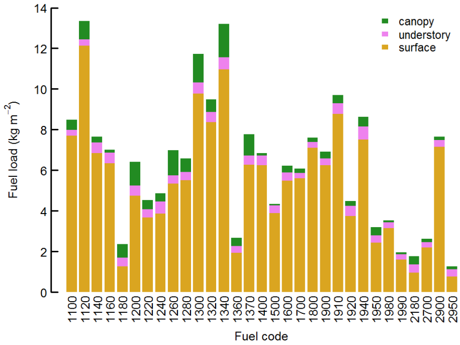
Figure 5. Best estimate (Table 4) forest fuel loading in canopy, understory, and surface fuels by fuel type.
