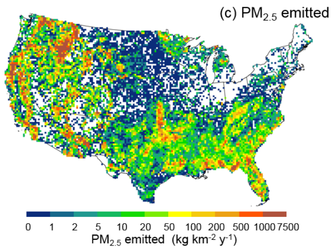
Figure 11. Annual burned area, fuel consumed, and PM 2.5 emitted averaged over 2003-2015.
