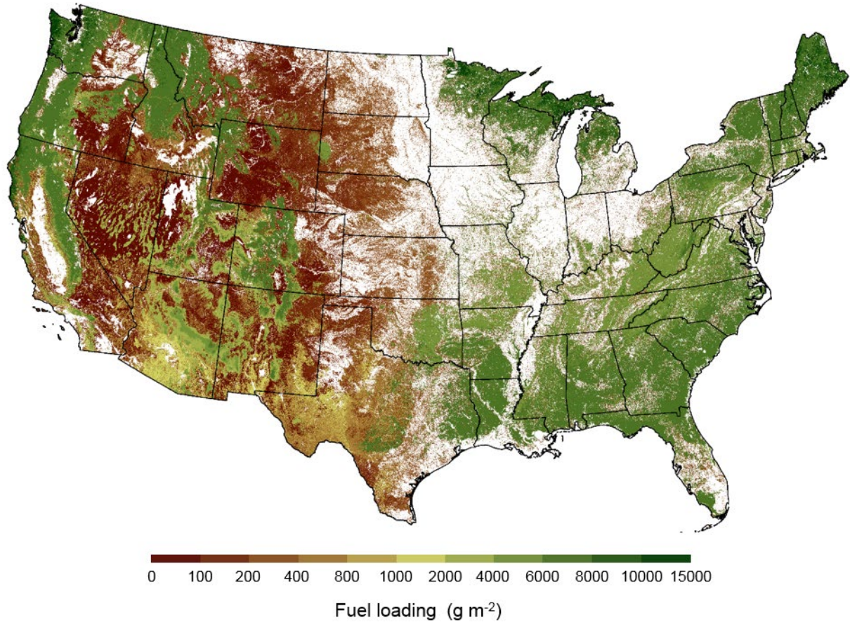
Figure 9. Map of best estimate fuel loading for forest and rangelands in \text{g m}^{-2} .
