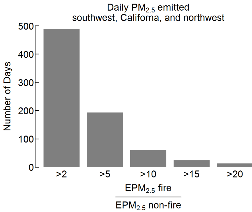
Figure 19. Number of days over 2003-2015 when the wildfire to non-wildfire PM 2.5 emission ratio in the west exceeds thresholds of 2, 5, 10, 15, and 20.
