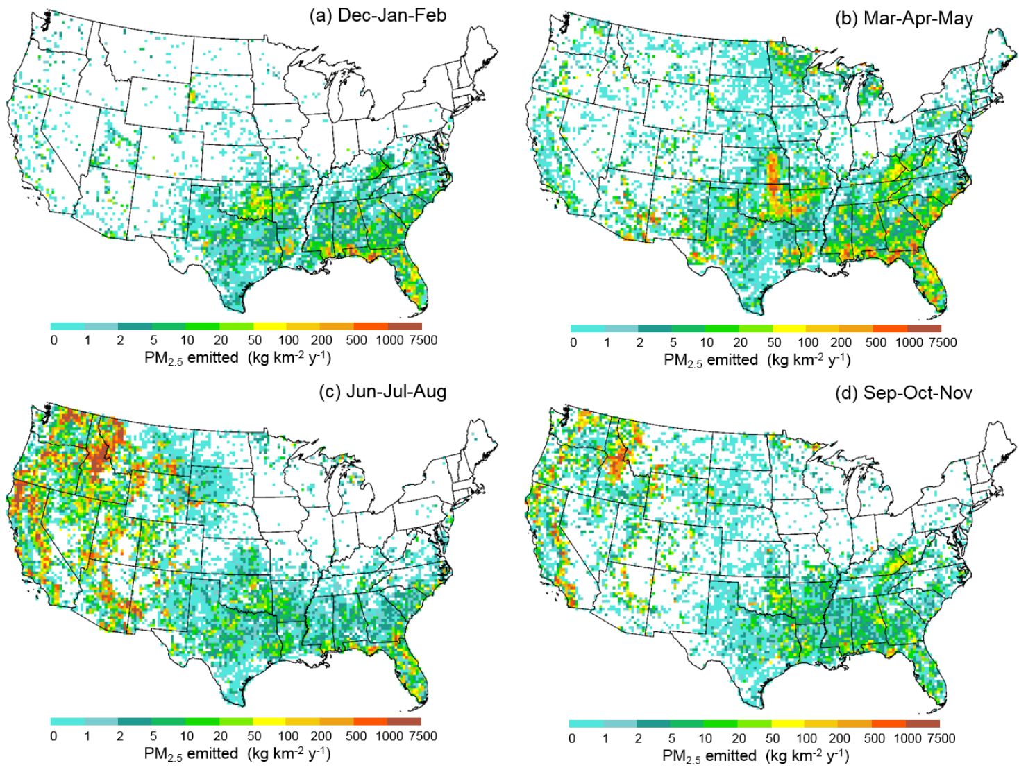
Figure 13. Seasonal PM 2.5 emitted average over 2003-2015.
