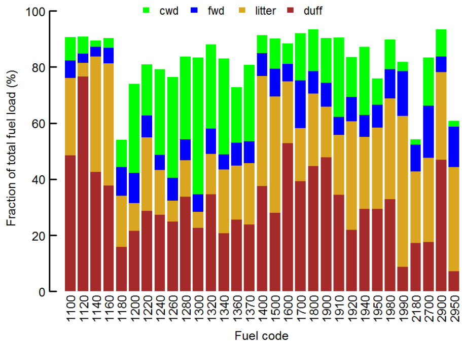
Figure 6. Fraction of best estimate total forest fuel loading in surface fuel loading groups (Table 4) by fuel type.
