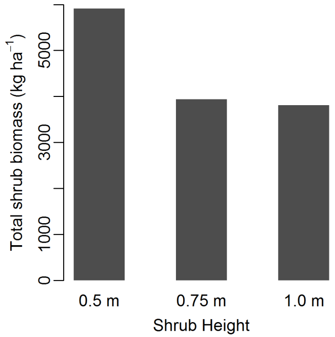
5 Figure C1. Total shrub biomass estimates for a pixel with EVT class of Big Sagebrush shrubland, EVH class of 105, and EVC class of 112 (see text).
