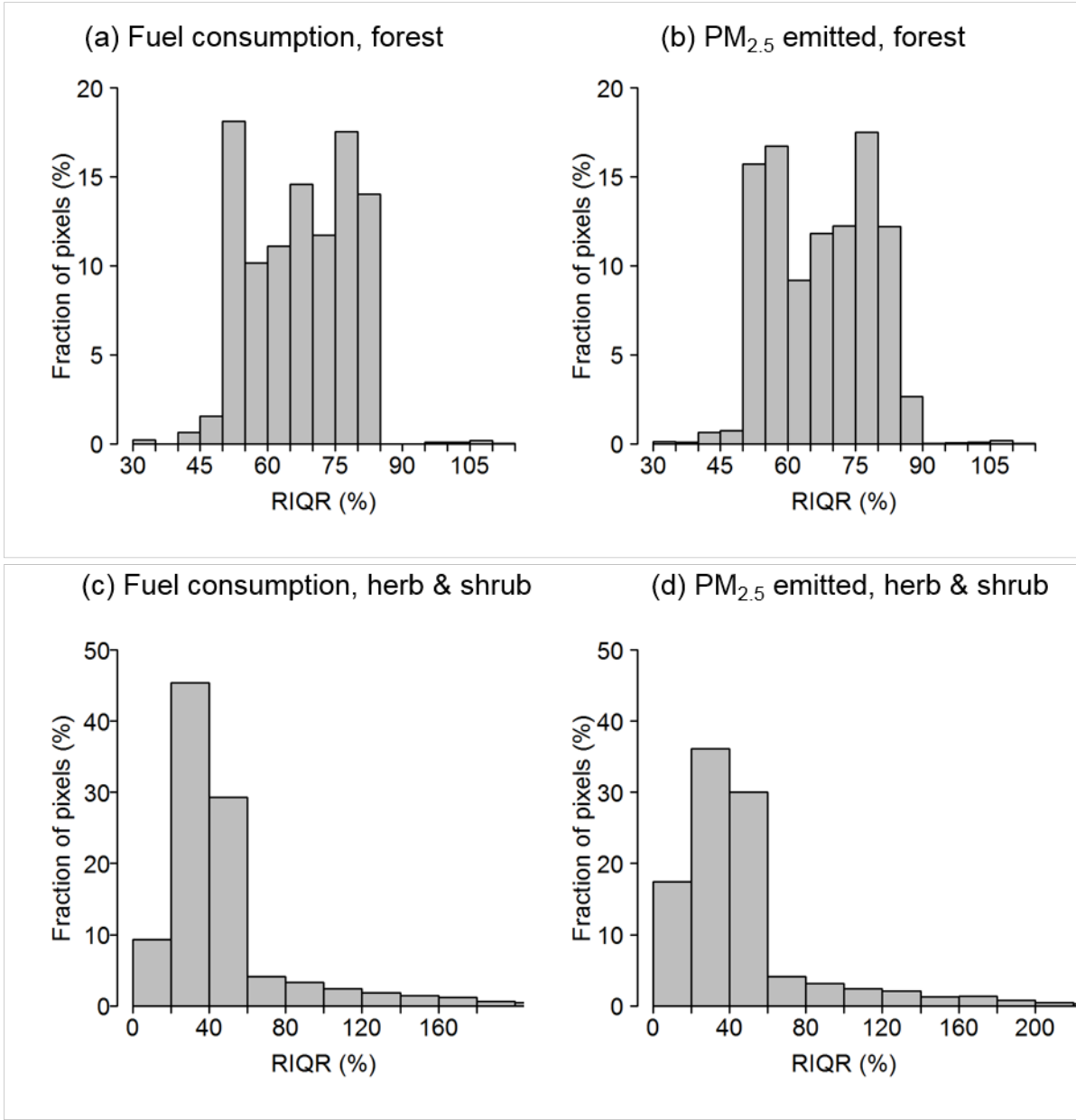
5 Figure 20. Distribution of relative interquartile range from pixel level Monte Carlo style simulations.
