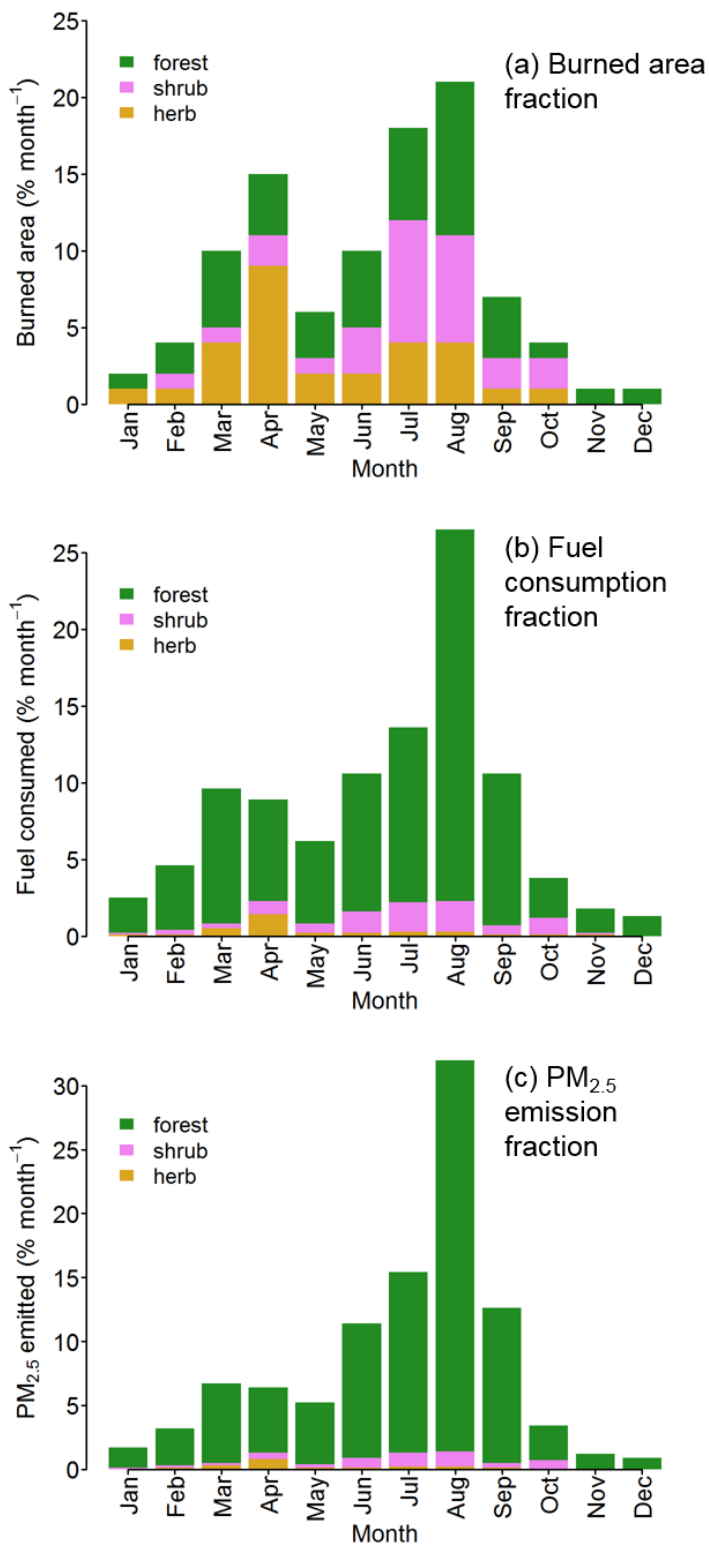
Figure 12. Monthly distributions of burned area, fuel consumption, and PM 2.5 emitted over 2003-2015, broken down by cover type.
