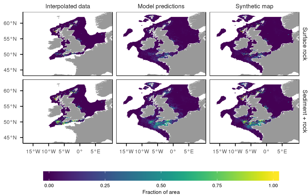
Figure 9. Proportion of area in each rock classification. Areas were classified by whether there was rock at the surface or a surface sediment layer plus rock in the top 50 cm. Historical survey logs and borehole records were first interpolated to provide a map of rock cover where we have sufficient data. Random forests were used to predict rock cover elsewhere using wave and tidal velocities, bathymetry, measures of bathymetry variation and distance from the coast as predictors.
