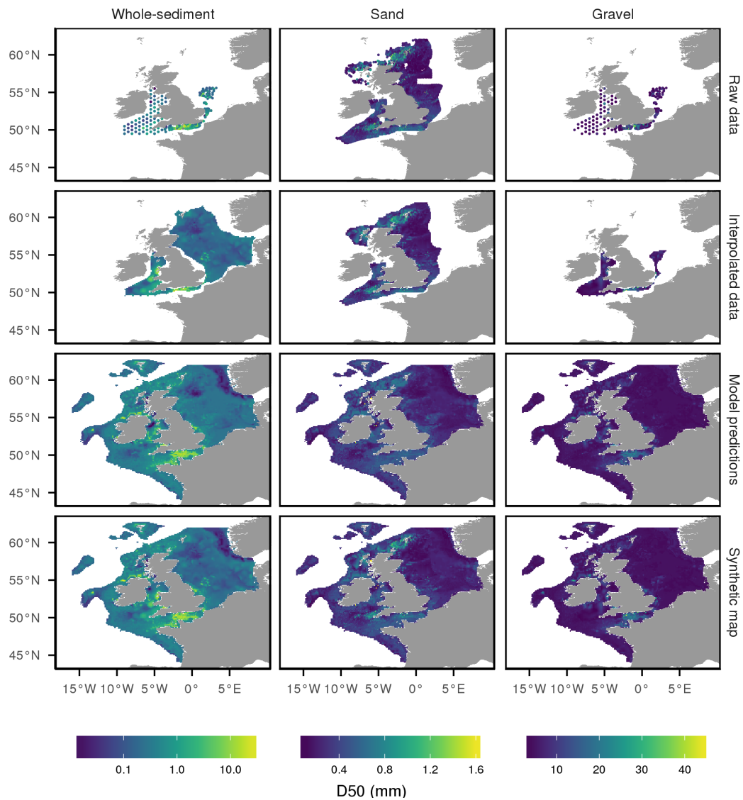
Figure 7. Summary of derivation of the synthetic median grain size maps. Where we have sufficient median grain size data we spatially interpolated a map of D50. In other locations we used the synthetic map of mud, sand and gravel percentages and a GAM model which relates the D50 to the mud, sand and gravel percentages to predict the D50.
