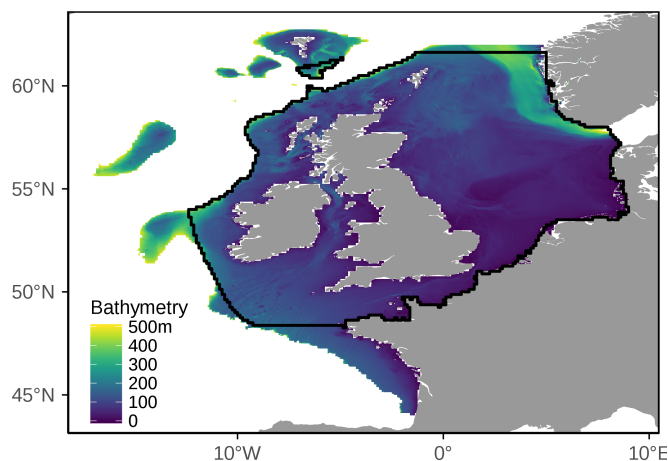
Figure 1. Region where the sedimentary environment was mapped. We defined the northwest European Shelf as the region between 17° W and 9° E and 44° N and 63° N , where bathymetry was less than 500 m. The solid black line demarcates the region where tidal velocities were taken from the Scottish Shelf Model, as described in section 2.2.4.
