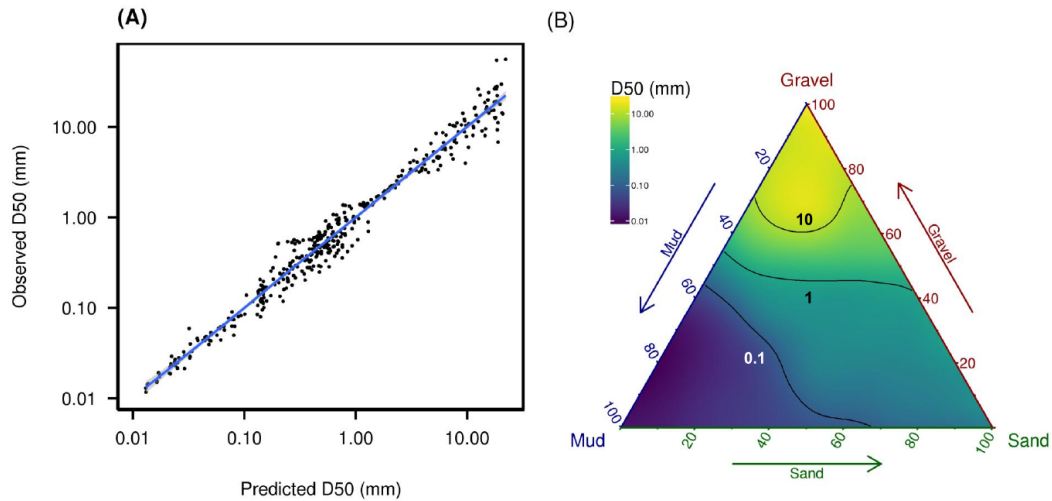
Figure 6. A: Predictions of a GAM model that relates whole-sediment D50 to the mud, sand and gravel percentages. B: Relationship between total sediment median grain size and percentage mud, sand and gravel. The relationship was derived using a general additive model which relates the D50 to the mud, sand and gravel percentage.
