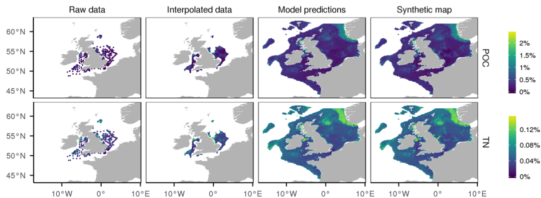
Figure 10. Derivation of the synthetic maps of particulate organic carbon (POC) and total-nitrogen (TN) of sediments . Data was interpolated based on field observations in areas with good spatial coverage. In other regions, parameters were predicted using a random forest which had mud content and physical environmental variables as predictors.
