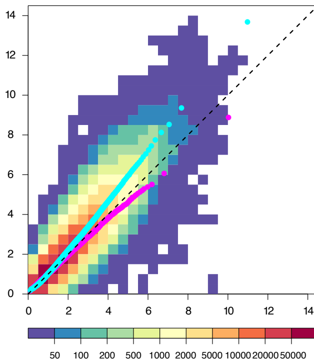
Figure 6. Scatter and quantile-quantile plot of observed (x-axis) and coastDat2 hindcast (y-axis) SWH [m]. Coloured squares indicate the number of the data in each 0.5 m x 0.5 m bin. Coloured dots represent the percentile values of the quantile-quantile plots between observed and coastDat2 hindcast significant wave heights (cyan) and between observed and ERA-Interim SWH (magenta).
