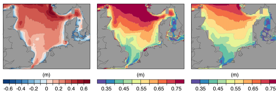
Figure 4. Spatial distribution of bias (left), root mean square distance (middle) and standard deviation of the error (right) [m] between SWHs derived from the coastDat2 hindcast and the ERA-Interim reanalysis for the period 1980–2014.
