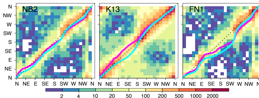
Figure 9. Scatter and quantile-quantile plot of observed (x-axis) and coastDat2 hindcast (y-axis) mean wave direction. Coloured squares indicate the number of counts in each 15^\circ \times 15^\circ bin. Coloured dots represent the percentile values of the quantile-quantile plots between observed and coastDat2 hindcast mean wave directions (cyan) and between observed and ERA-Interim mean wave directions (magenta). Note that the comparison is made for different periods according to data availability (see Table 1).
