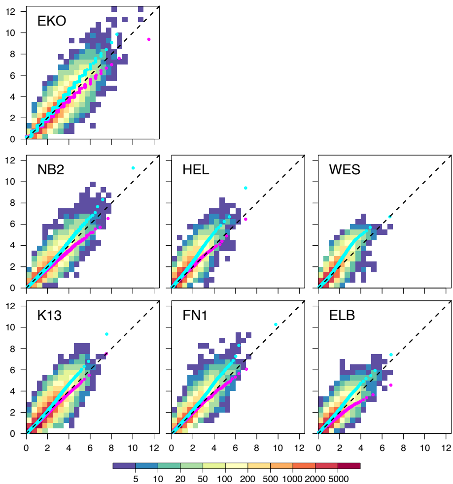
Figure 2. Scatter and quantile-quantile plot of observed (x-axis) and coastDat2 hindcast (y-axis) SWH [m]. Coloured squares indicate the number of data in each 0.5 m x 0.5 m bin. Coloured dots represent the percentile values of the quantile-quantile plots between observed and coastDat2 hindcast (cyan) and between observed and ERA-Interim reanalysis significant wave heights (magenta). Note that the comparison is made for different periods according to data availability (see Table 1).
