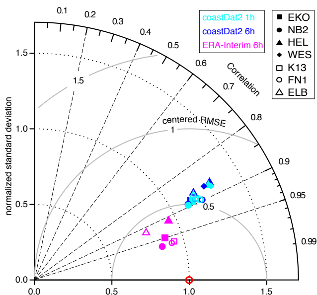
Figure 3. Normalized Taylor diagram from hourly (cyan) and six hourly (blue) coastDat2 SWHs and from six-hourly ERA-Interim (magenta) SWHs at seven (coastDat2) and at six (ERA-Interim) observational sites. The red circle would represent a perfect model compared to the observations.
