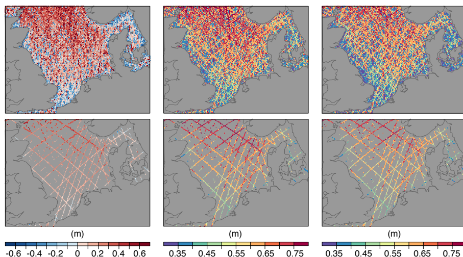
Figure 5. Spatial distribution of bias (left), root mean square error (middle) and standard deviation of the error (right) [m] between SWHs from the coastDat2 hindcast and the GlobWave data set for the period 1992 – 2014 when all available satellite data are used for comparison (top) and when only data with more than 100 flyovers per grid point are used (bottom).
