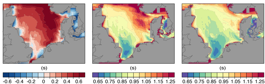
Figure 8. Spatial distribution of bias (left), root mean square error (middle) and standard deviation of the error (right) [s], between the mean wave period between from the coastDat2 hindcast and ERA-Interim reanalysis for the period 1980 – 2014.
