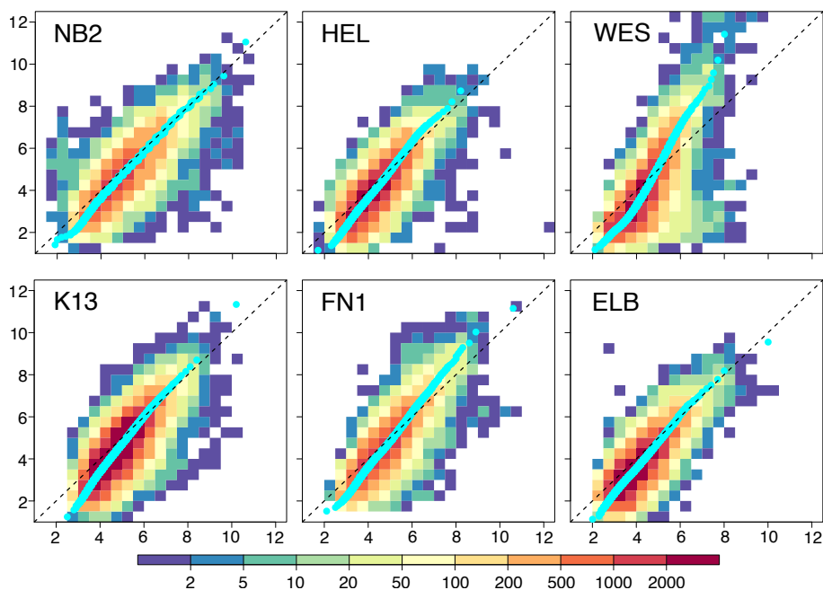
Figure 7. Scatter and quantile-quantile plot of observed (x-axis) and coastDat2 hindcast (y-axis) T_{m02} wave period [s]. Coloured squares indicate the density of the data in each 0.5 s x 0.5 s bin. Coloured dots represent the percentile values of the quantile-quantile plots between observed and coastDat2 hindcast T_{m02} (cyan) wave periods. Note that the comparison is made for different periods according to data availability (see Table 1).
