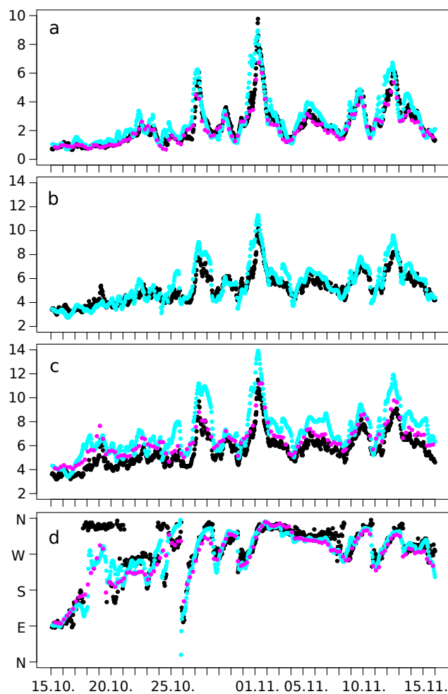
Figure 10. Time series of significant wave height [m] (a), T_{m02} [s] (b) and mean wave period [s] (c) and mean wave direction [°] (d) at FN1 for the period 15 October 2006, 00:00 UTC to 15 November 2006, 00:00 UTC. Observations are shown in black (a–d), the coastDat2 hindcast is shown in cyan (a–d) and the ERA-Interim data are shown in magenta (a,c,d).
