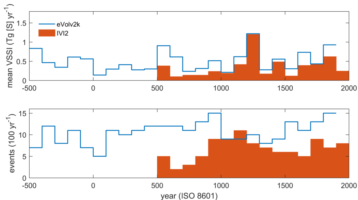
Figure 4: (a) Centennial mean volcanic stratospheric sulphur injections (VSSI) from the IVI2 and eVolv2k reconstructions. (b) The number of volcanic events per century included in the eVolv2k and IVI2 reconstructions. Years are shown using the ISO 8601 standard, which includes a year zero.
