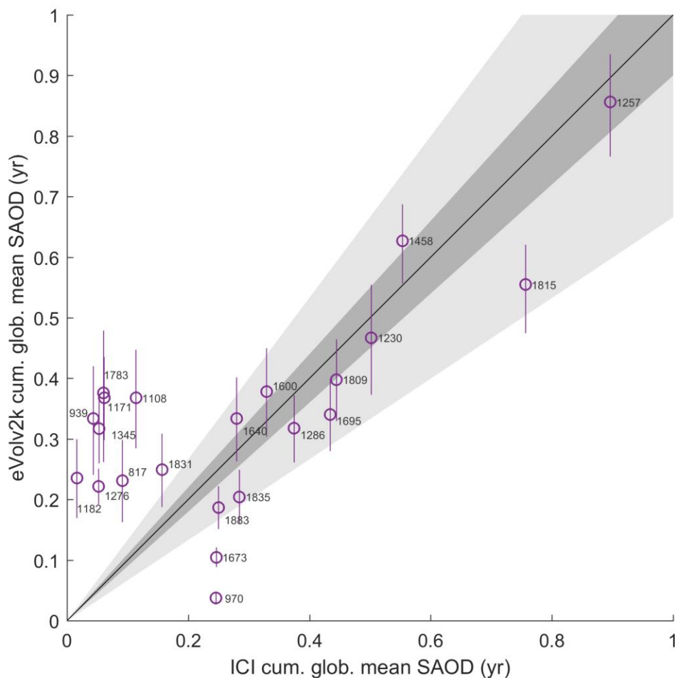
Figure 6: Scatter plot of matched EVA(2k) versus ICI estimates of 3-year cumulative global mean SAOD, for events with values greater than 0.2. Matches are defined in Table S4. Labels show the eVolv2k date of each event. Vertical bars indicate the 1\sigma uncertainty in the EVA(2k) SAOD estimates. The 1:1 line is shown in black, with dark and light gray shading denoting the \pm 10 and 33 % range around 1:1.
