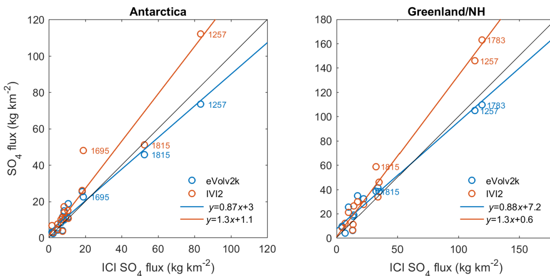
Figure 1: Composite sulphate fluxes derived from ice cores for (left) Antarctica and (right) Greenland (or NH). Values from the eVolv2k (this work) and IVI2 (Gao et al., 2008) reconstructions are plotted vs. composite values from the ICI reconstruction (Crowley and Unterman, 2013), for event matches defined in Table S2. Linear fits to the scatter plots are included, with best fit slopes and intercepts as included in the legends.
