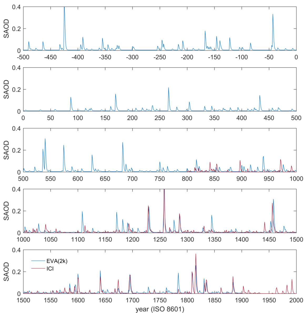
Figure 5: Global mean, annual mean stratospheric aerosol optical depth (SAOD), from the EVA(2k) and ICI reconstructions. Years are shown using the ISO 8601 standard, which includes a year zero.
