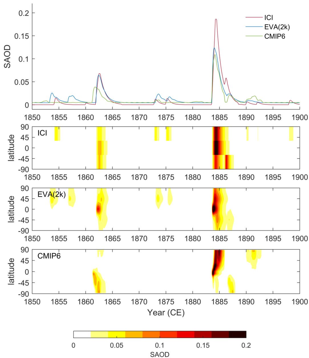
Figure 8: (top) Global mean SAOD from the ICI, EVA(2k) and CMIP6 reconstructions for the 1850-1900 time period of overlap. (bottom) Zonal mean SAOD from the three reconstructions as labelled for the same time period.
