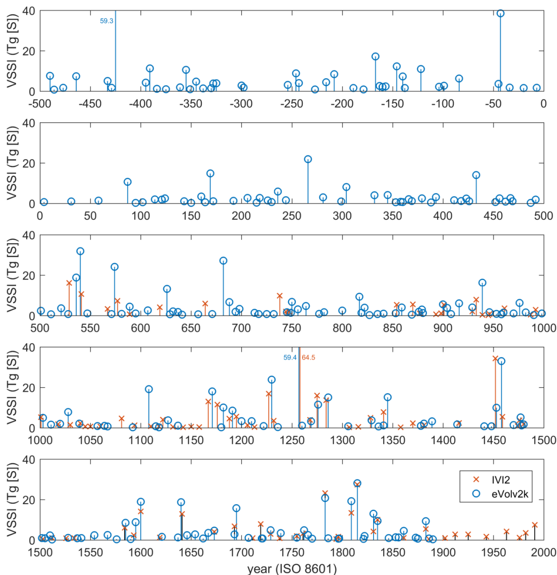
Figure 2: Volcanic stratospheric sulphur injection (VSSI) from the IVI2 and eVolv2k reconstructions. Values exceeding the y-axis limits are denoted as text. Years are shown using the ISO 8601 standard, which includes a year zero.
