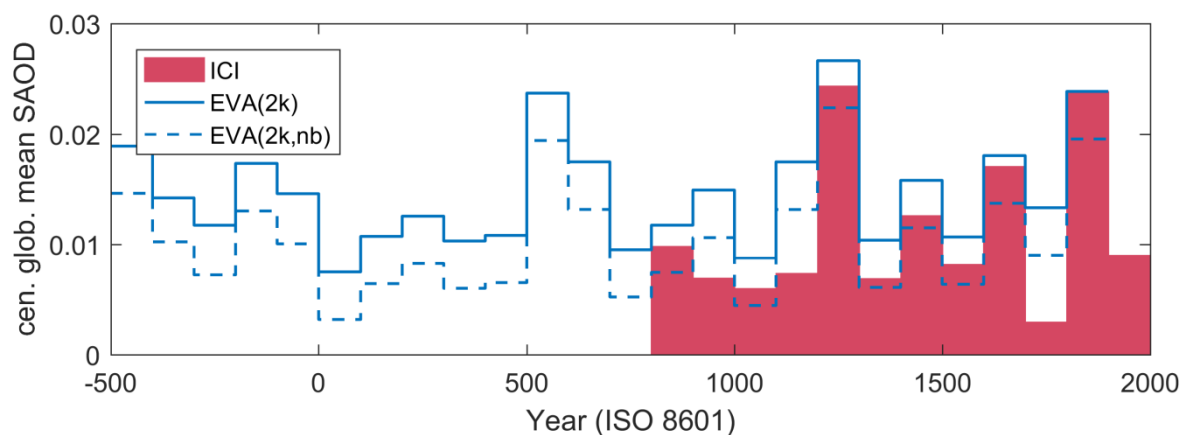
Figure 7: Centennial global mean SAOD from the ICI and EVA(2k) reconstructions. A version of the EVA reconstruction which includes no background sulphur injection, EVA(2k,nb), is shown by the dashed line.
