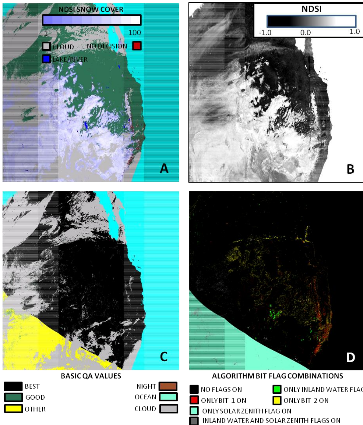
5 Figure 11. VIIRS C1 VNP10 acquired 18 December 2016 at 202 UTC, imaging the western CONUS. Datasets: NDSI_Snow_Cover (A) NDSI (B), Basic QA (C) and a selected combination of the Algorithm_bit_flag QA (D). Unprojected image. The extent of snow cover seen is similar to snow cover extent found on the IMS United States snow cover map ( www.ncdc.noaa.gov/snow-and-ice/snow-cover/us/20161218 ).
