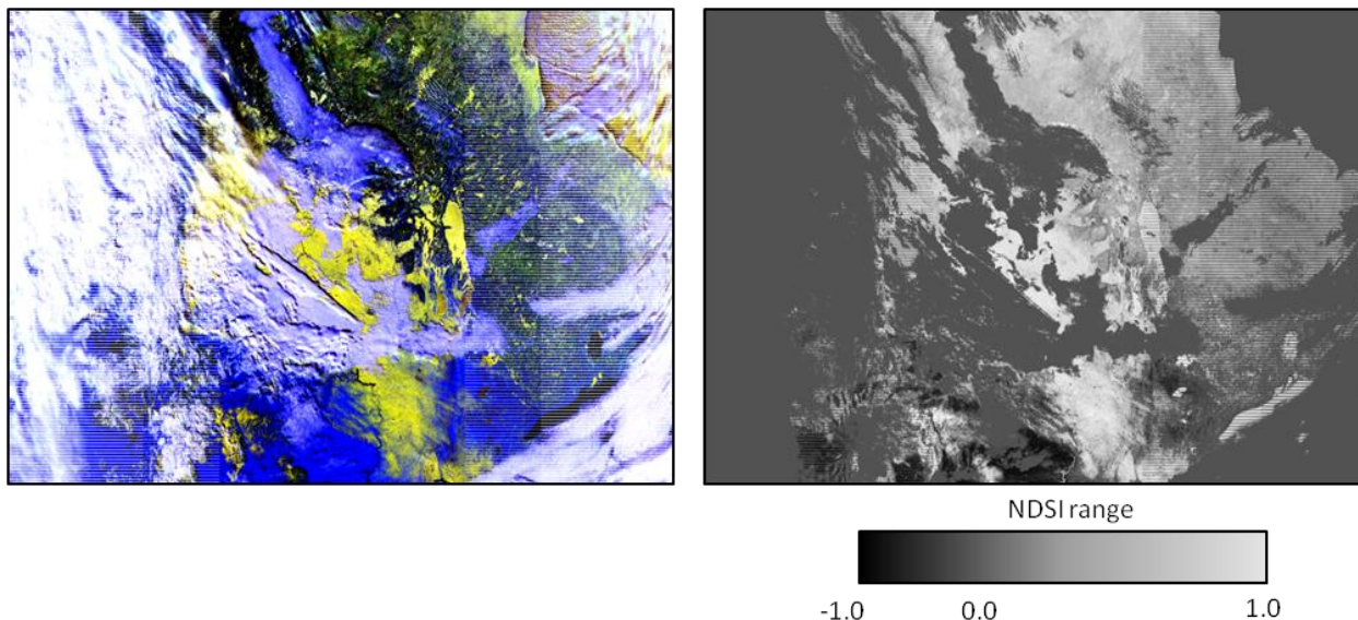
Figure 3. VIIRS NDSI. VIIRS swath of NDSI dataset (right) for 5 December 2014 1945 UTC compared to false color display of bands I1,I2,I3 (left) with snow covered landscape in hues of yellow. NDSI data in range of -1.0 to 1.0, clouds,oceans and night are masked. Swath covers central Canada, Lake Winnipeg is near the center of the swath and Plains of the USA. Note that the striping and the edge of the VIIRS swath is the result of “pixel trimming” resulting in a reduction of the VIIRS “bow-tie” effect in the NASA Level 1 product (Wolfe et al., 2013).
