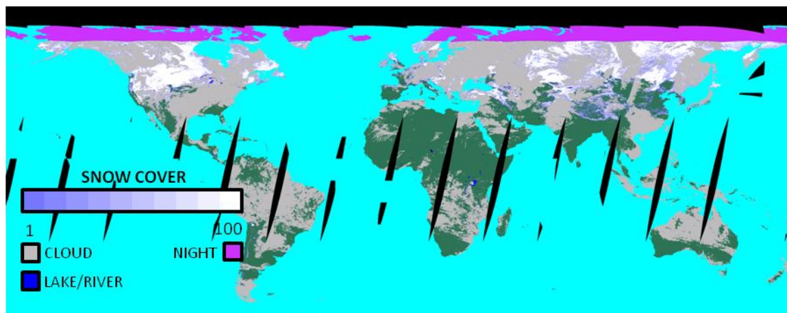
Figure 9. MODIS global snow cover on 14 January 2017. Global snow cover is from MOD10C1.A2017014.006*.hdf. Snow cover is shown with the cloud cover data layer overlaid; the snow cover and cloud cover are in separate data layers in the product.
