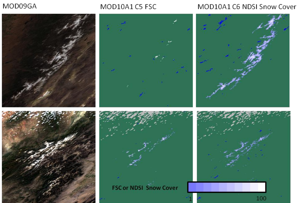
5 Figure 6. Comparison of snow-cover extent between MOD10A1 C5 and MOD10A1 C6. Sierra Nevada range on 15 June 2002, top row, and Upper Rio Grande region on 22 May 2002, bottom row. True color (bands 1, 4, 3) image of the MOD09GA is shown in left column. Significant snow cover extent was missed in C5 FSC however all the snow cover extent is detected in C6 NDSI_Snow_Cover by the revised algorithm.
