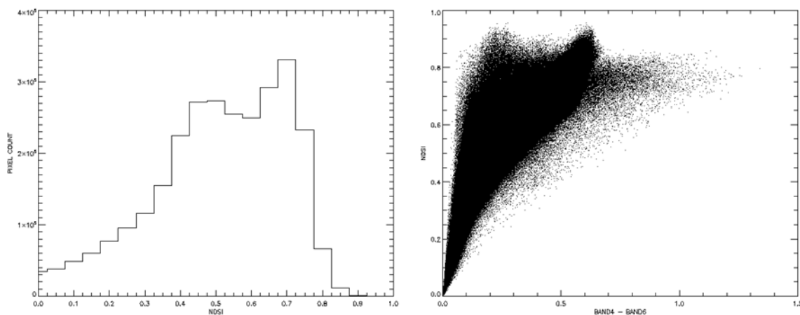
Figure 4. NDSI histogram (left) and scatter plot of NDSI versus VIS-SWIR difference (right) for the MOD10_L2.A2003010.1750.006 image in Fig. 2. Pixels restricted to snow only, i.e. NDSI > 0.0 and not masked as cloud in the NDSI_Snow_Cover dataset. Histogram was calculated with NDSI bin size of 0.05.
