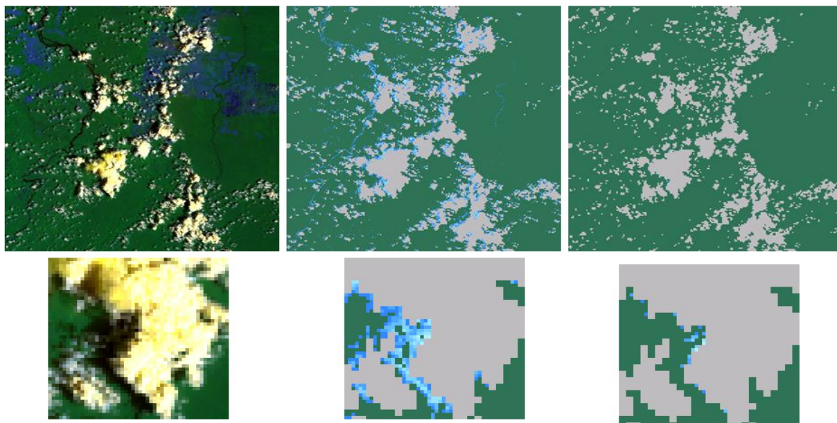
5 Figure 7. Image of southeastern Brazil from VIIRS swath 2014255.1720.PI_03001. False color image of I1, I2, I3 in top left image, zoom of cloud shadow detail in bottom left image. VIIRS NDSI snow cover output without the surface temperature screen in middle images. Top and bottom zoom show the snow commission errors associated with cloud shadowed land and fringes of cloud. VIIRS NDSI snow-cover output with the surface temperature screen applied in right images. Top image and bottom zoom show the effectiveness of alleviating snow commission errors. A few pixels of snow commission error remain at the fringe of clouds, which have NDSI > 0.0, and are below the surface temperature threshold and are not reversed by other screens.
