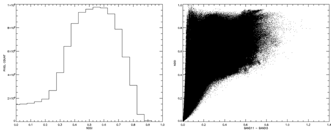
Figure 5. NDSI histogram (left) and scatter plot of NDSI versus VIS-SWIR difference (right) for the VIIRS 5 December 2015, 1945 UTC image in Fig. 3. Pixels restricted to snow only, i.e. NDSI > 0.0 and not masked as cloud in the NDSI_Snow_Cover dataset. Histogram was calculated with NDSI bin size of 0.05.
