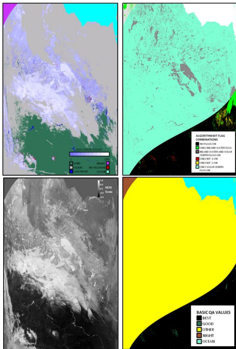
Figure 10. MODIS C6 MOD10_L2.A2003010.1750, imaging the Great Plains and boreal forest in North America. datasets: NDSI_Snow_Cover (upper left) NDSI (lower left), a selected combination of the Algorithm_bit_flag QA is shown in upper right, and the basic QA is shown in lower right.
