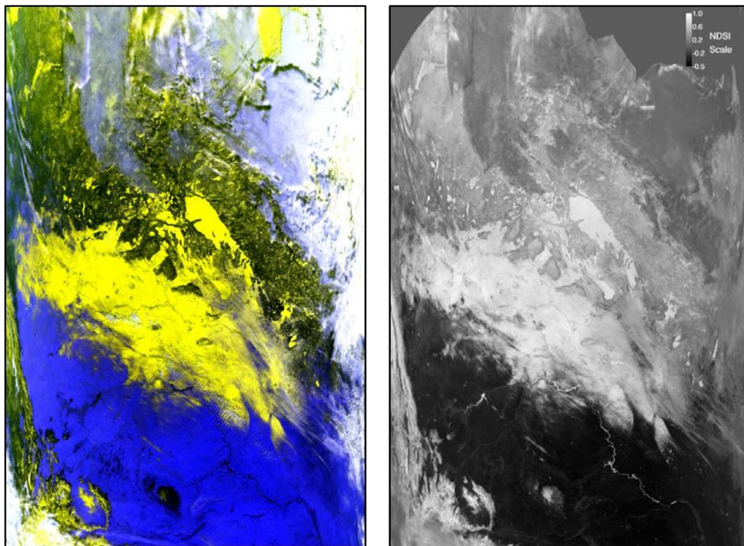
Figure 2. MODIS NDSI. Swath of MOD10_L2 NDSI dataset (right) for 10 January 2003 1750 UTC compared to false color display of MOD02HKM bands 1,4,6 (left) with snow covered landscape in hues of yellow. NDSI data in range of -1.0 to 1.0, clouds are not masked, while oceans and night are masked. Swath covers central Canada, Lake Winnipeg near center of image, and Plains of the USA. Snow covered forest, snow covered plains and snow free plains are seen in this swath.
