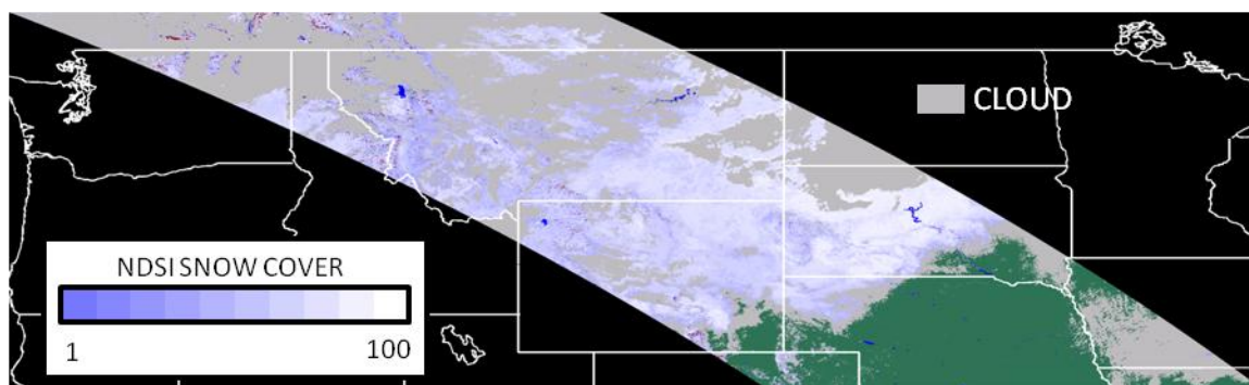
10 Figure 8. Snow cover MOD10A1.A2016366.h10v04.006.*.hdf. Snow cover across the Plains and Rockies on 31 December 2016. The tile has been projected to geographic grid.
