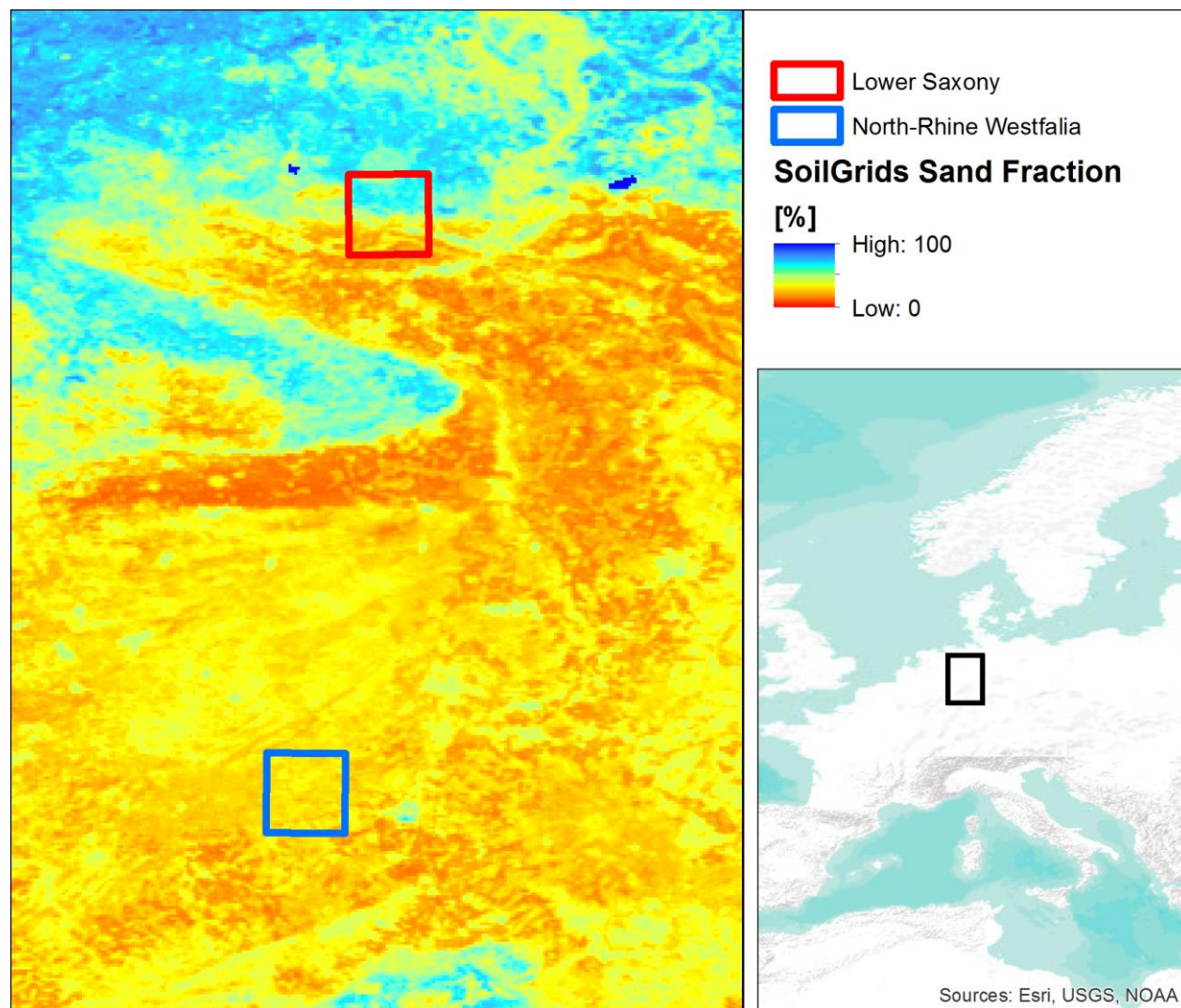
Figure 2: Location of the 0.25° test pixels in Germany, and their sand fraction based on SoilGrids1km.
