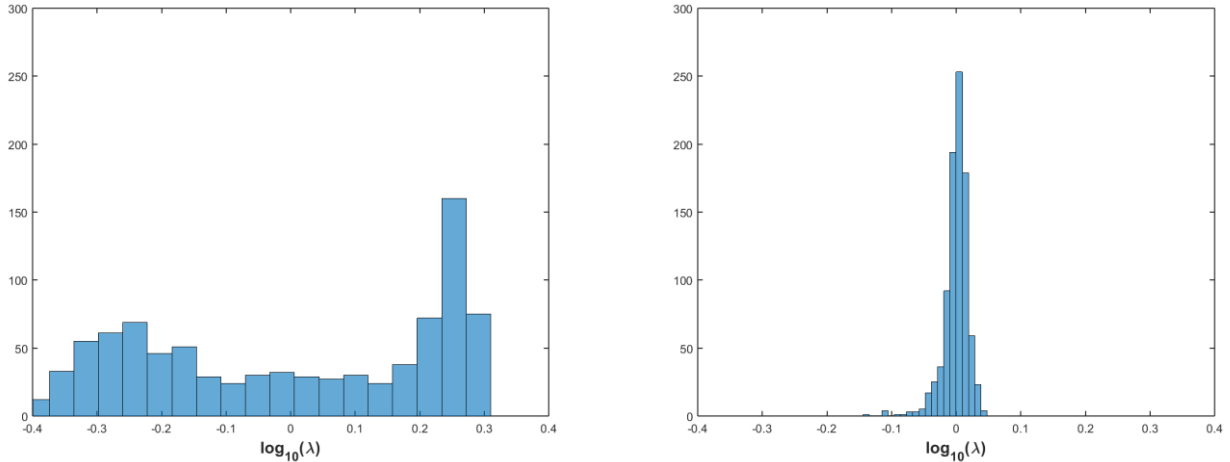
Figure 10: Histograms of the retention scaling parameter ( \log_{10} \hat{\lambda}_i ) for Lower Saxony (left) and North-Rhine Westfalia (right).
