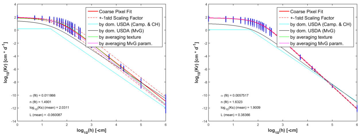
10 Figure 9: Hydraulic conductivity curves for Lower Saxony (left) and North-Rhine Westfalia (right). The coarse pixel fit is the result of the Miller-Miller scaling approach, where also (\log_{10} \hat{\lambda}_i) was estimated. Therefore, also \pm 1\text{std}(\log_{10} \hat{\lambda}_i) could be provided to identify the sub-grid uncertainty. Further hydraulic conductivity curves were calculated by dominant USDA class (both for Brooks & Corey with Clapp & Hornberger and for MvG equation), by averaging texture and by averaging MvG parameters. Blue points indicate \log_{10}(K_r) at standard hydraulic heads for each individual subpixel.
