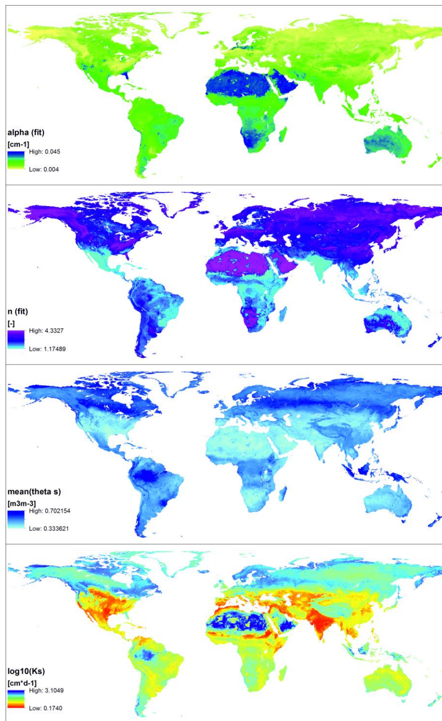
Figure 5: Global map of \hat{\alpha} (top), \hat{n} (top middle), \overline{\theta}_s (bottom middle) and \text{mean}(\log_{10}(K_s)) (bottom) as derived when using the SoilGrids1km data set as input to the Rosetta PTF (Schaap et al., 2001), at 0.25° spatial resolution.
