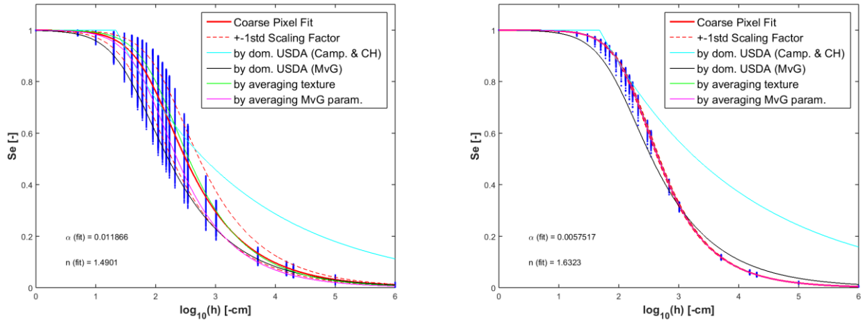
5 Figure 8: Retention curves for Lower Saxony (left) and North-Rhine Westfalia (right) calculated using different approaches. The coarse pixel fit is the result of the Miller-Miller scaling approach, where also (\log_{10} \hat{\lambda}_i) was estimated. Therefore, also \pm 1\text{std}(\log_{10} \hat{\lambda}_i) could be provided to identify the sub-grid uncertainty. Further retention curves were calculated by dominant USDA class (both for Brooks & Corey with Clapp & Hornberger and for MvG equation), by averaging texture and by averaging MvG parameters. Blue points indicate S_e at standard hydraulic heads for each individual subpixel.
