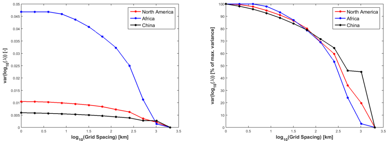
5 Figure 11: Retention scaling parameter variance \text{var}(\log_{10} \hat{\lambda}_i) for different grid resolutions and regions of interest (North America, Africa, and China, see also Figure 4). Left) absolute variance and right) variance normalised as percentage of the maximum variance at 1 km original SoilGrids resolution.
