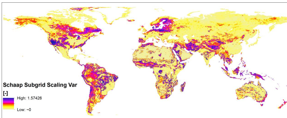
Figure 6: Global map of \text{var}(\log_{10} \hat{\lambda}_i) calculated from SoilGrids1km data set and the Rosetta PTF (Schaap et al., 2001) for 0.25° resolution.
