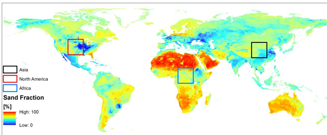
Figure 4: Example regions selected to evaluate the scaling variance loss from Miller-Miller scaling at different spatial resolutions when neglecting the scaling variance. The background shows the sand fraction from SoilGrids1km.
