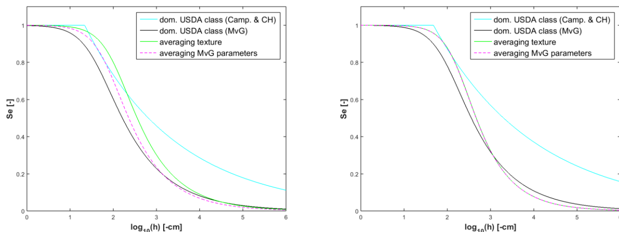
Figure 7: PF curve after applying typical scaling or aggregation methods: by dominant USDA soil class and Clapp & Hornberger parameters for the Brooks & Corey equation, by dominant USDA soil class and MvG equation, by averaging soil texture parameters and then applying ROSETTA PTFs, and by averaging MvG soil hydraulic parameters directly, for Lower Saxony (left) and North Rhine-Westfalia (right).
