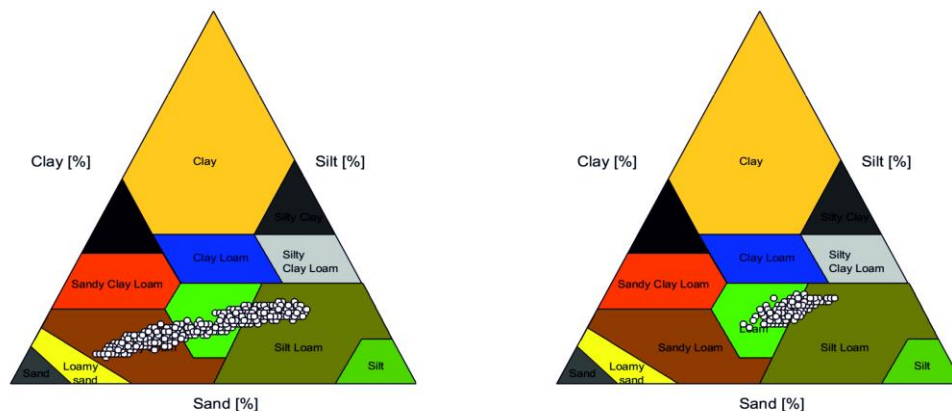
Figure 3: Soil texture triangles, illustrating the difference in soil textural variability of the Lower Saxony pixel (left) and the North-Rhine Westfalia pixel (right), according to USDA classification.
