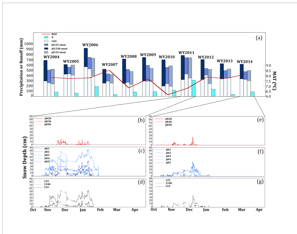
Figure 3: (a) Cumulative annual precipitation from sites 125, 124b, and 125 and cumulative runoff (q) as measured at the JD outlet and mean annual temperature (MAT) based on stations 124 and 125 which are collecting data over the entire 11 WY. That the three precipitation sites are similar in WYs 2005 & 2011 suggests warmer, less windy conditions. Streamflow (q) is specific discharge, or total volumetric stream flow (Q) normalized by catchment area. (b–g) Snow depth in the JD for WY2011 (b–d) and WY2014 (e–g). Panels (b) and (e) show snow depth from sites on the south-facing slopes in red colors, (c) and (f) show snow depth on the north-facing slopes in blue colors, and (d) and (g) show snow depth from 125, 124b, and 124 in grayscale. Each legend shows sites ordered from lowest to highest elevations with brighter tones at lower elevations. Snow depths increase inconsistently with increasing elevations due to wind scour from exposed sites and accumulation in sheltered areas. Gaps due to instrument failure are seen as breaks in the continuous time series line in some subplots.
