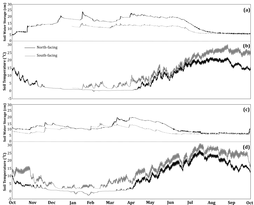
Figure 4. Soil water storage (panels (a) and (c)) and ground temperatures at 20cm (panels (b) and (d)) on both north- and south-facing slopes, up to depths of 100 and 50 cm, respectively, in WY 2011 (a-b) and 2014 (c-d). The legend in (b) applies to all panels. Water storage and temperatures for north-facing slopes were calculated based on jdt1, jdt2, jdt3, and jdt4, and for south-facing slopes, these values were calculated based on jdt2b, jdt3b, and jdt4b. During October - January of WY2011 (panel a), no soil temperature or moisture data on the south-facing slopes were collected due to the soil moisture sensors not yet being installed.
