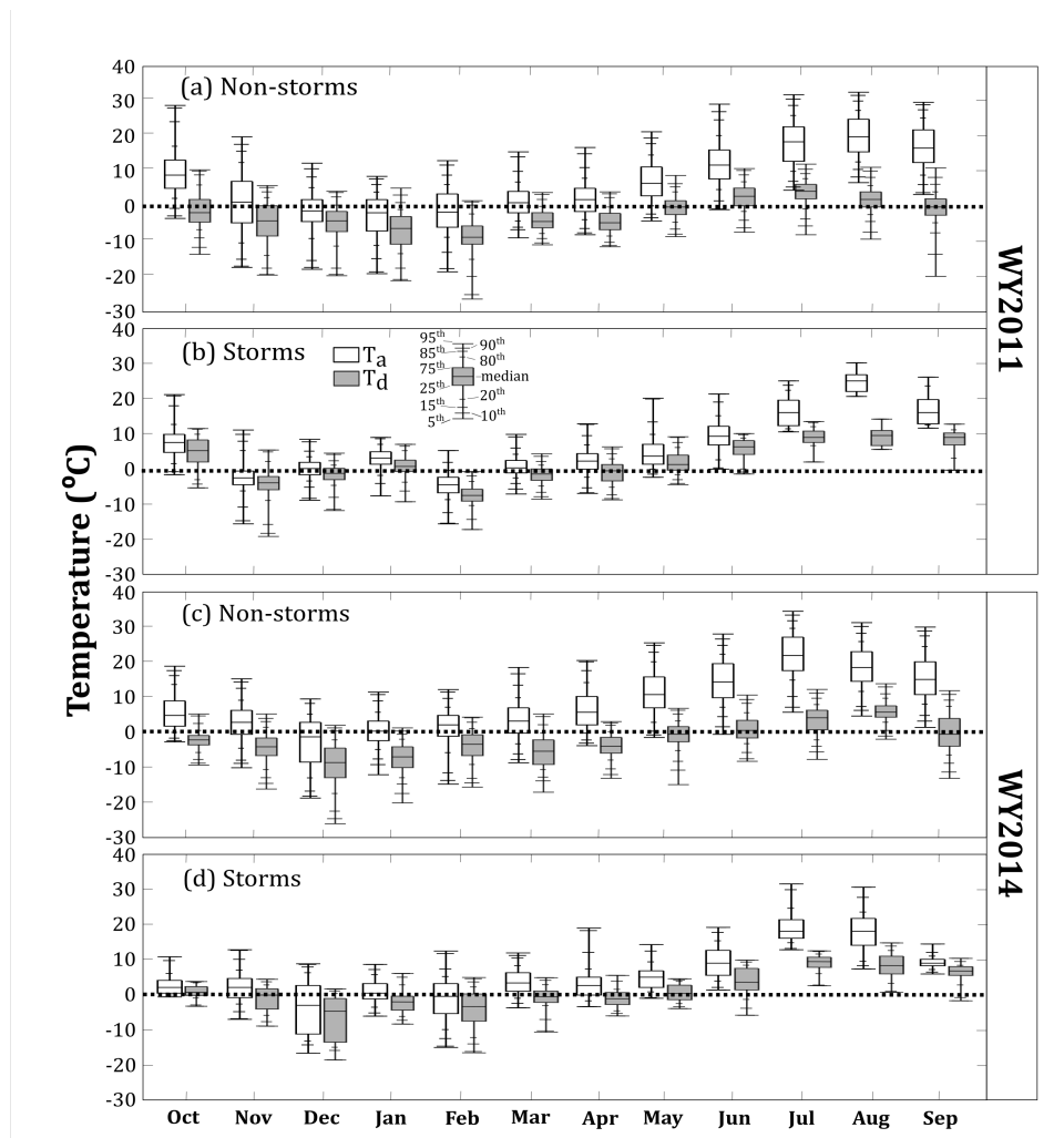
Figure 2: Monthly average T_a (white) and T_d (grey) during non-storm (a and c) and storm (b and d) periods for WY2011 and WY2014 based on data from all stations. The legend in (b) applies to all panels; boxes depict the interquartile range and whiskers indicate the 5 th and 95 th percentiles of data.
