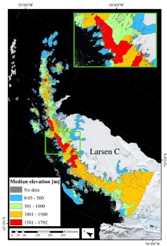
Supplement 1. Color-coded glacier areas for visualization of the median elevation for 1541 glaciers.
