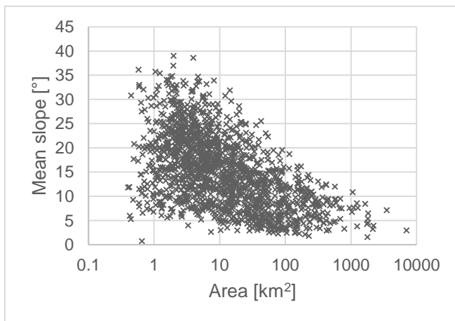
5 Supplement 2. Mean glacier slope vs. glacier area of 1541 glaciers.
