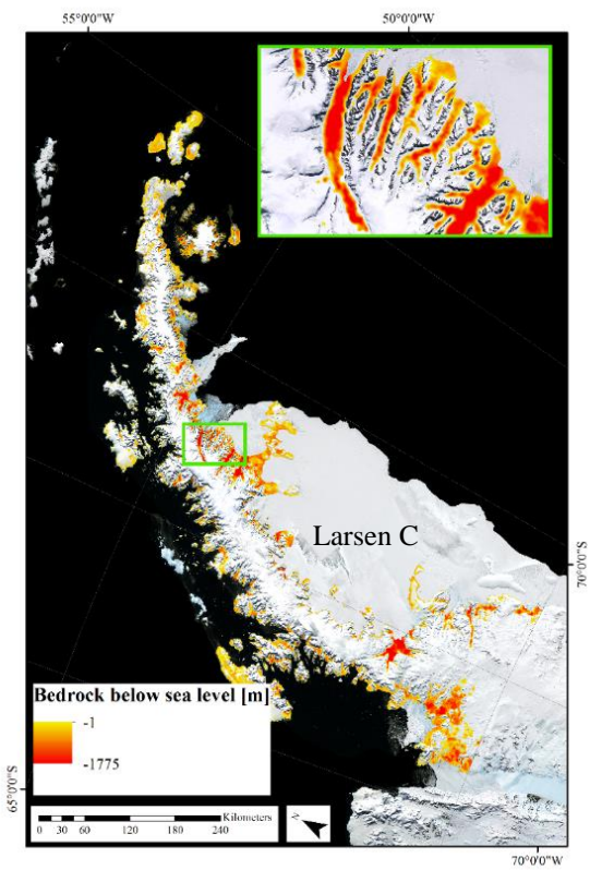
Supplement 4. Negative elevation values representing the bedrock below sea level.
