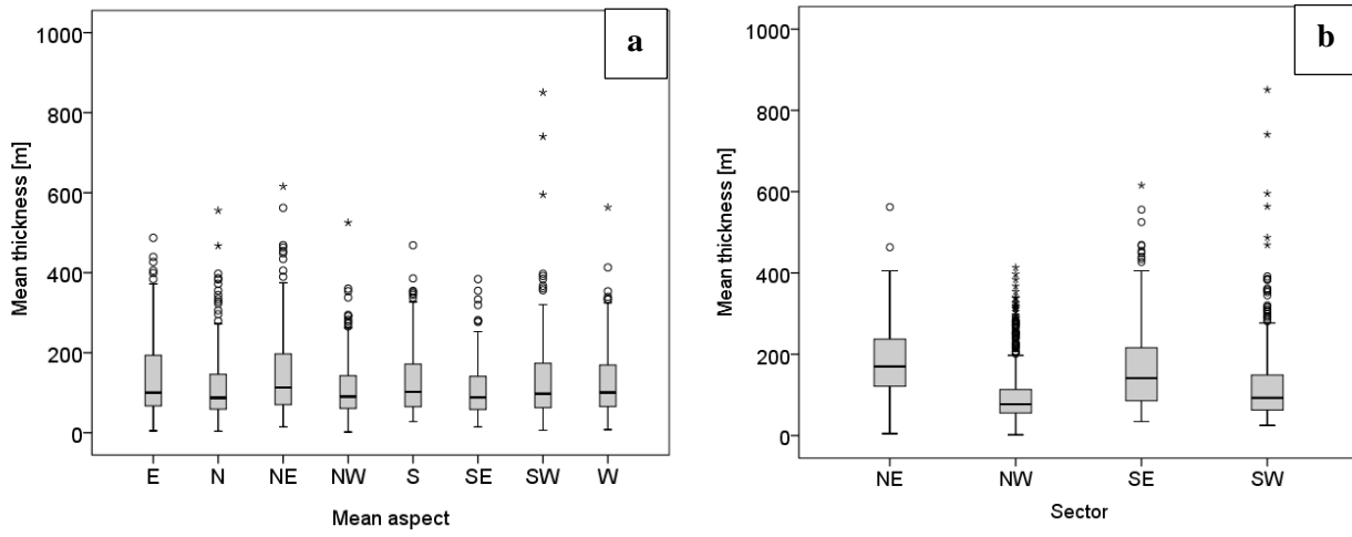
Supplement 3. Boxplots of a) mean thickness per mean aspect and b) mean thickness per sector of the 1539 glaciers including thickness information.
