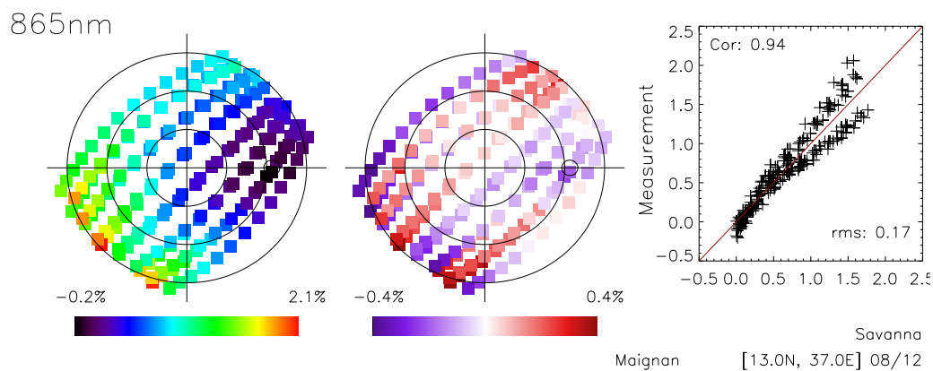
Figure 4: An example of the “ Target BPDF ” window contents. The presentation is similar as for Figure 2 , but only the polarized reflectance at 865 nm is shown.
