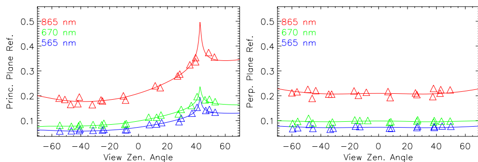
Figure 3: An example of the Principal plane (left) and perpendicular plane (right) window contents. The measurements are shown as triangles and the model prediction is indicated as a line. Three channels are shown which can be selected among 6. The Y-scale can be either linear or logarithmic depending on the MCW setting ( Figure 1 ).
