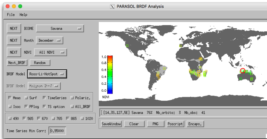
Figure 5: Main Command Window (MCW) when the yearly database is used as input. There are additional options (from the MCW of Figure 1) to display time series of various parameters
