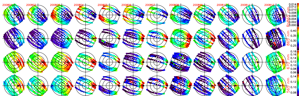
Figure 8: An example of the content of the “All BRDF/BPDF” window. This window shows, for a given target, the measurements for all 12 months in the database. The top line is the BPDF at 865nm while the other three lines are for the reflectances for the three selected bands among 6.
