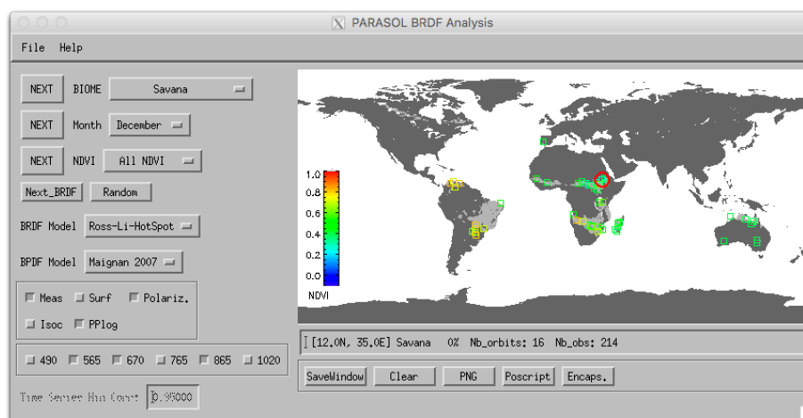
10 Figure 1: Main Command Window (MCW) of the visu_BRDF analysis tool. Various buttons and drop-down menus permit the selection of a given target and various display options as described in the text.
