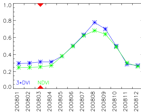
Figure 6: An example of the NDVI window content. It shows the time series of the NDVI and the DVI. The red triangles indicate the month that is displayed on other windows (Figures 2-4).
