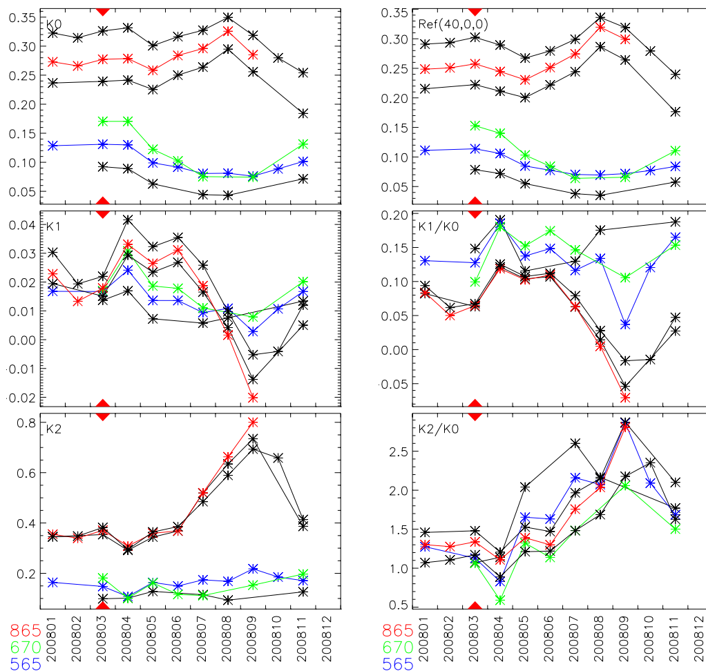
Figure 7: Example of the “Time Series” window content. Depending on a setting of the MCW , this window shows either the monthly time series of the BRDF model parameters (left), or a combination of the same. For the later option, the top figure is the reconstructed reflectance for a reference observation geometry. On these figures, the coloured line/symbols are for the 3 selected bands while the same parameters for the other bands are also shown in black.
