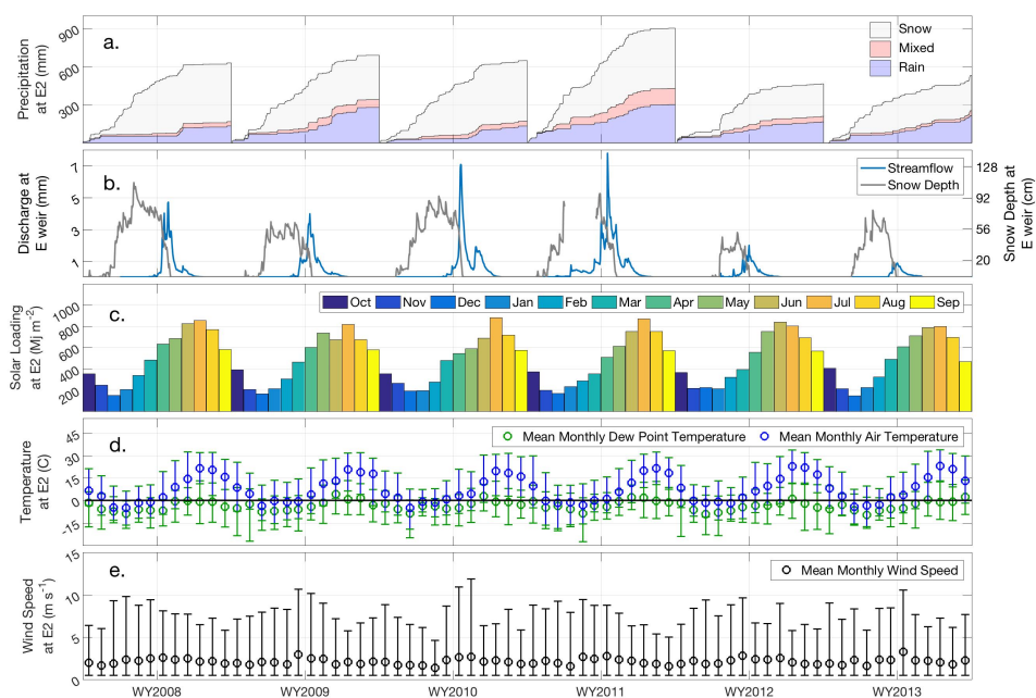
Figure 3. Example forcing data from Catchment E and Weather Station E2 showing a) precipitation amount and phase, b) streamflow, c) monthly incoming solar radiation, d) air and dew point temperature, and e) wind speed.
