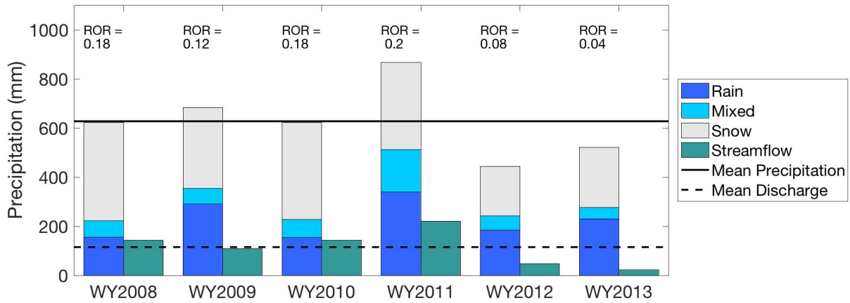
Figure 2. Total water year precipitation split up into phase at the South Mountain Experimental Catchments showing that the precipitation regime is snow dominated. Mean water year water year precipitation was 627 mm as depicted by the solid black line. Mean total catchment streamflow is shown as green bars. The 6-year six-year mean water year stream flow was 115 mm as shown with the dashed black line. Runoff ratios (ROR) are displayed for each water year above the bars.
