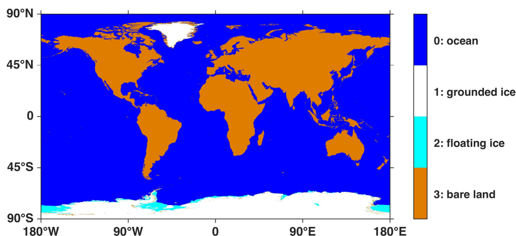
Figure 7. Global surface type mask (compare with Timmermann et al. (2010), Fig. 7 but Greenland ice sheet included).
