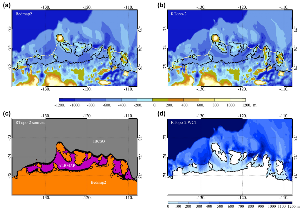
Figure 6. Top line: Bathymetry for Getz Ice Shelf cavity and its surrounding in Bedmap2 (a) and the merged bathymetry in RTopo-2 (b). Panel (c): Indication of data sources for the RTopo-2 bathymetry grid, with colors corresponding to the global source map in Fig. 2. Panel (d): Water column thickness obtained from RTopo-2 ice shelf draft and bathymetry.
