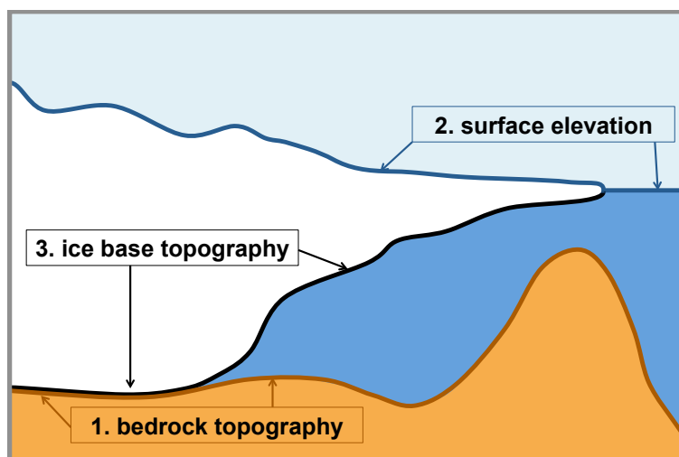
Figure 1. Sketch of a 2D vertical section along a floating glacier tongue/ice shelf with grounded and floating ice (white), sub-ice bedrock/ocean seafloor (brown), water in a subglacial cavity and the open ocean (blue). Lines indicate the bedrock topography (brown), the surface elevation (dark blue), and the ice base topography (black).
