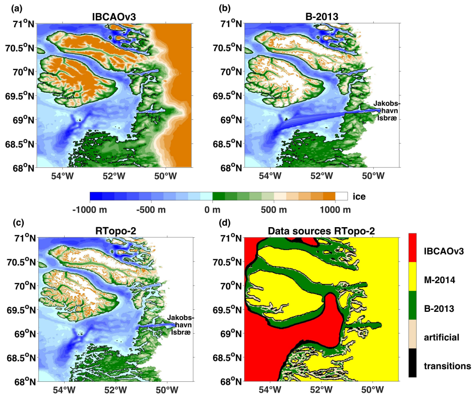
Figure 3. Coastal and shelf region in the west of Greenland including Jakobshavn Isbræ. Maps show the ocean bathymetry/surface elevation in IBCAOv3 (a), ocean bathymetry/bedrock elevation in B-2013 (b), ocean bathymetry/bedrock elevation in RTopo-2 (c) and the data sources for RTopo-2 (d). The color scale is identical for all bathymetry maps. White shading indicates grounded ice and floating ice tongues; black lines mark the coastline. The color flags of the different data sources are identical to Fig. 2.
