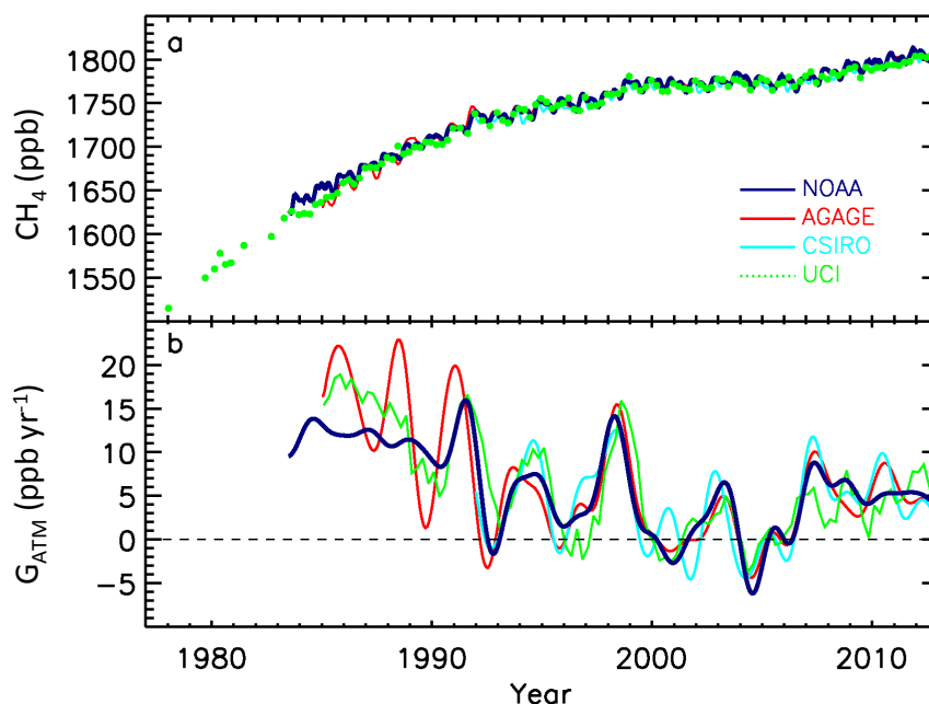
Fig. 1. Globally averaged atmospheric CH 4 (ppb) (a) and its annual growth rate G ATM (ppb yr -1 ) (b) from four measurement programs, National Oceanic and Atmospheric Administration (NOAA), Advanced Global Atmos
