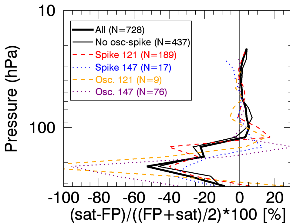
Figure A3: Comparison between Aura MLS WV and frostpoint hygrometer sounding data, (similar to Fig. 3), separated by category of UTLS oscillation in the MLS data.
