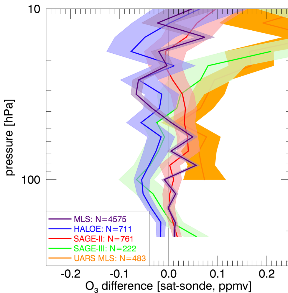
Figure 4: The difference as a function of height between matched satellite and ozonesondes observations. The number of matches at 82 hPa is shown in the legend, and the mean difference (solid) and \pm 2 standard error ( 2\sigma/\sqrt{N} ) range (shaded) are shown at each level.
