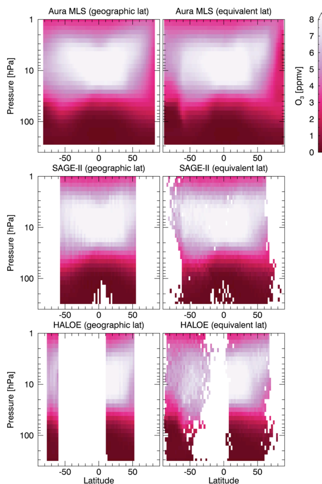
Figure 10: Ozone height vs. latitude plots on geographic latitude (left column) and equivalent latitude grids (right column), for October 2004. Increased data coverage and increased depth of Antarctic ozone depletion is apparent in the equivalent latitude gridded data.
