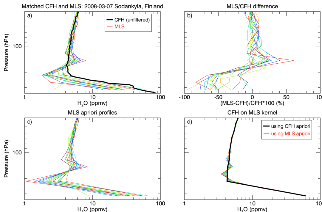
5 Figure A1: (a) Cryogenic Frostpoint Hygrometer H 2 O profile (black) taken from Sodankyla, Finland (67°N) on 2008-03-07, along with the 15 closest matched Aura Microwave Limb Sounder H 2 O profiles (colored). (b) The difference between the matched MLS profiles and the CFH data. (c) The MLS a priori profiles corresponding to the MLS H 2 O retrieval values shown in the upper left panel. (d) The CFH data averaged to the MLS resolution using different a priori profiles as input to the procedure described by Read et al. (2007). The black line is based on the CFH as the a priori, whereas the colored lines are the result of using the corresponding colored line from the lower left panel.
