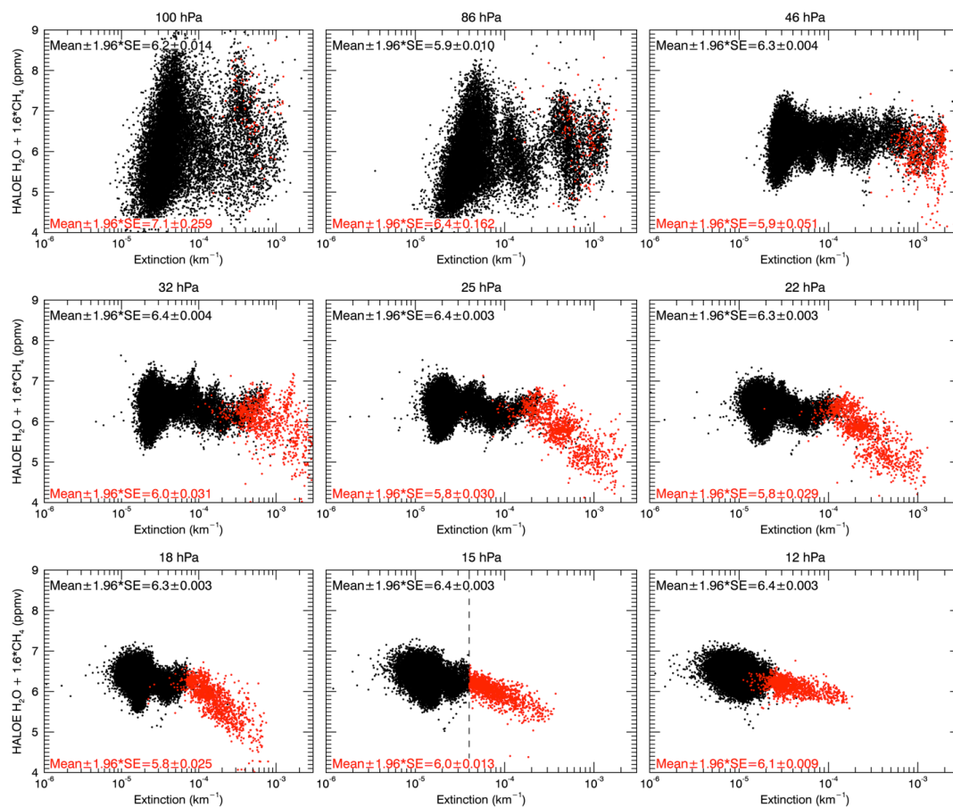
Figure 2: HALOE “total water” ( \text{H}_2\text{O} + 1.6 \cdot \text{CH}_4 ) versus aerosol extinction in the HALOE NO channel for tropical ( 30^\circ\text{S} - 30^\circ\text{N} ) data, segregated by events with low extinction ( < 4 \times 10^{-5} \text{ km}^{-1} , black) and high extinction ( > 4 \times 10^{-5} \text{ km}^{-1} , red) at 15 hPa. The mean \pm 1.96 * standard error of the mean (i.e., the 95% confidence interval) is given for each level and extinction category.
