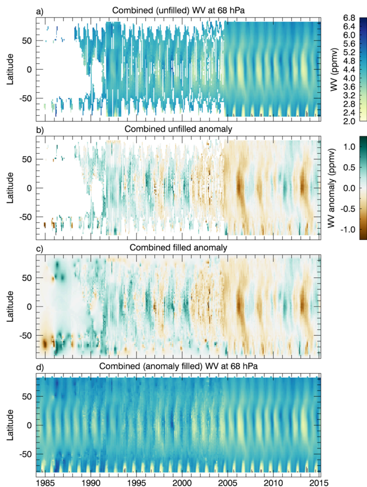
Figure 11: (a) Combined (unfilled) latitude vs. time cross-section of WV at 68 hPa. (b) The anomaly of a), defined as a) minus the seasonal cycle at each latitude. (c) A filled version of b), using radial basis function interpolation. (d) The combined (anomaly filled) product, which is constructed by adding the (latitude dependent) seasonal cycle to the filled anomaly c).
