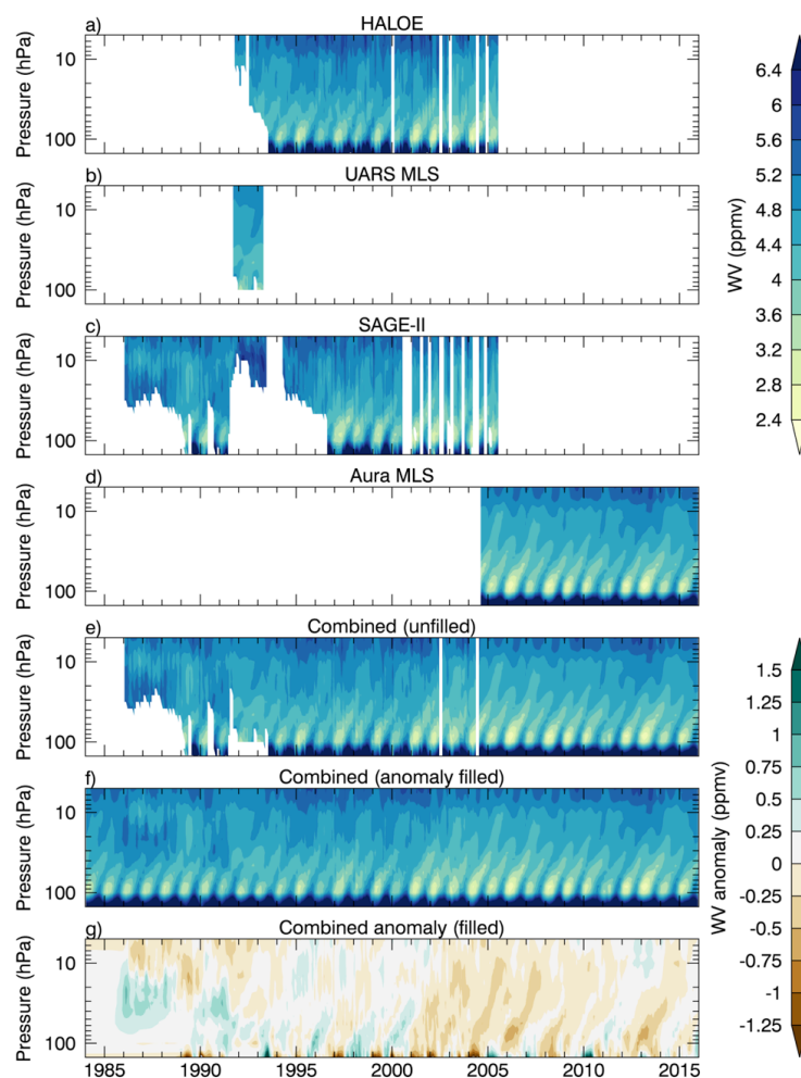
Figure 12: The tropical average ( 30^{\circ}\text{S} - 30^{\circ}\text{N} ) water vapor concentration as a function of height and time, which is commonly referred to as the “tropical tape recorder”, for each satellite data set in SWOOSH (a-d), as well as the two combined products (e-f) and the combined (filled) anomaly product (g). SAGE-III data are nonexistent in the tropics, and therefore not included.
