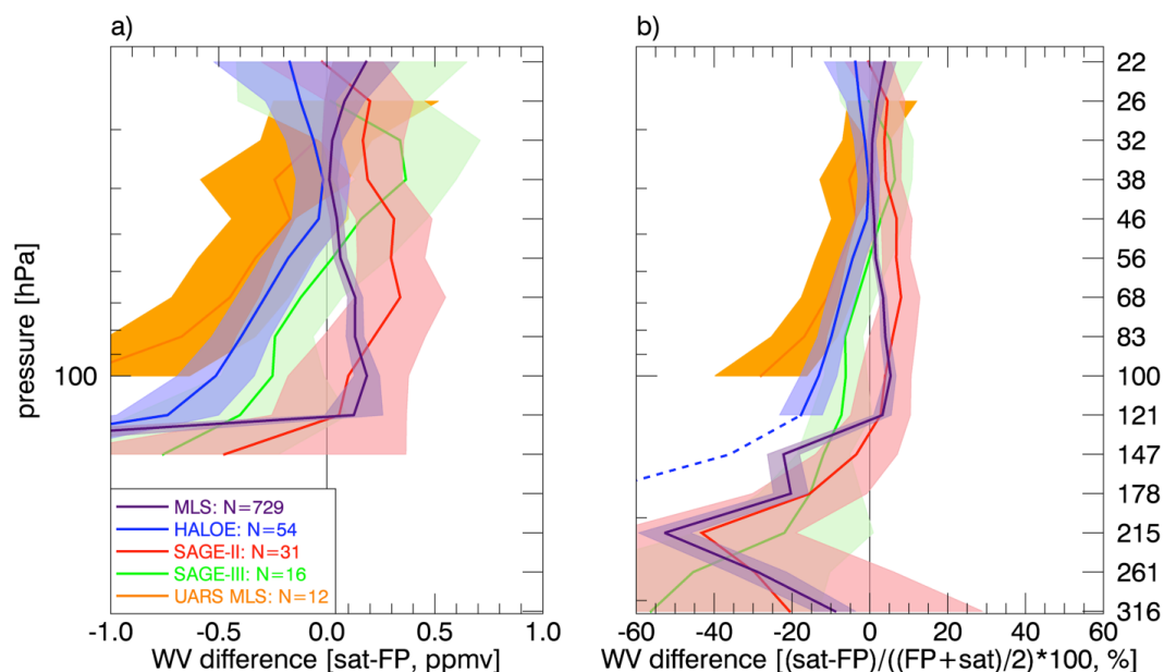
Figure 3: The difference as a function of height between matched satellite and balloon frostpoint hygrometer water vapor data, expressed in (a) as a mixing ratio difference and in (b) as a percent difference between the mean value at each level (see discussion in Sect. 3.1). The number of matches at 82 hPa is shown in the legend, and the mean difference (solid) and \pm 2 standard error ( 2\sigma/\sqrt{N} ) range (shaded) are shown at each level. The dashed blue line shows the HALOE data that are excluded from SWOOSH, at and below 147 hPa.
