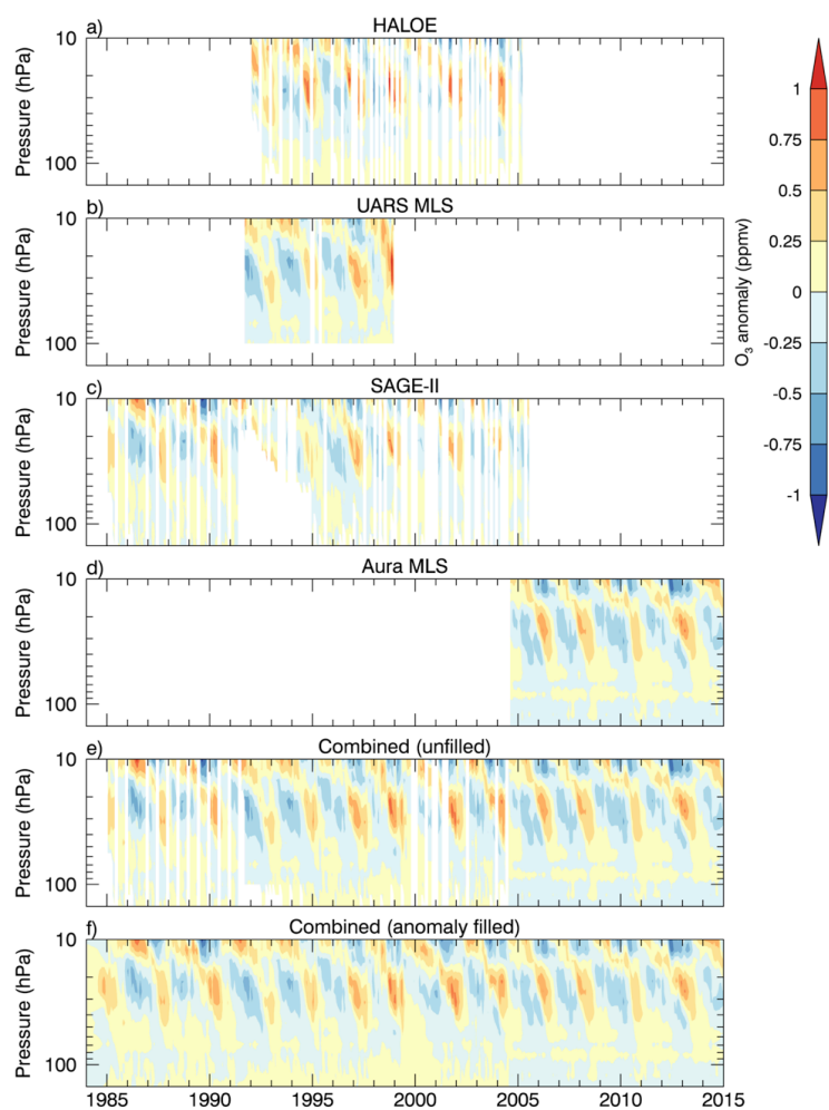
Figure 13: The tropical average (10°S – 10°N) ozone concentration anomaly as a function of height and time for each satellite data set in SWOOSH (a-d), as well as the two combined products (e-f).
