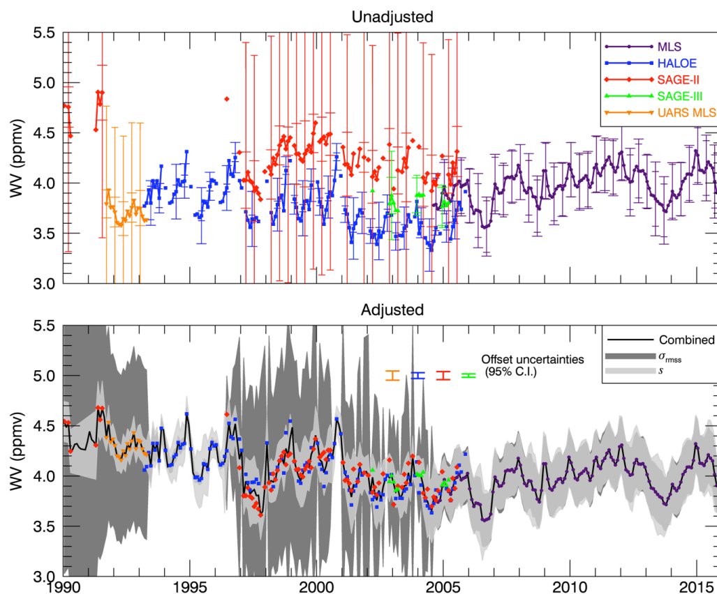
Figure 8: (Top) The uncorrected source water vapor timeseries in the 30° - 40°S latitude band at 68 hPa, along with the source standard deviation (wide error bars) and root-mean-sum-of-squares (RMSS) uncertainty values ( \sigma_{rms} , narrow error bars). (Bottom) The offset-corrected source measurements along with the combined (“anomaly filled”) product. The lighter and darker gray shaded regions show the combined RMSS uncertainty ( \sigma_{rms} , narrow error bars) and the combined standard deviation ( s ), respectively. The vertical errorbars in the lower panel show the 95% confidence interval of the offset uncertainties for the 30° - 40°S latitude band at 68 hPa.
