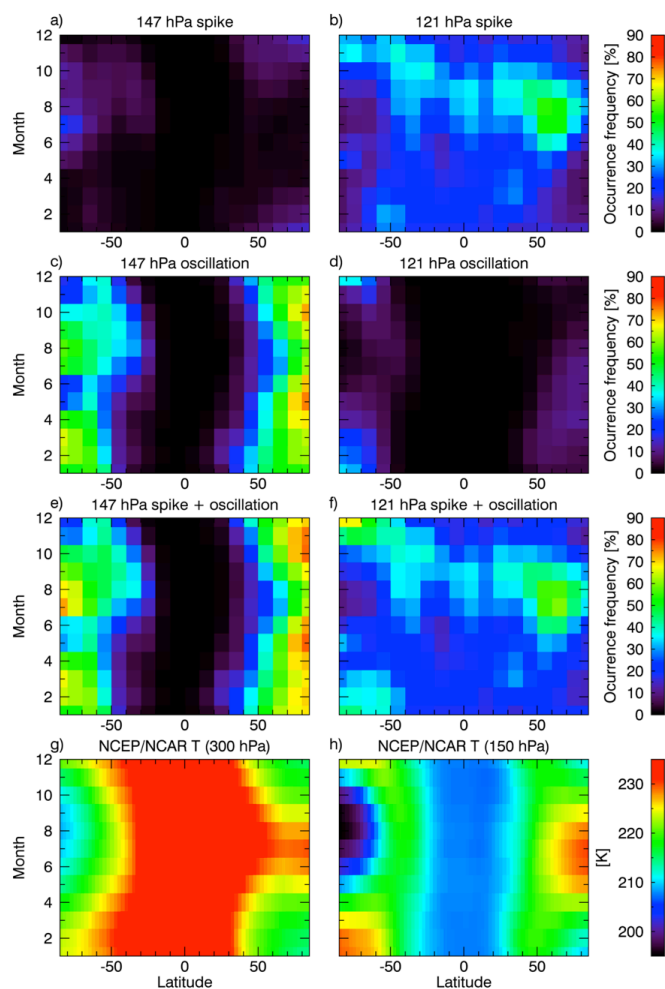
Figure A4: (Top rows) Occurrence frequency statistics for the four types of Aura MLS UTLS WV oscillations identified. (Bottom row) NCEP/NCAR reanalysis 1981-2010 climatological mean zonal-mean temperature at 300 hPa and 150 hPa.
