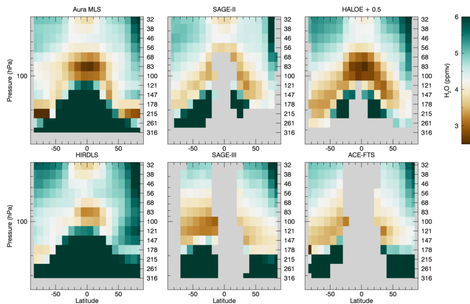
Figure A2: Zonal-mean height vs. latitude cross-section of water vapor from six satellite instruments for the month of March, averaged from 2001 – 2009. Data are gridded on a 10° latitude grid using PV-based equivalent latitude from MERRA.
