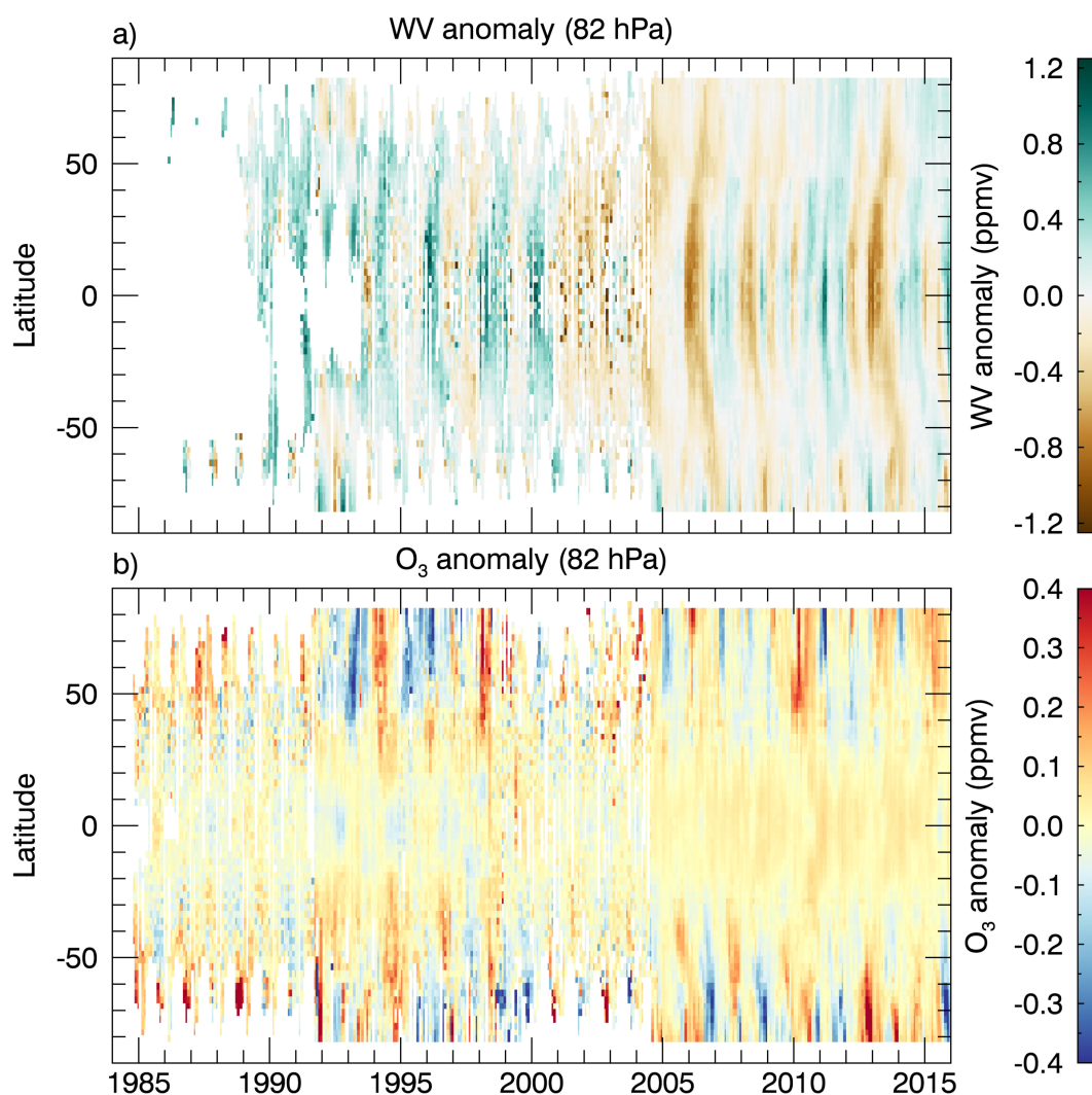
Figure 14: SWOOSH combined product water vapor and ozone anomalies (unfilled) at 82 hPa.
