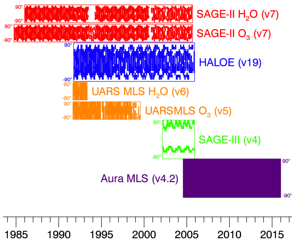
5 Figure 1: Temporal and latitudinal coverage of satellite data used as input to SWOOSH. The boxes surrounding each data set span 90°S – 90°N in the vertical. Data are filled for each month and 10° latitude band containing valid data. Where significant coverage differences exist for WV and O 3 for a given satellite, the coverage is plotted separately.
