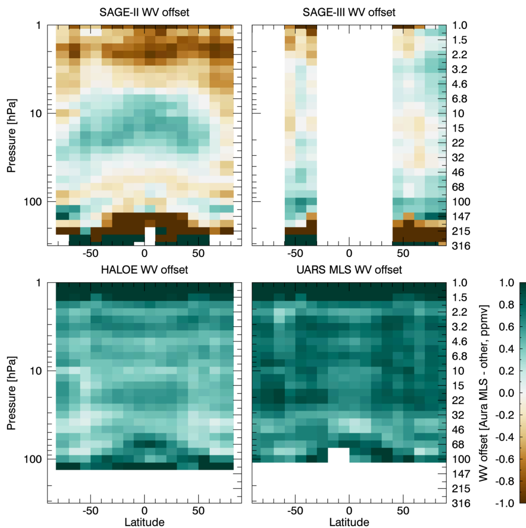
Figure 5: WV offsets relative to Aura MLS for satellite data sets used in SWOOSH. WV offsets are defined as the mean of MLS minus the given dataset. Offsets are computed on the MLS vertical grid in 10° latitude bands.
