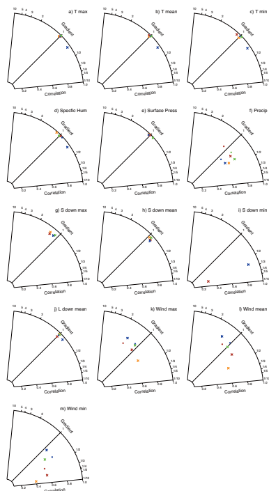
Figure 7. Correlation diagrams for GTMP data and daily site observation data showing Pearson's correlation coefficient and gradient of the fitted line for (a) maximum air temperature, (b) mean air temperature, (c) minimum air temperature, (d) specific humidity, (e) surface pressure, (g) maximum downward shortwave radiation, (h) mean downward shortwave radiation, (i) minimum downward shortwave radiation, (j) downward longwave radiation, (k) maximum wind speed, (l) mean wind speed, and (m) minimum wind speed. Level 0 data are shown as crosses and Lv1 data as dots. Sites are shown by colours, i.e. Fairbanks (orange), Kevo (red), Tiksi (blue), and Yakutsk (green).
