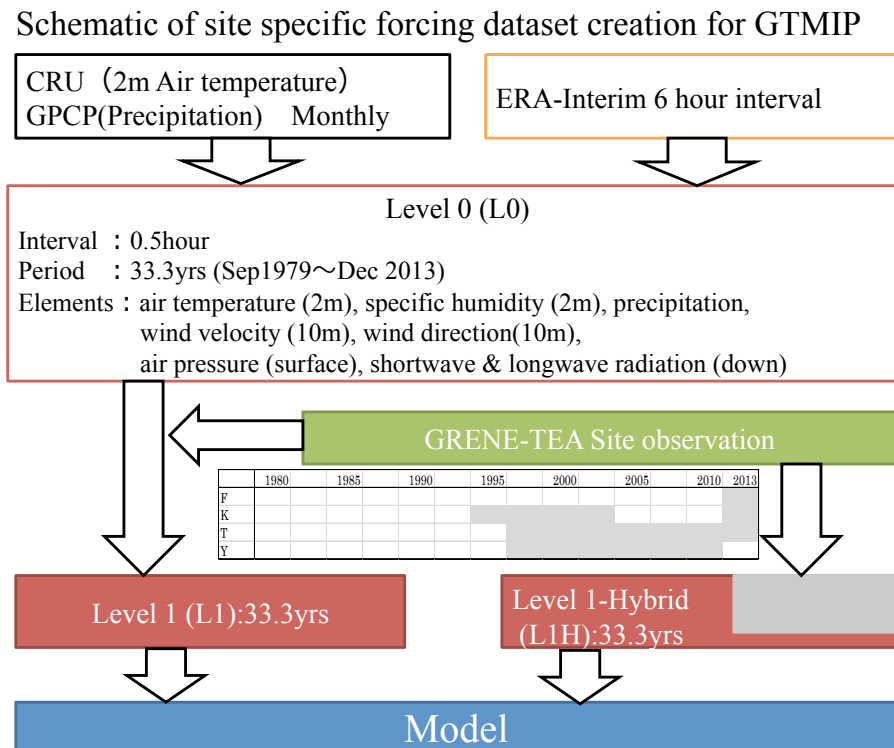
Figure 2. Schematic diagram for data creation during GTMIP stage 1.
