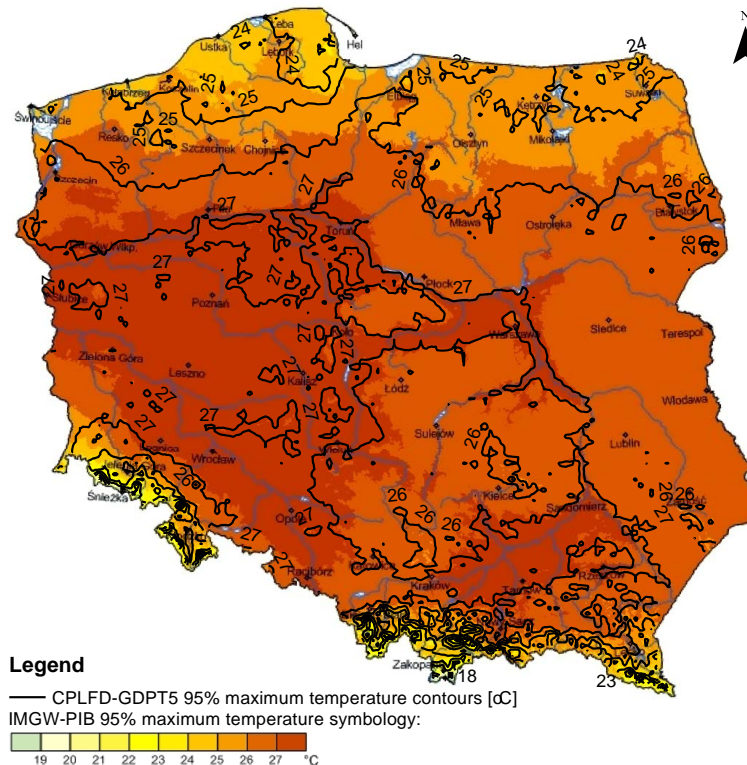
Figure 14. Comparison of CPLFD-GDPT5 95 % maximum temperatures contours with IMGW-PIB 95 % maximum temperatures map for the 1971–2000 period. Contours are in 1 °C intervals. The IMGW-PIB map indicates also major rivers (blue lines) and major cities (labelled black circles). The IMGW-PIB map is adapted from the Climatic Maps of Poland (IMGW-PIB, 2015).
