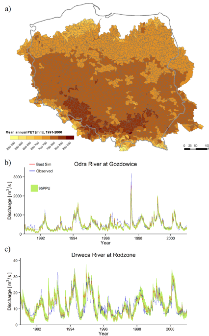
Figure 15. Example application of CPLFD-GDPT5 in the hydrological model SWAT of the Visula and Odra basins. (a) Mean annual potential evapotranspiration calculated using the Hargreaves method based on daily minimum and maximum temperature data. (b) Simulated and observed daily stream flow on the Odra river at Gozdowice gauging station. (c) Simulated and observed daily stream flow on the river Drweca at Rodzone gauging station. Green band denotes 95 percent prediction uncertainty, blue and red lines denote observed and simulated (best solution) flows, respectively.
