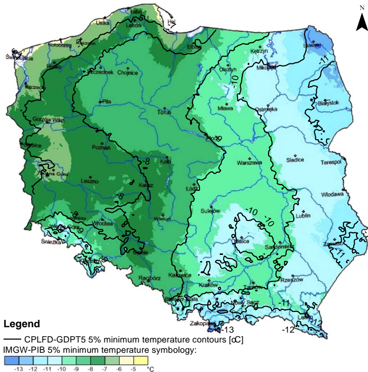
Figure 13. Comparison of CPLFD-GDPT5 5% minimum temperatures contours with IMGW-PIB 5% minimum temperatures map for the 1971–2000 period. Contours are in 1 °C intervals. The IMGW-PIB map indicates also major rivers (blue lines) and major cities (labelled black circles). The IMGW-PIB map is adapted from the Climatic Maps of Poland (IMGW-PIB, 2015).
