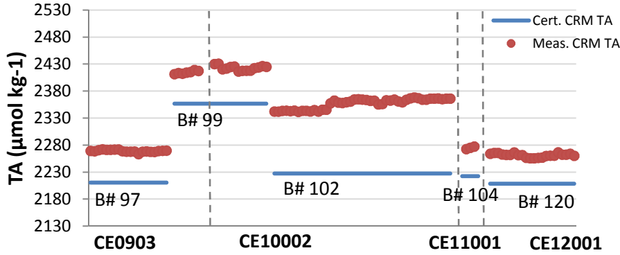
Figure 2 DIC and TA CRM measured values plotted against certified values for each of the surveys. Dashed lines indicate a new survey.
