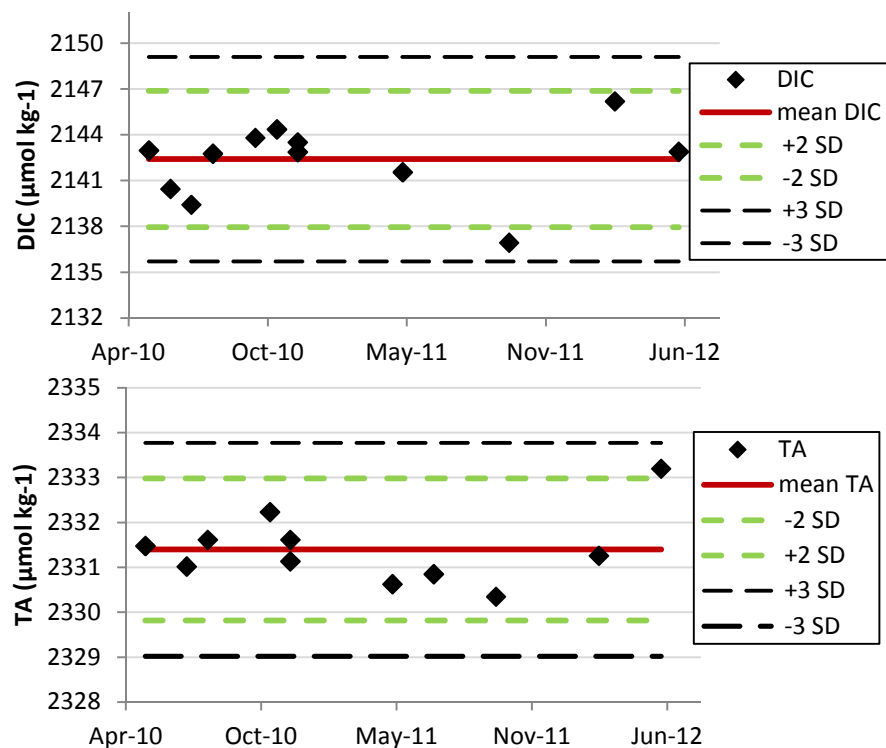
Figure 3 Average monthly (from at least 2 sample bottles) DIC and TA concentrations over 2 years of storage. The mean and standard deviations for DIC were based on the first year of
