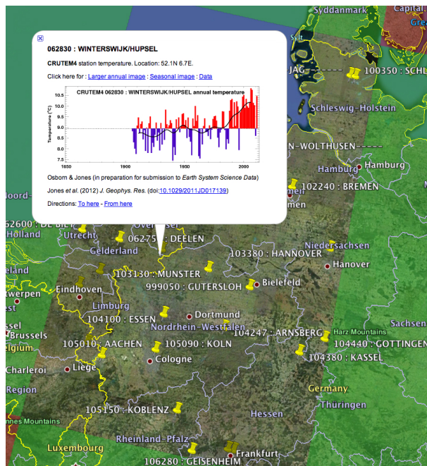
Fig. 5. Image from Google Earth showing the box that appears after clicking on one of the weather station marker pins. The box shows the annual-mean temperature timeseries as bars (blue for values below a reference mean, red for values above; the reference mean is from the 1961–1990 period if there are at least 18 annual values within that period, otherwise it is the overall mean of the data) with a black line for the 20 yr smoothed variations. The box also shows the location of the weather station, its CRUTEM4 identifier (usually the WMO identifier) and name, and provides links to a larger image of the annual timeseries, to an image of the seasonal-mean temperature timeseries, and to a text file containing the monthly, seasonal and annual temperature values for this weather station.
