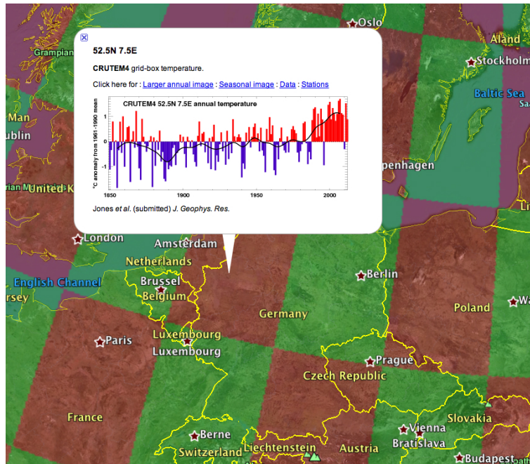
Fig. 3. Image from Google Earth showing a box that appears after clicking on one of the highlighted grid boxes. The box shows the annual-mean temperature anomaly timeseries as bars (blue for values below the 1961–1990 reference period mean, red for values above) with a black line for the 20 yr smoothed variations. The box also shows the location of the centre of the grid box and provides links to a larger image of the annual timeseries, to an image of the seasonal-mean temperature anomaly timeseries, to a text file containing the monthly, seasonal and annual temperature anomaly values for this grid box, and a link to load into Google Earth a KML file for the CRUTEM4 weather stations that lie within this grid box.
