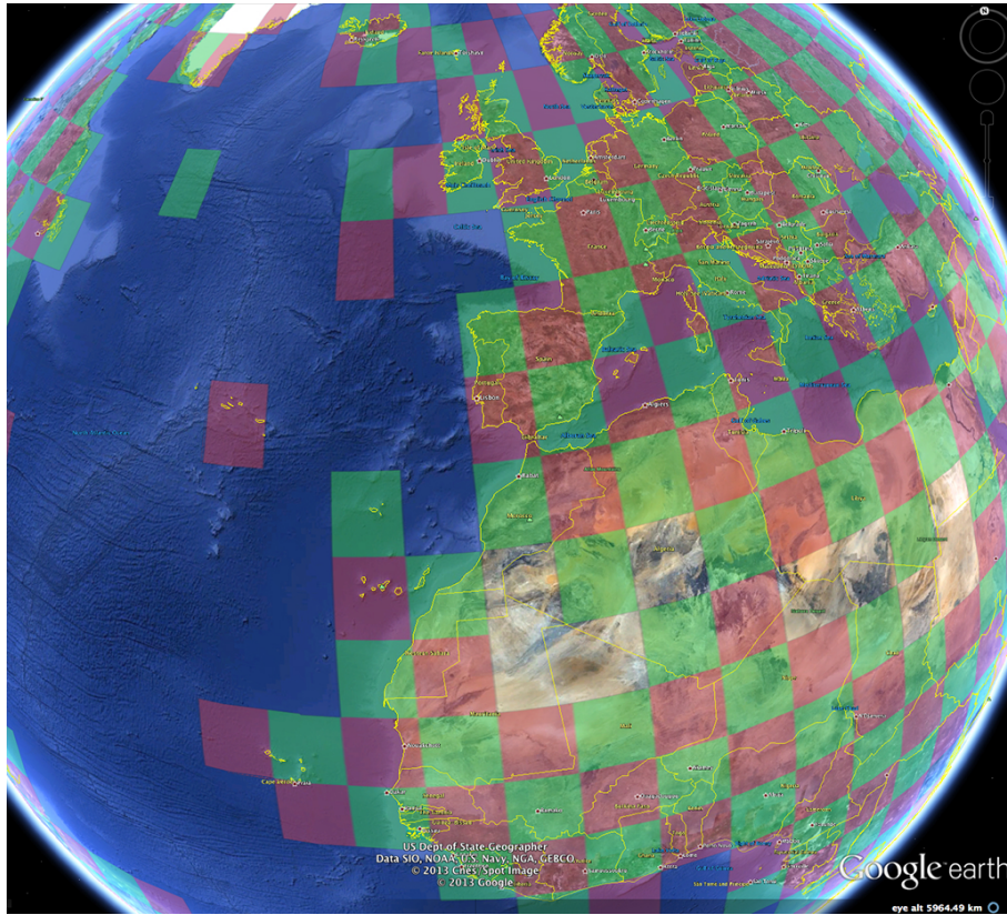
Fig. 2. Image from Google Earth showing the grid boxes that contain some gridded temperature anomaly data in CRUTEM4, highlighted by translucent green and red boxes. Land areas that are not marked by a green or red box do not contain any gridded temperature anomaly data in the CRUTEM4 dataset.
