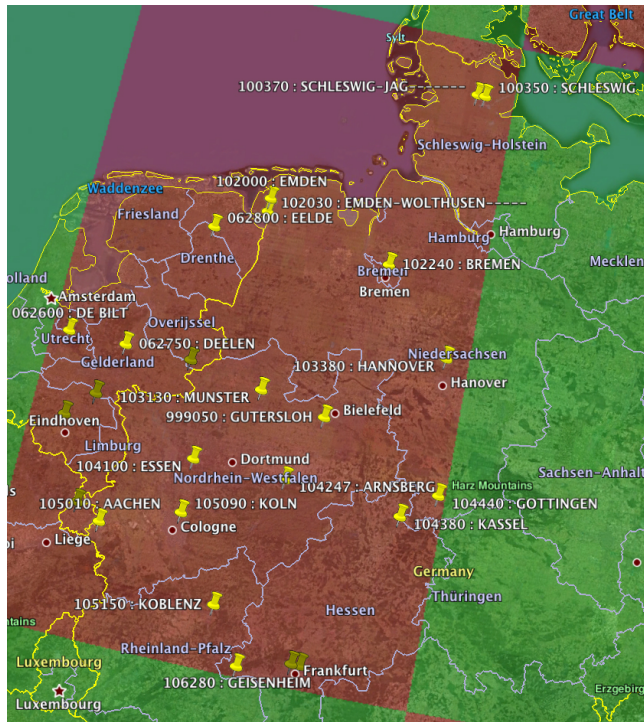
Fig. 4. Image from Google Earth showing the CRUTEM4 weather station locations within a particular grid box (the yellow marker pins). The CRUTEM4 identifier number (ID) and name of each weather station is shown with white text next to each yellow marker pin. The ID is usually the WMO ID, made up of two or three digits to represent the country and the remaining digits to represent the station (in this example, the stations beginning 06 are in the Netherlands, and 10 are in Germany). If the station has not been allocated a WMO ID, or is from a source that has not used the WMO ID system, then it usually begins with 99 (e.g. 999050 Gutersloh in this example).
