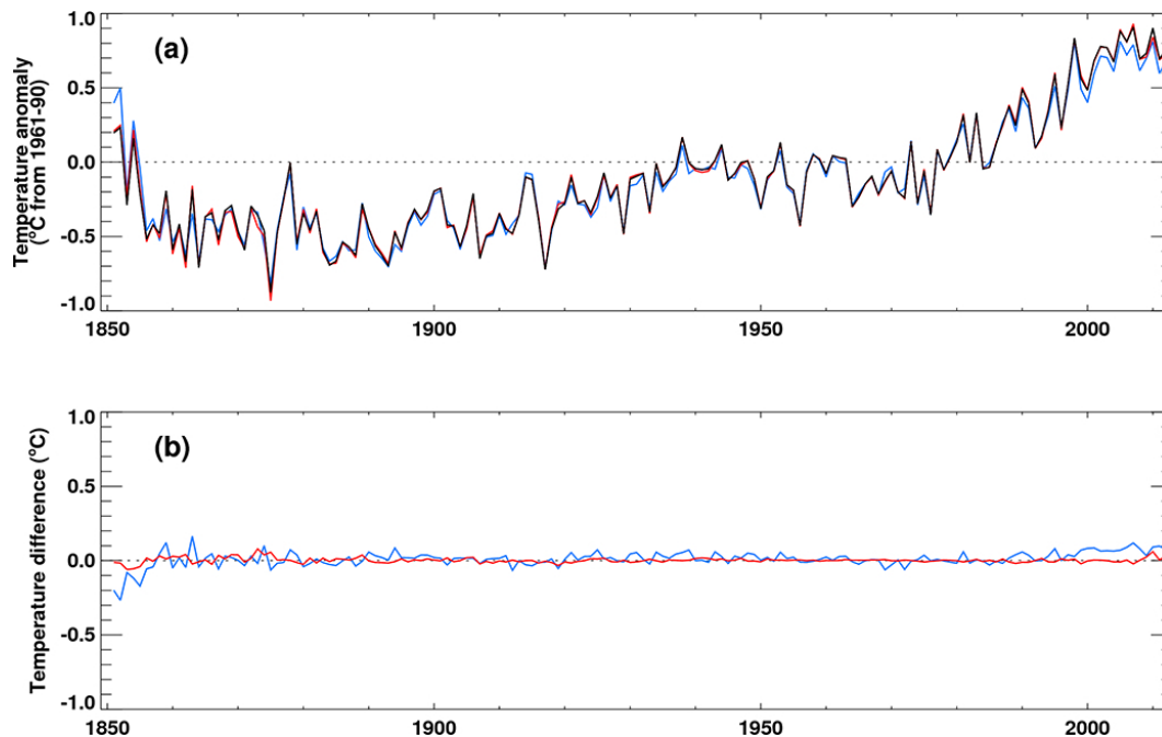
Fig. 1. Annual and global mean land air temperatures anomalies calculated using three approaches: (1) from monthly hemispheric means, then annual means, then global means (Eq. 9) weighted by land area in each hemisphere (black); (2) from annual grid-box means, then hemispheric means, then global means weighted by land area in each hemisphere (red); (3) from hemispheric means, then annual means, then global means of equally-weighted hemispheres. The three results are compared in (a), and differences (red = (1)–(2), blue = (1)–(3)) are shown in (b) with the same vertical scale as in (a).
