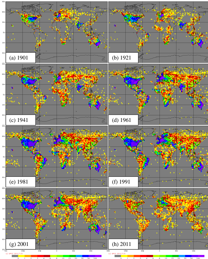
Fig. 7. Spatial distribution of the number of stations per 2.5^{\circ} \times 2.5^{\circ} grid available for the July reanalyses (Version 6) of (a) year 1901 with 10 907 stations, (b) year 1921 with 16 688, (c) year 1941 with 24 602, (d) year 1961 with 41 032, (e) year 1981 with 42 670, (f) year 1991 with 42 511, (g) year 2001 with 36 156, and (h) year 2011 with 9726 stations.
