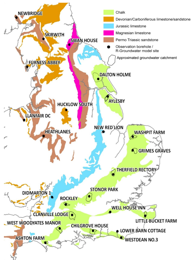
Fig. 2. Future Flows Hydrology R-Groundwater model sites. Copyright © NERC (BGS) 2012. Contains Ordnance Survey data © Crown Copyright and Database Right.
