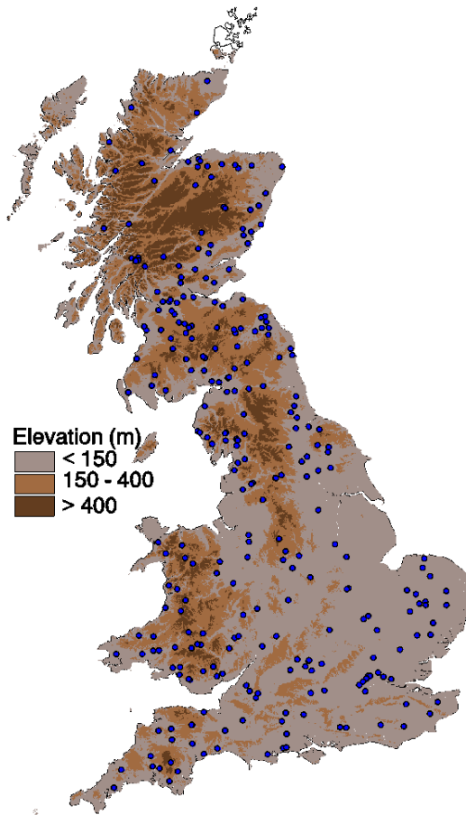
Fig. 1. Catchment river outlets where Future Flows Hydrology time series are generated. Copyright © NERC (CEH) 2012. Contains Ordnance Survey data © Crown Copyright and Database Right.
