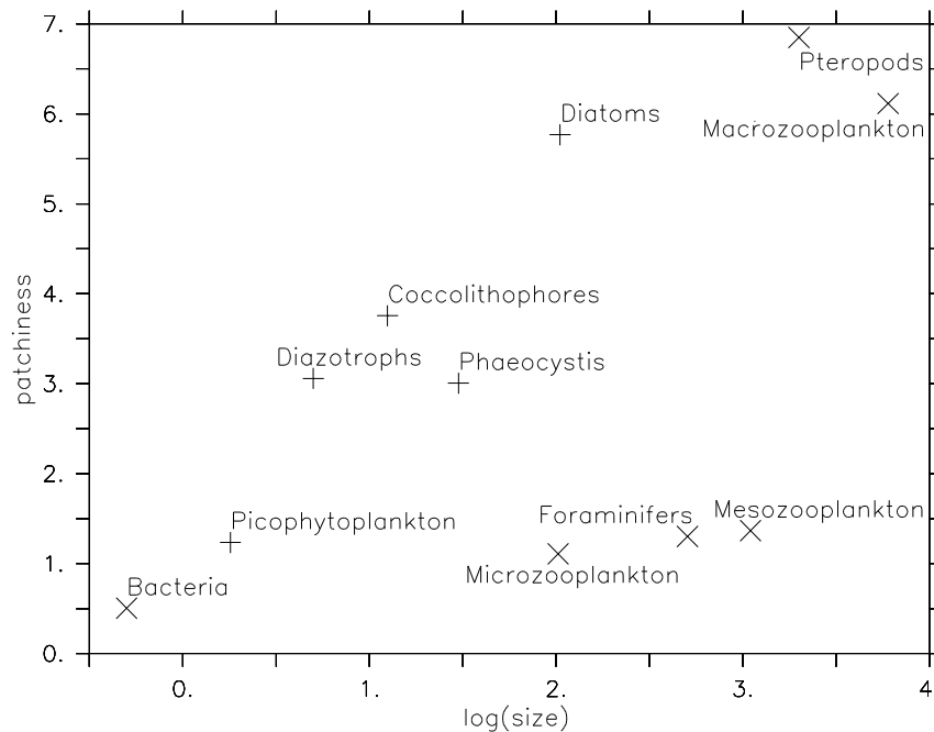
Fig. 4. Patchiness (see Sect. 2.3) as a function of log (nominal organism size in \mu\text{m} ). Pluses: autotrophs, crosses: heterotrophs.
