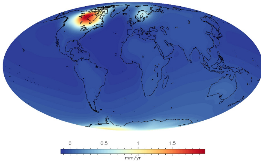
Fig. 10. Geoid change per year due to Glacial Isostatic Adjustment as predicted by the associated 180 \times 180 spherical harmonic expansion.
