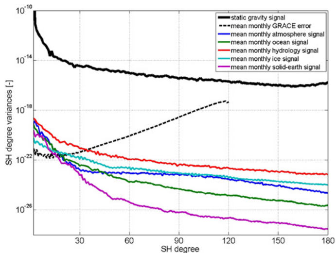
Fig. 12. Mean of monthly signal in terms of spherical harmonic degree variances for different mass variation fields compared to mean monthly error from GRACE time variable gravity field estimates.
