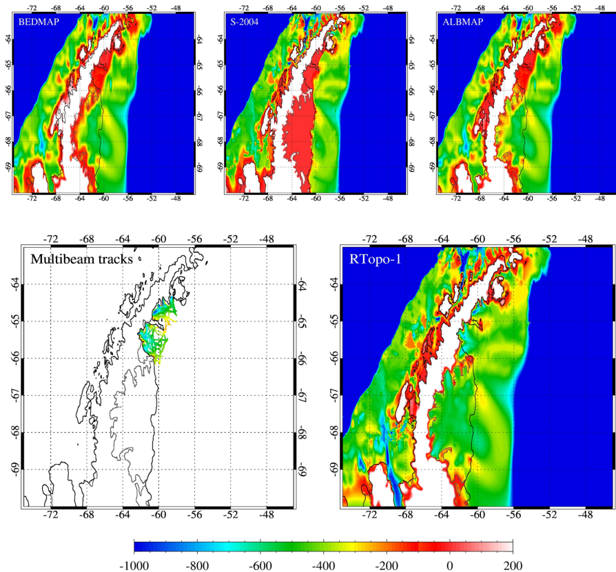
Fig. 5. Different representations of bathymetry (bedrock topography) in the area of the Larsen Ice Shelves. Top row: BEDMAP (left), S-2004 (middle), and ALBMAP (right). Bottom row: Multibeam track data (left), and the RTopo-1 product (right). Ice shelf front and coastline are marked with a black line, grounding line location with a grey line.
