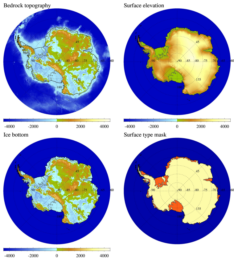
Fig. 2. Antarctic subset of the RTopo-1 dataset. Top left: Bedrock topography (ocean bathymetry). Top right: surface elevation. Bottom left: ice bottom surface height (including ice shelf draft). Bottom right: surface type mask, blue = ocean, yellow = grounded ice, orange = floating ice, grey = bare bedrock (appears only on islands not attached to the Antarctic Ice Sheet here). Grey line marks the grounding line, black line the ice shelf front or coast.
