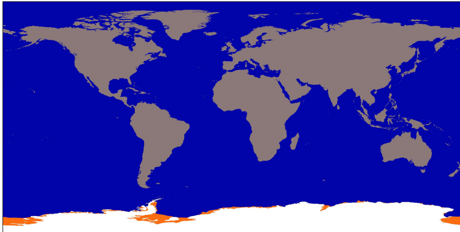
Fig. 7. Global surface type mask in RTopo-1. Blue = ocean, white = grounded ice, orange = ice shelf, grey = bare land surface.
