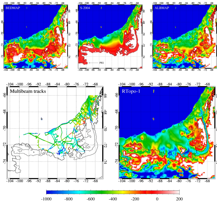
Fig. 6. Different representations of bathymetry (bedrock topography) in the Bellingshausen Sea. Top row: BEDMAP (left), S-2004 (middle), and ALBMAP (right). Bottom row: Multibeam track data (left), and the RTopo-1 product (right). Note the differences for Pine Island Glacier (PIG) and George VI sub-ice bathymetries. Black line represents the coastline or ice shelf front, dark grey line the grounding line.
