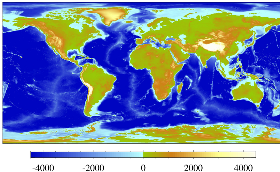
Fig. 1. RTopo-1 global bedrock topography. On continents outside Antarctica, this represents the topography of the solid surface (e.g. bottom of lakes, surface elevation of glaciers and continental ice caps) and mirrors the S-2004 dataset.
