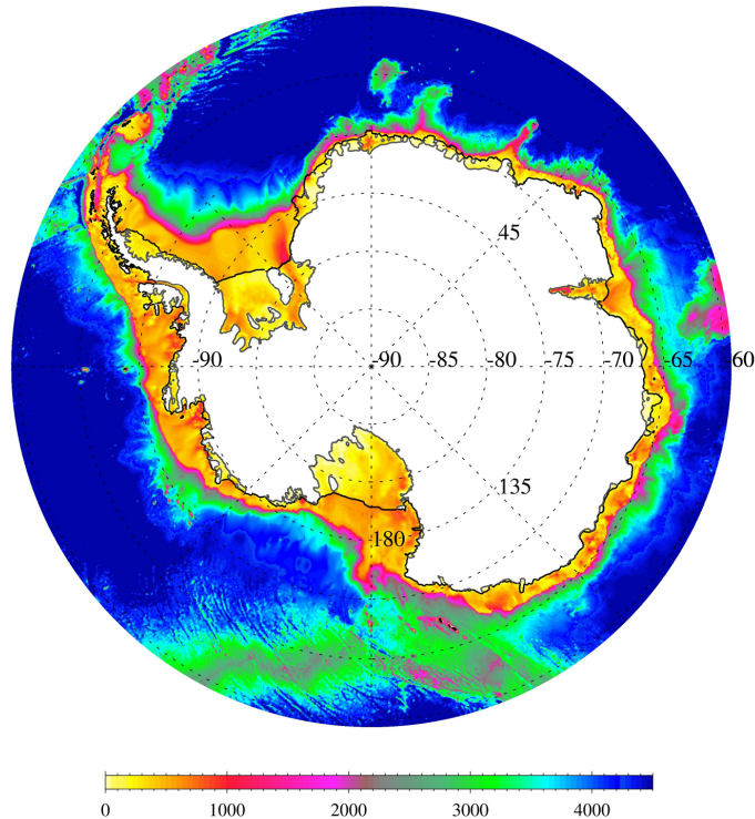
Fig. 8. Water column thickness in the Southern Ocean sector of RTopo-1.
