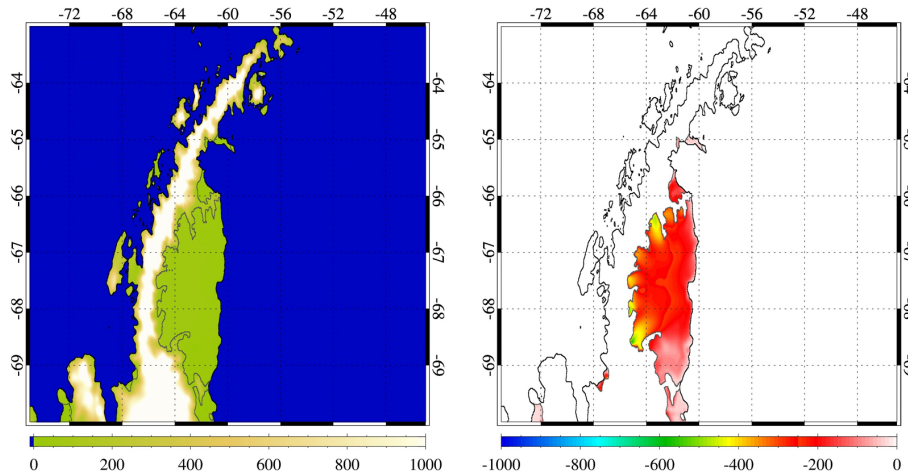
Fig. 4. Surface elevation (left) and ice shelf draft (right) for the Antarctic Peninsula, including Larsen C ice shelf and the remnants of Larsen B ice shelf. The ice shelf front is marked with a black line, the grounding line location with a grey line.
