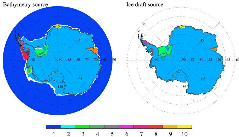
Fig. 3. Data sources for ocean bathymetry (left) and ice sheet/shelf topography (right). See Table 1 for an explanation of numbers. White areas mark transition zones between the datasets.
