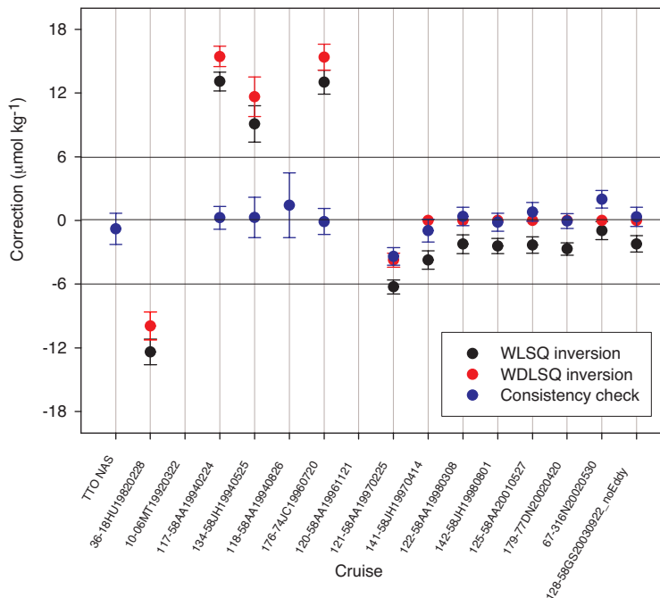
Fig. 2. Corrections from the WLSQ and WDSLQ inversion of manual crossover offsets, as well as corrections determined through a cnaX analysis of the data with recommendations implemented. 58GS20030922 (128) had several stations in a submesoscale coherent eddy (Kasajima et al., 2006), the “_noEddy” signifies that these data were removed prior to this analysis. Note that the cruises have been sorted by time in this figure. The crossover results that were used in the inversions to prepare this figure can be accessed at the CARINA website ( http://cdiac.ornl.gov/oceans/CARINA/Carina_inv.html ).
