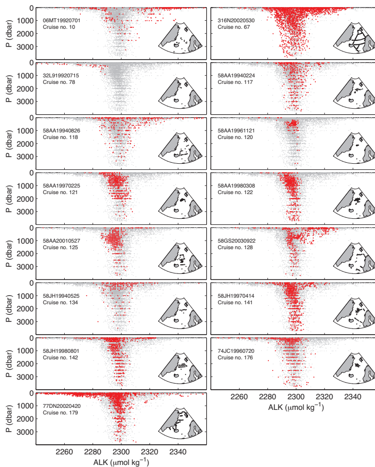
Fig. 4. Station positions and ALK data of Nordic Seas CARINA cruises after secondary QC. All data shown in grey and specific cruise in red.
