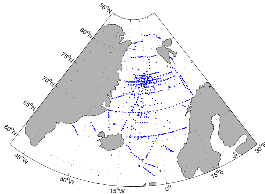
Fig. 1. The Nordic Seas with ALK sampling positions, includes only data retained through analyses described here.
