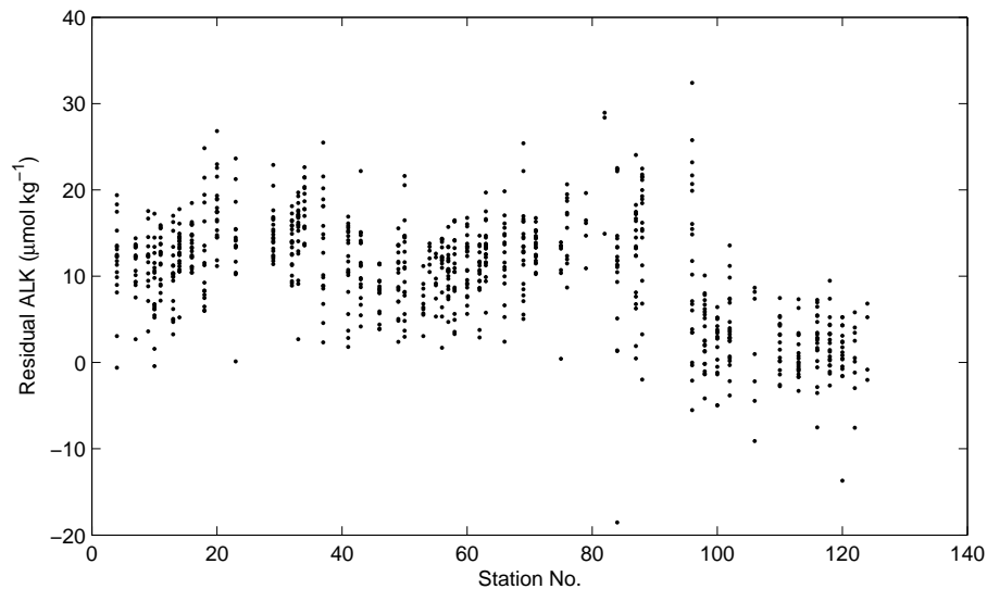
Fig. 3. Difference between measured and calculated (from Eq. 1) 18HU19820228 (36) ALK values vs. station number (measured – estimated).
