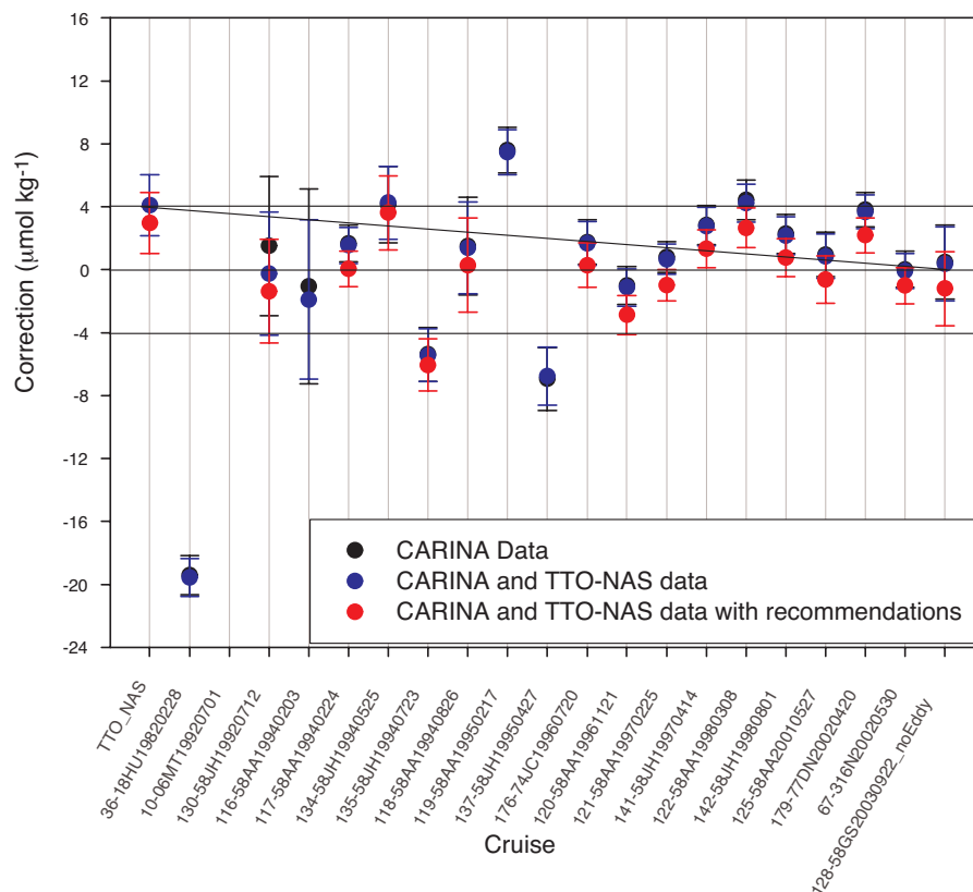
Fig. 2. Corrections from WLSQ inversion of crossover offsets for (1) the CARINA data, (2) The CARINA and TTO-NAS data, and (3) the CARINA and TTO-NAS data after completed secondary QC. The straight line has been drawn to emphasise the change between TTO-NAS and 58GS20030922. “no_Eddy” signifies that the stations in the submesoscale coherent eddy encountered at this cruise (Kasajima et al., 2006) were excluded from the analyses.
