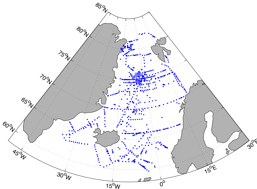
Fig. 1. Nordic Seas with \text{TCO}_2 sampling positions, includes only data retained after secondary quality control.
