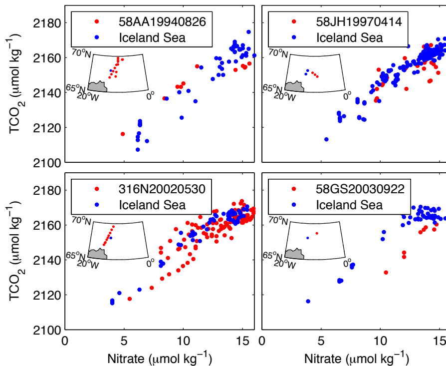
Fig. 5. Iceland Sea TCO 2 vs. nitrate, along with data from 4 cruises which had stations in the vicinity.
