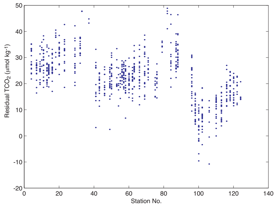
Fig. 3. Difference between measured 18HU19820228 TCO 2 data and those determined using MLR (Eq. 1), measured – estimated.
