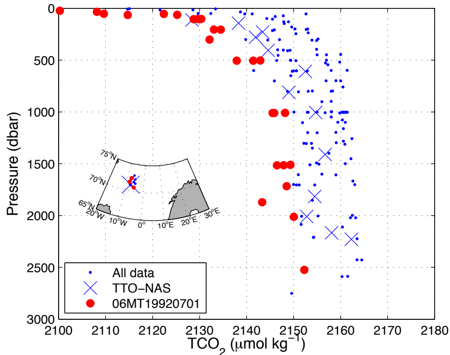
Fig. 4. TCO 2 data obtained to the north of Jan Mayen at the 06MT19920701 cruise, along with data from the TTO-NAS cruise as well as from the other, more recent, cruises with TCO 2 data in CARINA.
