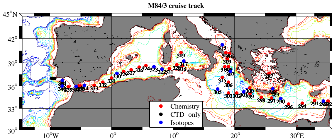
Figure 1. Cruise track of M84/3 with CTD stations marked in different colors based on the extent of measurements carried out.
