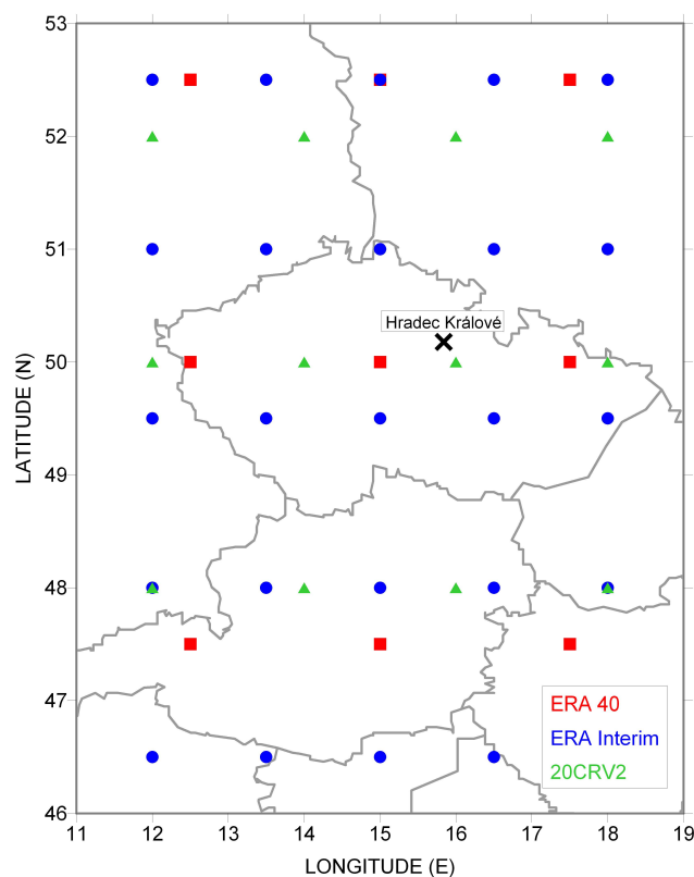
Figure 2. The grid points of 20th Century Reanalysis V2, ERA-40 and ERA-Interim re-analyses surrounding the location of Hradec Králové.
