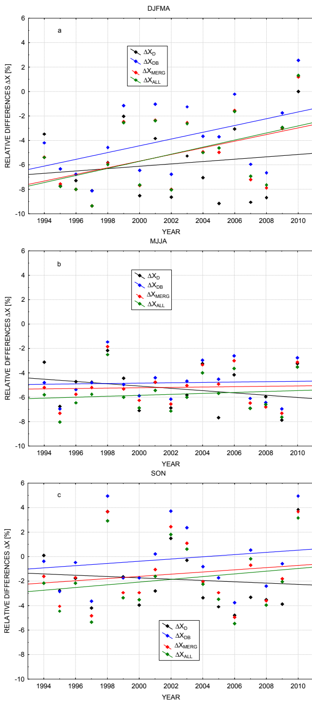
Figure 7. Linear approximations of the relative differences \Delta X_D , \Delta X_{DB} , \Delta X_{MERG} , \Delta X_{ALL} in the Post-Pinatubo period in particular seasons DJFMA (a), MJJA (b) and SON (c), Hradec Králové, 1994–2010.
