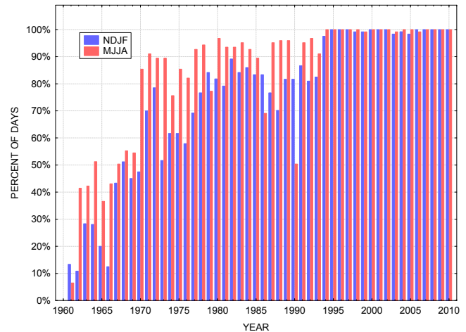
Figure 5. Average numbers of days with total ozone observations per month in the merged data series X_{MERG} in the winter (NDJF) a summer (MJJA) seasons, Hradec Králové, 1961–2010.
