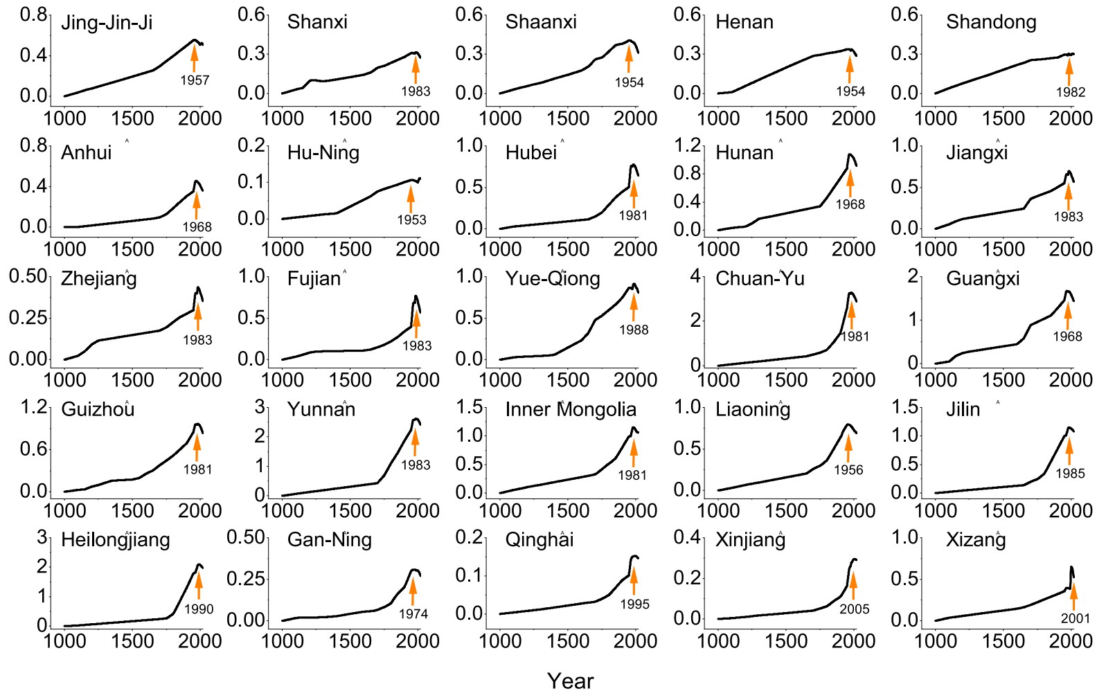
Carbon emission (Pg)
