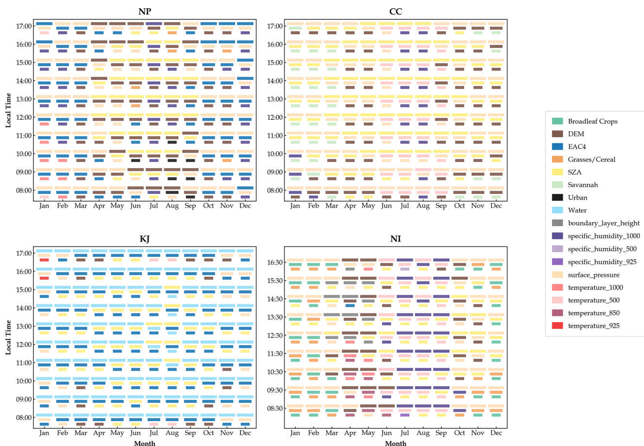
Figure 12. Monthly and hourly feature importance rankings for the four regions based on the zero-out perturbation method.
