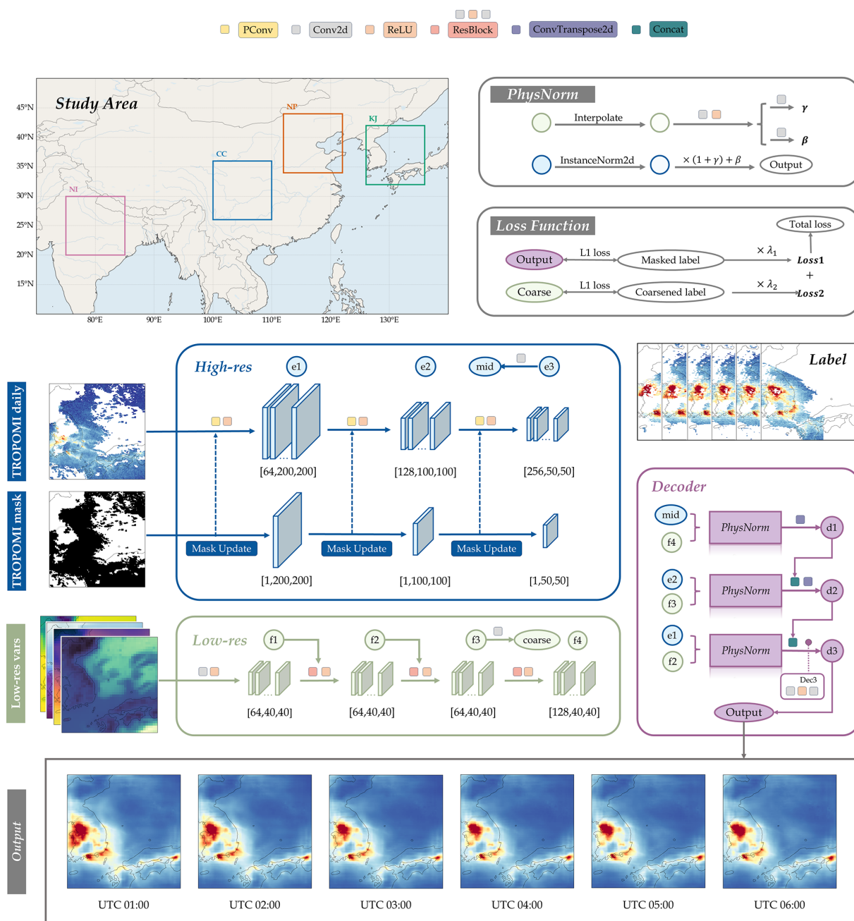
Figure 1. Architecture diagram of PhysNorm-Net.
