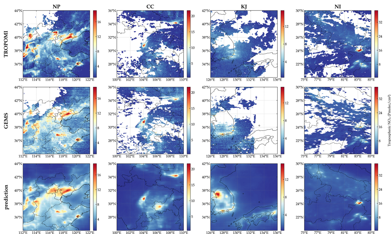
Figure 3. Comparison of single-day spatial distributions of NO 2 concentration from TROPOMI, GEMS, and model predictions on 26 April 2023.
