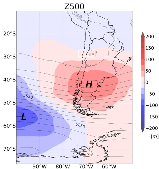
Figure 8. Composites of geopotential height at 500 hPa (contours) and its anomalies (colors) for the category Convergence on austral summer (DJF). The black rectangle frames the area related to the LB3 between 27–30° S. Cyclonic (“L”) and anticyclonic (“H”) circulation anomalies are highlighted.
