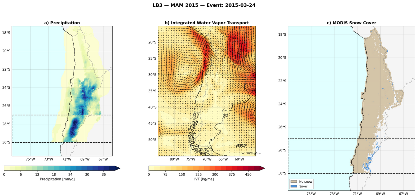
Figure A1. Example reading of the catalog for the LB3 MAM 2015 extreme precipitation event (24 March 2015). (a) Daily precipitation (mm d −1 ) from CR2METv2.5 over the study area (17.25–31.5° S, 77–66° W). (b) Vertically integrated water vapor transport magnitude (kg ms −1 ; shading) and direction (vectors; reference arrow: 100 kg ms −1 ) derived from ERA5, shown over a broader South American domain (15–55° S, 85–55° W). (c) MODIS-derived snow cover classification for the event date, distinguishing snow-covered (blue) and snow-free (beige) pixels. Dashed rectangles indicate the LB3 latitudinal band (27–30° S).
