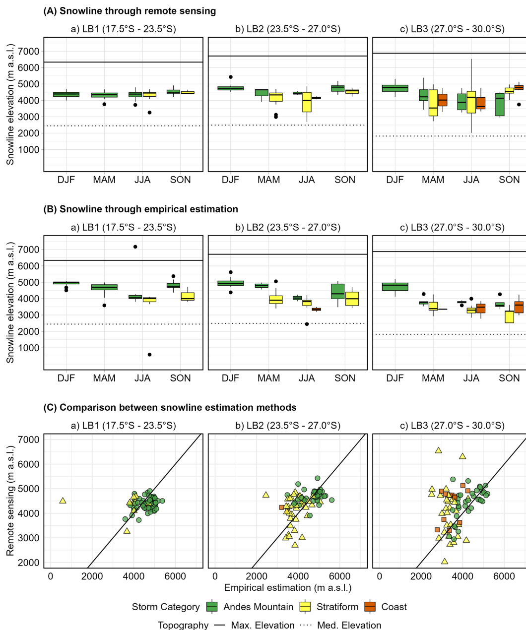
Figure 6. (A) Snowline elevation detected through MODIS imagery, (B) estimated empirically in each latitudinal band, and (C) estimation scatter plot, categorized by storm during 2000–2019. The Maximum (solid line) and median (dotted line) elevations by band are also included to illustrate the snow-covered area.
