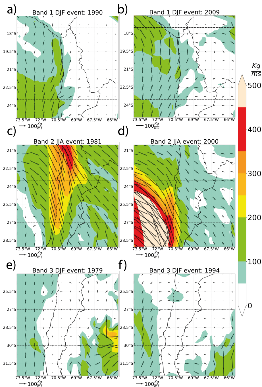
Figure 4. Examples of vertically Integrated Water Vapor Transport ( \text{kg ms}^{-1} ) patterns for the representative examples of extreme precipitation events selected in the catalog. The black rectangle encloses the latitudinal band area related to the event. The uppermost panels show DJF LB1 results, the middle section corresponds to JJA LB2, and the lowermost panels are for DJF LB3 precipitation patterns.
