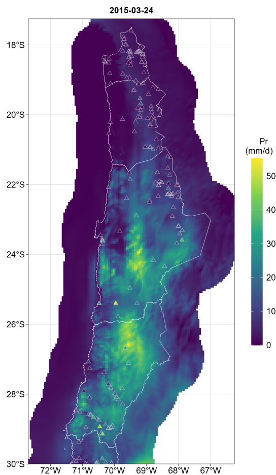
Figure A2. Daily precipitation during 24 March 2015 according to CR2METv2.5 (raster) and weather stations (triangles).
