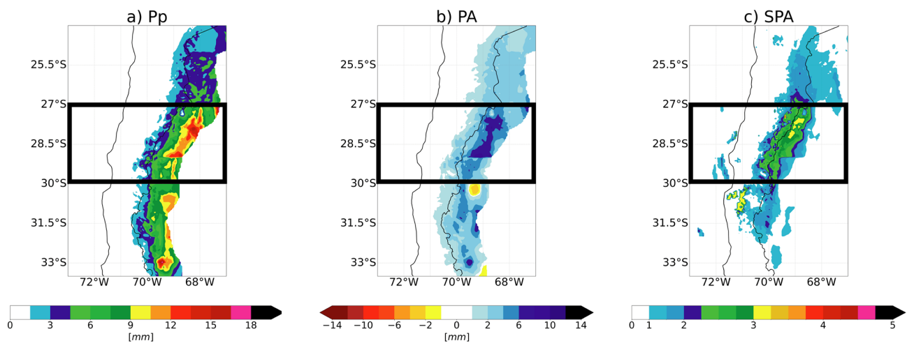
Figure 7. Composites for the LB3 Convergence category in austral summer (DJF) of: (a) daily precipitation data (Pp); (b) precipitation anomalies (PA; from daily climatology); and (c) standardized precipitation anomalies (SPA; from daily climatology and daily standard deviation). The black rectangles frame the area related to the LB3 between 27–30° S.
