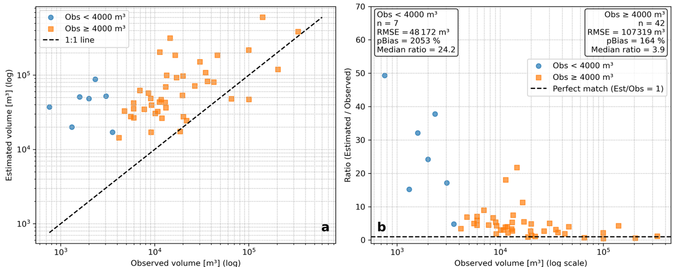
Figure 10. (a) Coarse estimation of debris flow volume based on transport capacity for the March 2015 event. Comparison with measured deposited volumes at 49 alluvial fans located in the Huasco River Basin. (b) Ratio of estimated vs. observed to quantify the prediction correlation degree.
