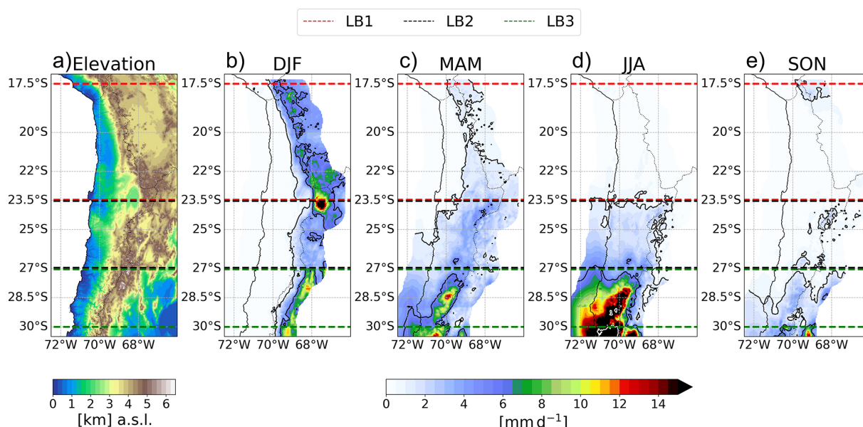
Figure 1. Climate and elevation features in northern Chile. (a) Topography (km a.s.l.); Panels (b) through (e) show the composite of maximum precipitation events ( \text{mm d}^{-1} ) for each season (1979–2019, 41 events per season). Dashed lines delimit the three latitudinal bands (LB1, LB2, LB3). Black contours indicate the 1 and 5 \text{mm d}^{-1} thresholds; white contours indicate 20 \text{mm d}^{-1} .
