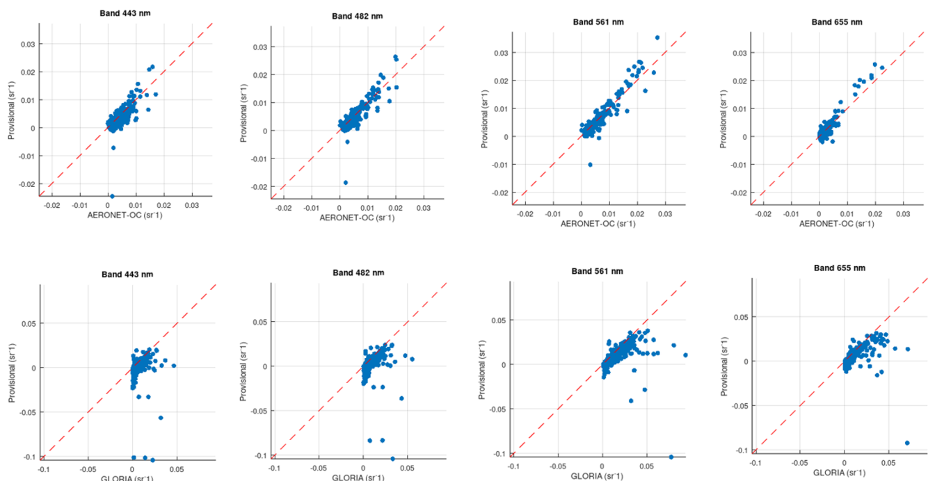
Figure 7. Per band scatter plots between Landsat 8/9 provisional AR with AERONET-OC (top) and GLORIA (bottom) in situ R_{\text{rs}} matchups. 1 : 1 line shown in red.
