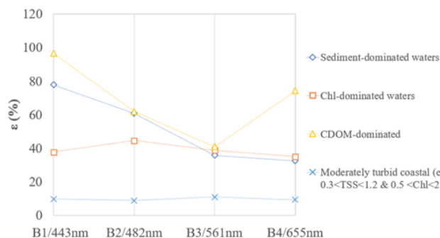
Figure 8. Isolated median symmetric accuracy ( \varepsilon ) between GLORIA in situ R_{\text{rs}} and Landsat 8/9 Level 2 provisional AR by reported water type.
