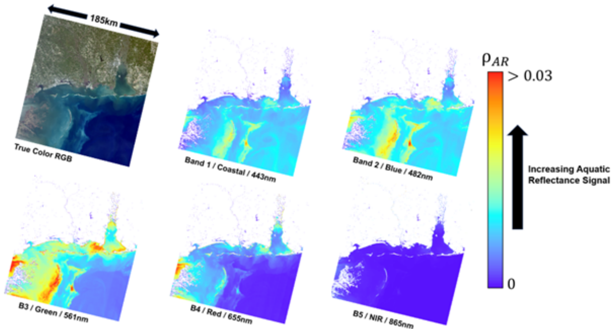
Figure 1. Example of the Landsat 8/9 Level 2 provisional Aquatic Reflectance product over coastal Alabama on 15 November 2021. The Landsat 8/9 Level 2 provisional AR product package includes AR for the five OLI visible and near infrared (VNIR) bands centered at 443 nm (coastal/aerosol), 482 nm (blue), 561 nm (green), 655 nm (red), and 865 nm (NIR) for identified water pixels at 30 m spatial resolution. Landsat image courtesy of the U.S. Geological Survey.
