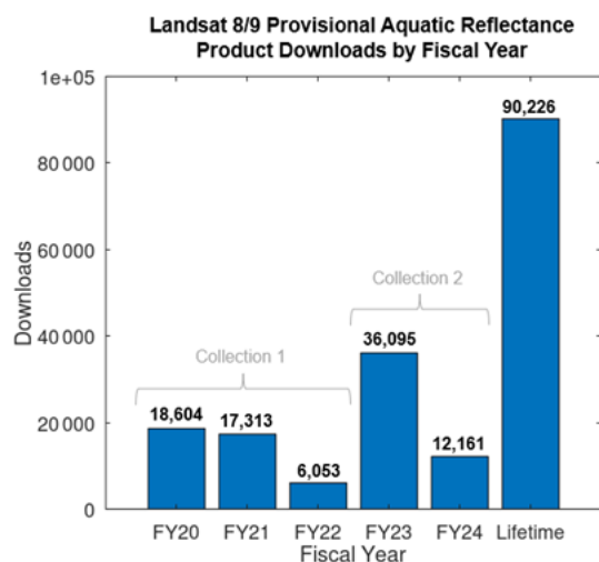
Figure 2. Annual download metrics of the Landsat 8/9 provisional AR science products. While not formally part of a Collection themselves, the AR products have been released using either Collection 1 or Collection 2 input data.
