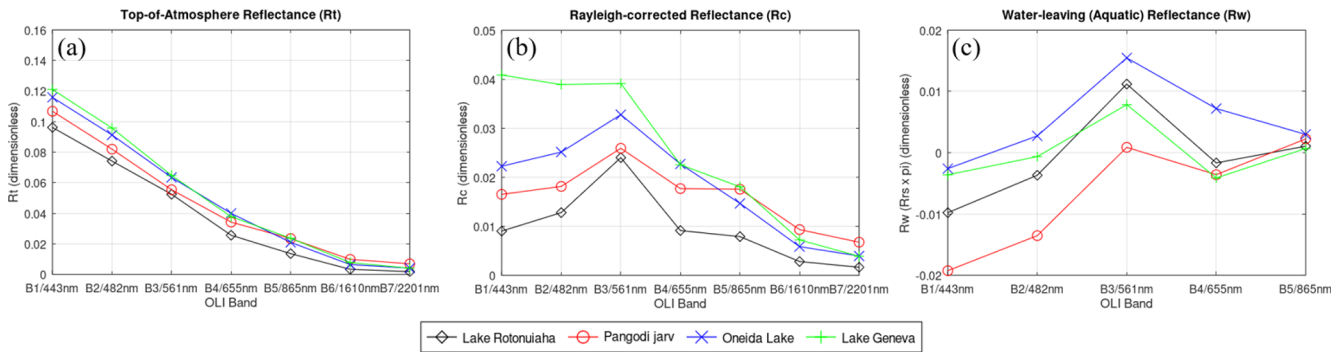
Figure 3. Examples of Landsat 8 top-of-atmosphere (TOA) reflectance (a), Rayleigh-corrected reflectance (b), and Landsat 8 provisional aquatic reflectance ( AR = R_{rs} \cdot \pi ) (c) for a collection of freshwater bodies, including Lake Rotonuiaha, New Zealand on 11 December 2017 (LC08_L1TP_072087_20171211_20200902_02_T1), Pangodi järv, Estonia on 26 May 2018 (LC08_L1TP_187019_20180526_20200901_02_T1), Oneida Lake, New York, USA on 30 August 2014 (LC08_L1TP_015030_20140830_20200911_02_T1), and Lake Geneva, Switzerland on 12 April 2020 (LC08_L1TP_196027_20200412_20200822_02_T1). Atmospheric interference impacts the spectral profile retrieved by the sensor in low Earth orbit, obscuring key reflectance and absorption features of the optically active constituents in surface waters (a). The Rayleigh correction mitigates the molecular scattering contribution from atmospheric gases, allowing for the retrieval of representative spectral profiles of diverse water targets (b). However, overcorrection of aerosols can lead to negative provisional AR spectra in the VIS bands (c).
