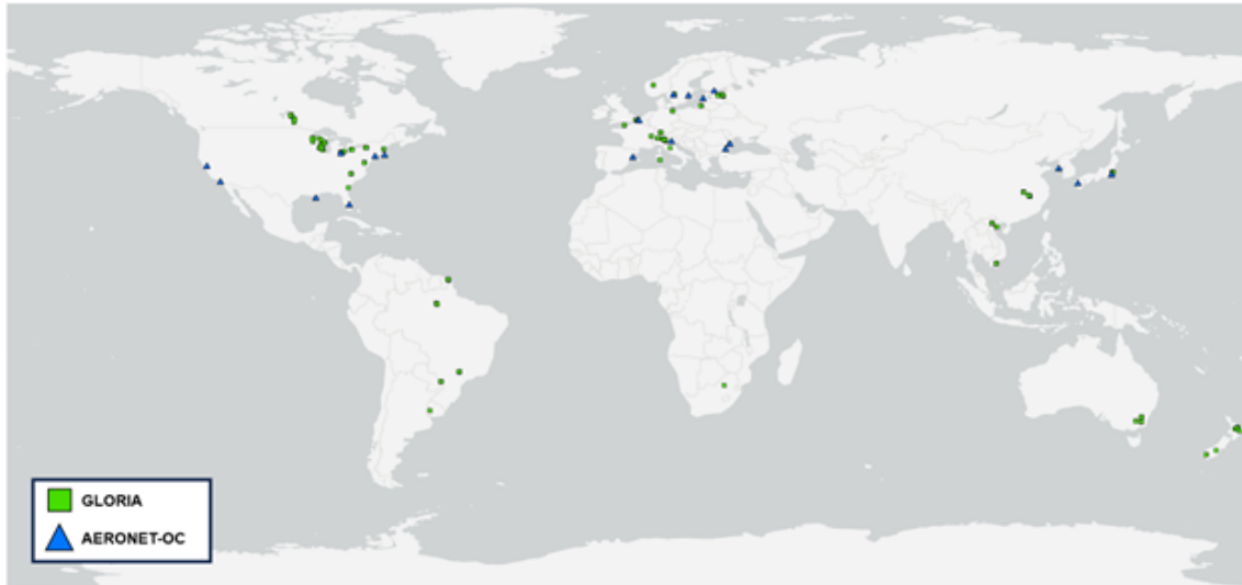
Figure 4. Global distribution of the combined AERONET-OC ( n_{\text{aeronet}} = 418 ) and GLORIA ( n_{\text{gloria}} = 554 ) matchups with Landsat 8/9 acquisitions.
