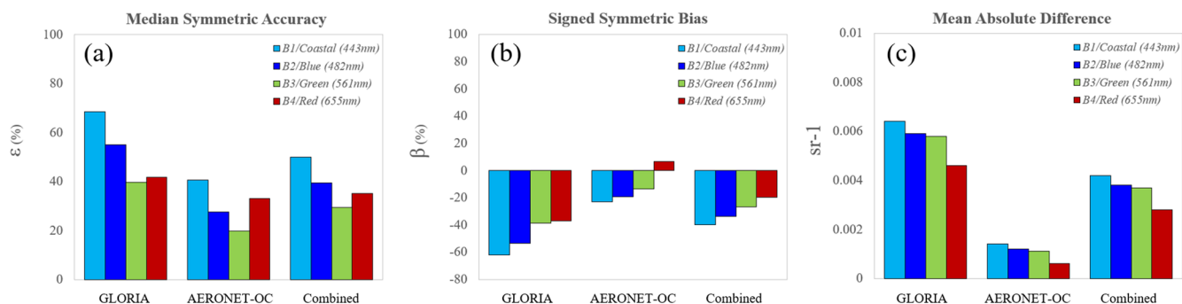
Figure 6. Performance metrics used to evaluate the accuracy of Landsat 8/9 provisional AR products between AERONET ( n_{\text{aeronet}} = 418 ), GLORIA ( n_{\text{gloria}} = 554 ), and the combined ( n_{\text{combined}} = 972 ) R_{\text{rs}} matchup datasets.
