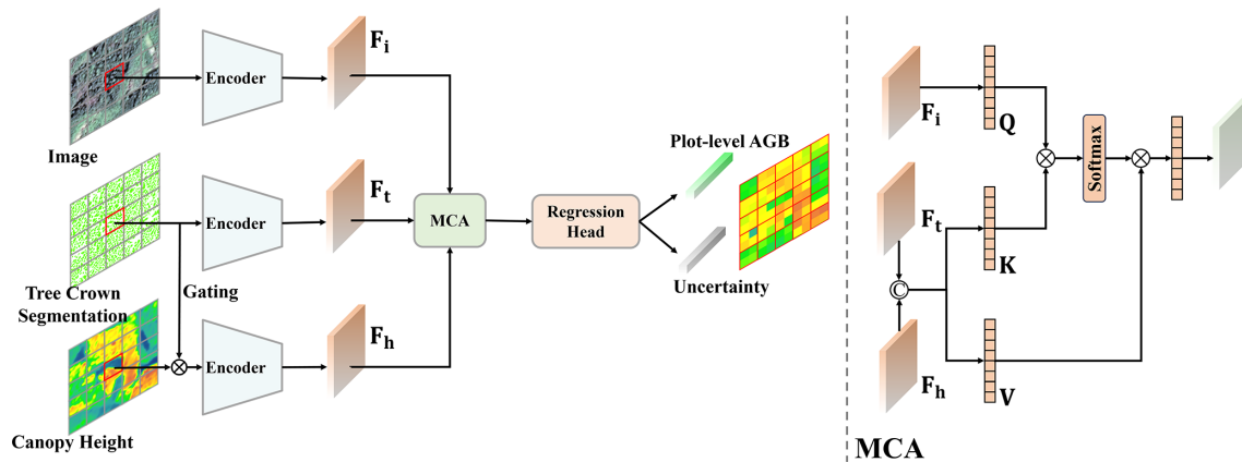
Figure 3. Architecture of the Canopy Structure-driven Multi-feature Fusion Network (CSMF-Net) and the Multi-feature Cross-Attention Module.
