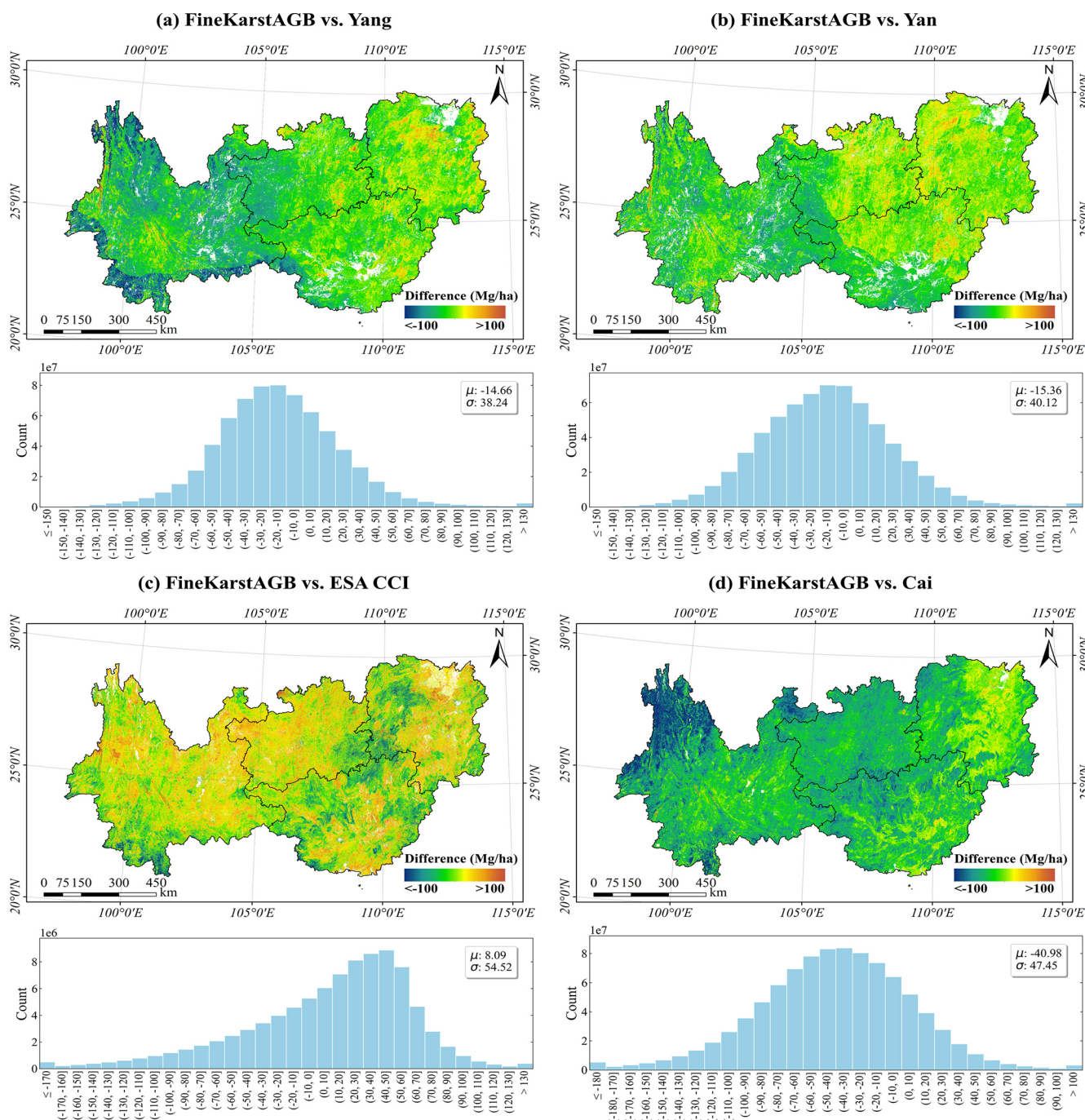
Figure 12. Spatial distribution and statistics of AGB differences between FineKarstAGB and the comparison datasets: (a) Yang et al. (2023), (b) Yan et al. (2023a), (c) ESA CCI, and (d) Cai et al. (2024b). Pairwise differences were calculated after spatial alignment using only pixels with valid estimates in both products. FineKarstAGB was aggregated to the native 100 m grid for comparison with ESA CCI. \mu and \sigma denote the mean and standard deviation of the AGB differences, respectively.
