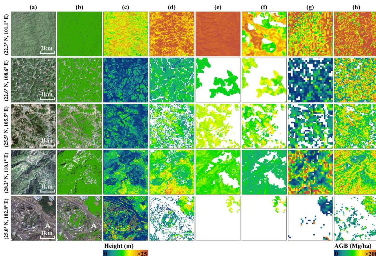
Figure 11. Comparison of different AGB datasets across typical landscapes. (a) GaoFen imagery, (b) Tree Cover, (c) Canopy Height, (d) FineKarstAGB (Ours), (e) AGB from Yang et al. (2023), (f) AGB from Yan et al. (2023a), (g) AGB from ESA CCI and (h) AGB from Cai et al. (2024b).
