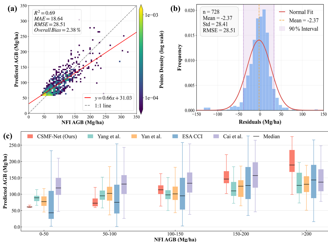
Figure 4. Evaluation of the CSMF-Net against independent NFI plots ( n = 728 ). (a) Scatter plot of predicted versus observed AGB for independent NFI test plots. (b) Distribution of residuals (predicted AGB minus observed AGB) for the NFI test plots. (c) Binned analysis of the AGB estimated by CSMF-Net (Ours) with the existing datasets.
