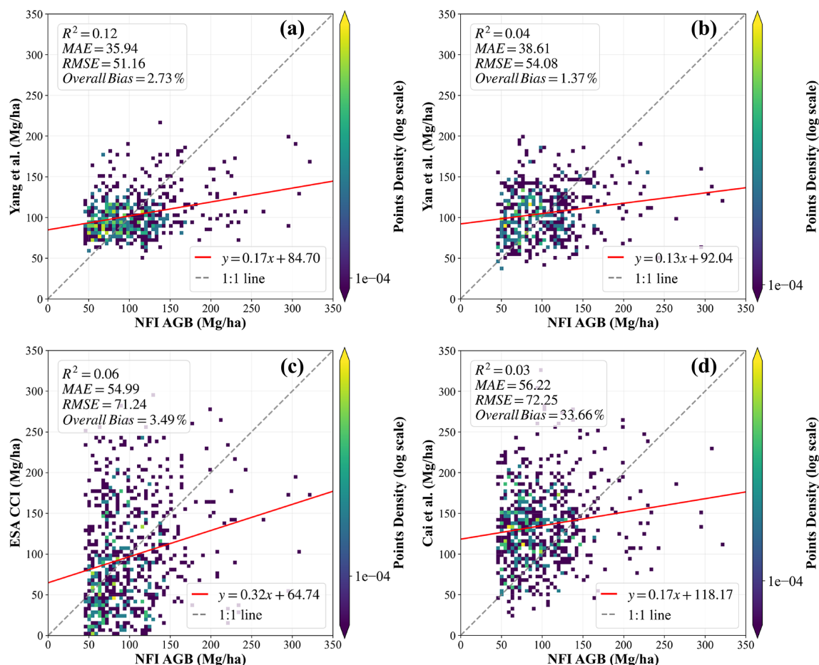
Figure 5. Comparison of the existing datasets with NFI data. (a) Yang et al. (2023), (b) Yan et al. (2023a), (c) ESA CCI and (d) Cai et al. (2024b).
