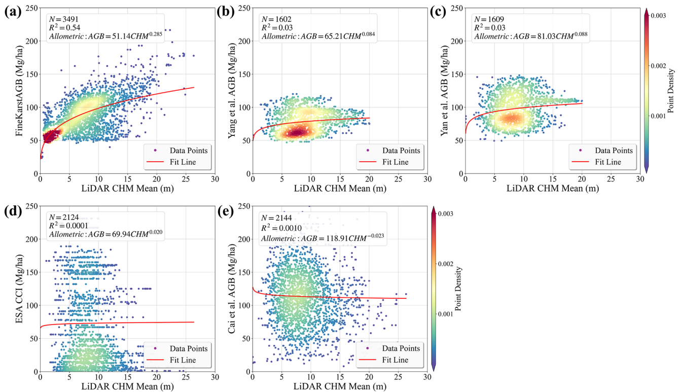
Figure 7. Structural-consistency assessment of the AGB datasets against mean UAV LiDAR-derived canopy height using forest validation samples. Results are shown for (a) FineKarstAGB, (b) Yang et al. (2023), (c) Yan et al. (2023a), (d) ESA CCI, and (e) Cai et al. (2024b). Sample sizes in panels (b)–(e) vary because only locations with valid values in the corresponding products were included.
