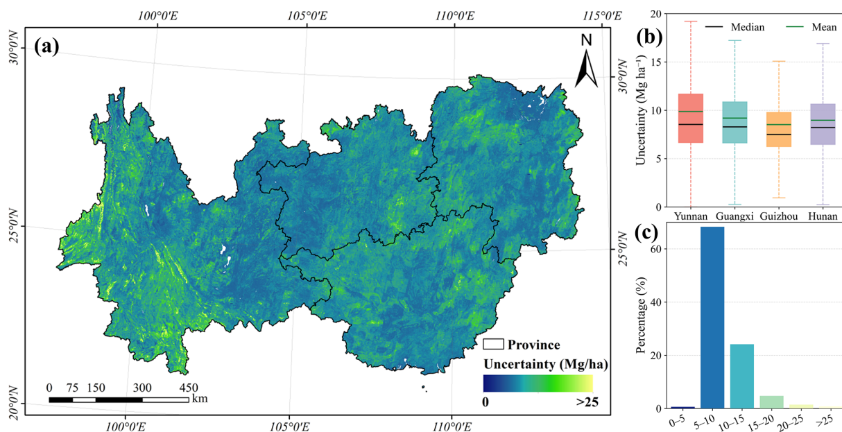
Figure 10. Spatial distribution and statistical characteristics of the predictive uncertainty of FineKarstAGB. (a) Spatial distribution of AGB uncertainty, (b) provincial uncertainty statistics, and (c) frequency distribution of uncertainty.
