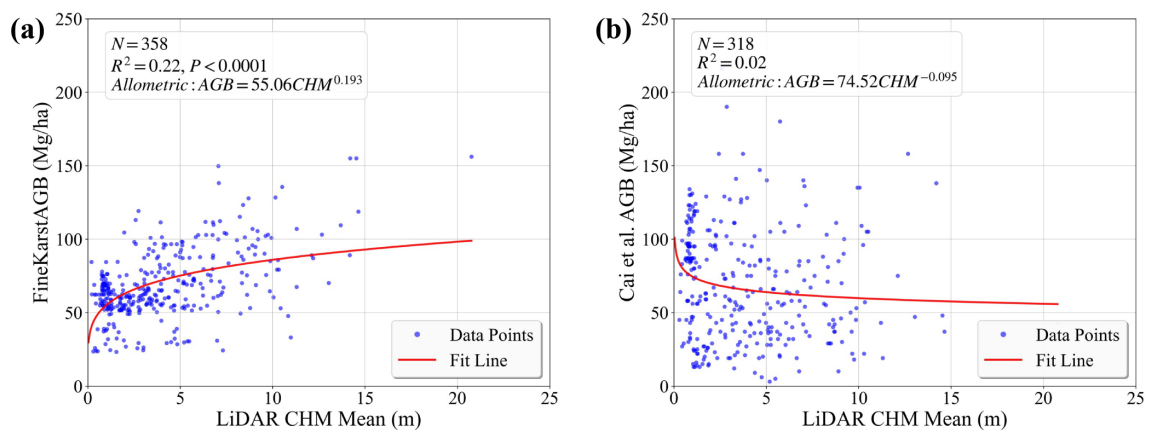
Figure 8. Evaluation of our dataset against LiDAR CHM data in non-forest areas. (a) results of FineKarstAGB (Ours), (b) results from Cai et al. (2024b).
